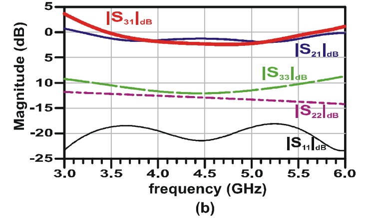
Fig.5-a. Simulated phases in degrees of S_{21} , S_{31} and their difference, and -b simulated return S_{11}(\text{dB}) , S_{22}(\text{dB}) and S_{33}(\text{dB}) , and insertion losses S_{21}(\text{dB}) and S_{31}(\text{dB}) .
