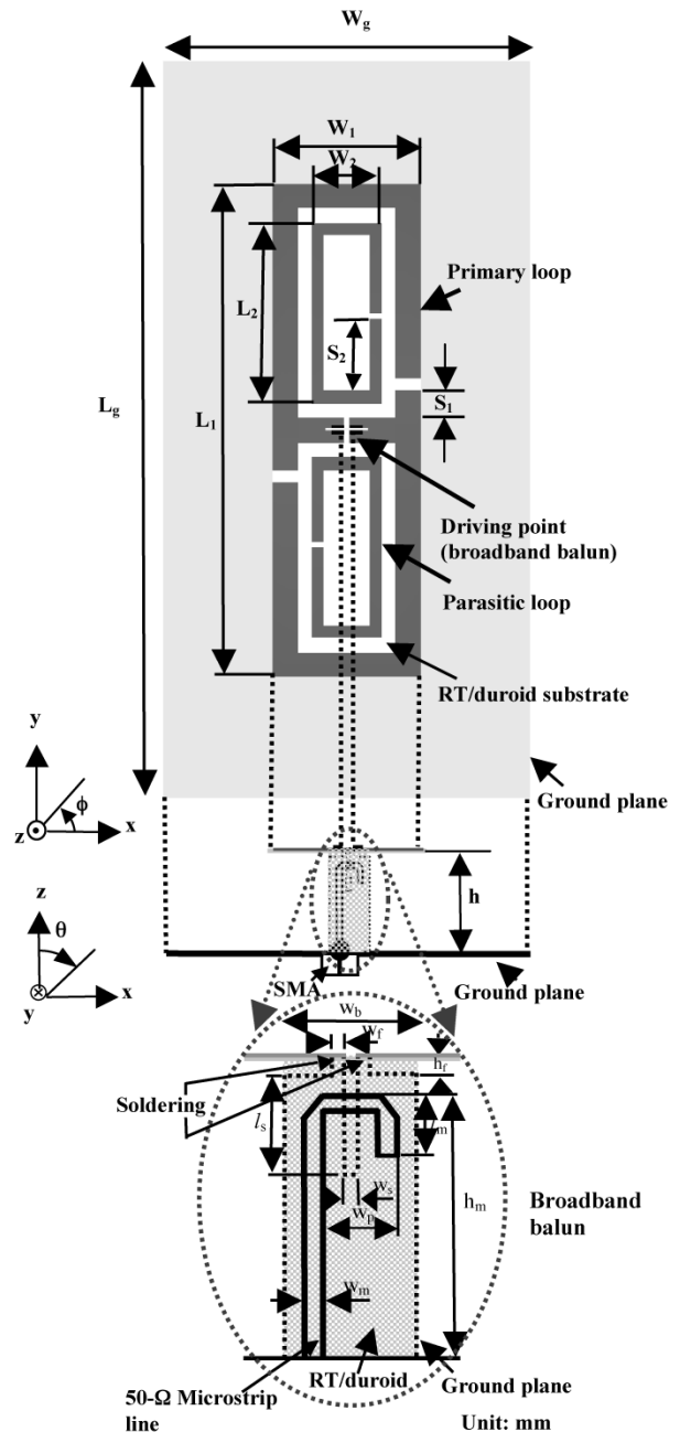
Fig. 1. Broadband circularly polarized rectangular loop antenna with impedance matching. (The strip widths of the primary loop and of the parasitic loops are 2.0 mm and 1.0 mm, respectively; the gap widths on the primary loop and on the parasitic loops are 1.0 and 0.5 mm, respectively; L_g = 60 mm, W_g = 30 mm, W_b = 6.0 mm, W_f = 0.6 mm, W_s = 0.5 mm, W_m = 0.8 mm, W_p = 3.2 mm, h_f = 1.0 mm, h_m = 13 mm, l_s = 5 mm, l_m = 3 mm.)
