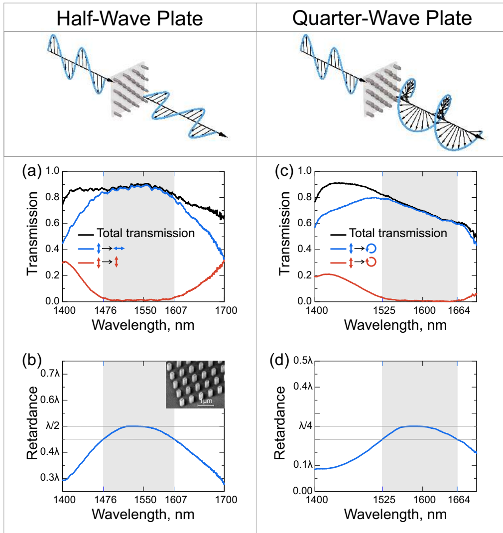
FIG. 4. Demonstration of half- and quarter-wave plates. (a) Experimental transmission spectra of the half-wave plate. Black line – total transmission . Red line – transmission through a metasurface positioned between a pair of linear parallel polarizer and analyzer with polarization axis oriented at 45^\circ to metasurface’s anisotropy axis. Blue line – transmission through a metasurface positioned between a pair of linear crossed polarizer and analyzer with polarization axis oriented at \pm 45^\circ to metasurface’s anisotropy axis. (b) Experimentally retrieved retardance of the half-wave plate. Highlighted region shows the spectral range, with a deviation from \lambda/2 by no more than 10%, or \lambda/20 . Inset shows a scanning electron micrograph of the fabricated half-wave plate. (c) Experimental transmission spectra of the quarter-wave plate. Black line – total transmission . Red line – transmission through a metasurface positioned between a pair of linear polarizer with polarization axis oriented at 45^\circ to metasurface’s anisotropy axis and a right-circular analyzer. Blue line – transmission through a pair of linear polarizer with polarization axis oriented at 45^\circ to metasurface’s anisotropy axis and a left-circular analyzer. (d) Experimentally retrieved retardance of the quarter-wave plate. Highlighted region show the spectral range, with retardance deviation from \lambda/4 by no more than \lambda/20 .
