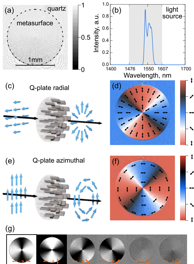
FIG. 5. Demonstration of highly-efficient q -plates. (a) Transmission image of the q -plate 1.5 mm in diameter placed on top of a quartz wafer, taken with an amplified spontaneous emission (ASE) broadband light source at around 1550 nm wavelengths. Note that the device appear to be nearly transparent. (b) Spectrum of the ASE light source used for the experiment. (c) q -plate functionality concept: conversion of vertical into azimuthal polarization. (d) Experimentally measured spatially-resolved polarization of the azimuthally polarized output beam. (e) The q -plate functionality concept: conversion of horizontal into radial polarization. (f) Experimentally measured spatially-resolved polarization of the radially polarized output beam. (g) Examples of light transmission through the q -plate positioned between different polarizers and analyzers (polarizer axes orientations marked in insets).
