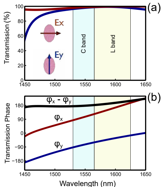
FIG. 3. (a) Transmission spectrum of the metasurface shown in Fig. 2, for polarizations parallel to the two axes of the nanopillar. (b) Phase of the transmitted waves with respect to the incident field for both orthogonal polarizations. The phase difference \varphi_x - \varphi_y shows a constant value of \pi over a broad spectral range, as required for a broadband half-wave plate.
