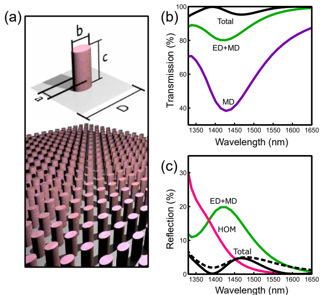
FIG. 2. (a) Schematic of our broadband metasurface. The spectra in (b) and (c) show the transmission and reflection of the metasurface and their dependence on the multipoles (ED = electric dipole, MD = magnetic dipole, and HOM = sum of higher-order multipoles). The black dashed curve in (c) shows the complete multipolar reflection when excluding reflection off the glass substrate. Dimensions are a = 285 nm, b = 450 nm, c = 860 nm and D = 750 nm, and the incident polarization is parallel to the short axis of the nanopillars.
