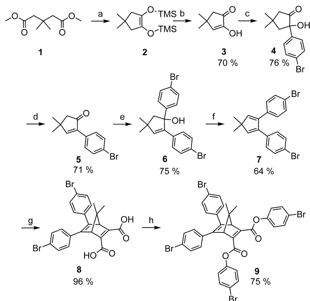
Scheme 1 (a). Na/K alloy, TMSCl, benzene; (b) Br 2 ; (c) n -BuLi, p -dibromobenzene, -78^{\circ}\text{C} ; (d) p -TsOH, Toluene, reflux; (e) n -BuLi, p -dibromobenzene, -78^{\circ}\text{C} ; (f) p -TsOH, toluene, reflux; (g) Butynedioic acid, toluene, reflux; (h) 1. Oxalylchloride, DMF, Et 3 N. 2. DMAP, p -bromophenol.
