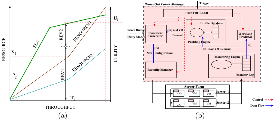
Fig. 1. (a) Utility Computation in BrownMap and (b) BrownMap Architecture
