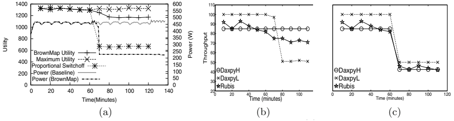
Fig. 8. Consolidating 2 blades with a power budget of 250W: (a) Comparative Power Consumption and Utility Earned. The Power drawn by Proportional SwitchOff is omitted as it closely follows BrownMap. (b) Normalized Throughput achieved by BrownMap (c) Normalized Throughput achieved by Proportional SwitchOff.
