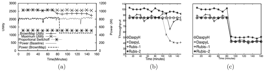
Fig. 9. Consolidating 4 blades with a power budget of 500W: (a) Comparative Power Consumption and Utility Earned. The Power drawn by Proportional SwitchOff is omitted as it closely follows BrownMap. (b) Normalized Throughput achieved by BrownMap (c) Normalized Throughput achieved by Proportional SwitchOff.
