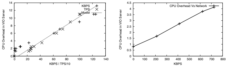
(a) VIO Overhead with LPAR Disk Activity (b) VIO Overhead with LPAR network activity
