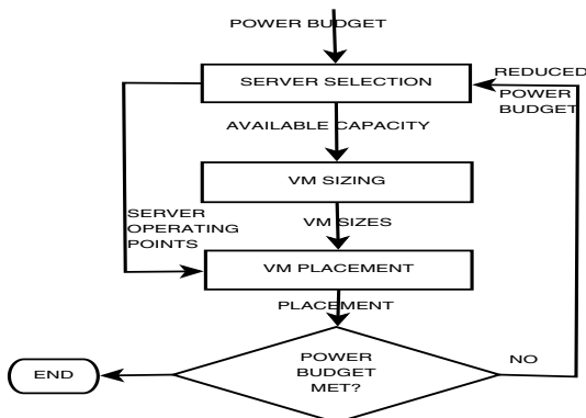
Fig. 3. BrownMap Placement Algorithm Flow
