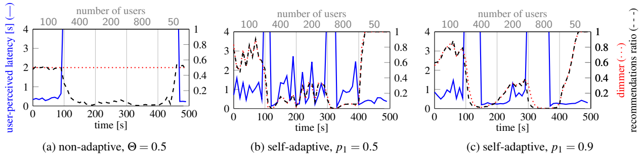
Figure 4: RUBiS behavior in a non-adaptive configuration and two self-adaptive configurations, varying the number of users.
