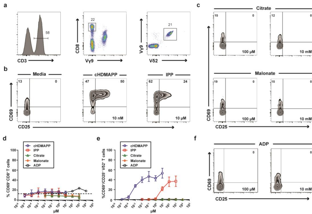
B30.2 domain of human BTN3A1 selectively binds small negatively charged moieties but only a limited set of these molecules directly activates human V \gamma 9/V \delta 2 + T cells.
