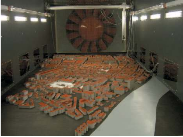
Fig. 23. Wind tunnel model (1:300) of the Kleinbasel area (corresponds approximately to the white area in Fig. 2). View from about 330^\circ . The light surface region in the foreground represents the river Rhine. White material within the scale model corresponds to vegetation
