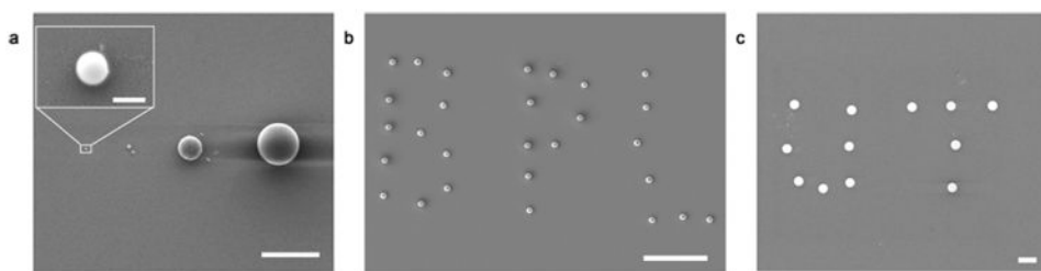
Figure 5. Patterning of PS beads at single-particle resolution. (a) Patterning of single PS beads with different sizes: 540 nm, 0.96 \mu\text{m} , 5.31 \mu\text{m} , and 9.51 \mu\text{m} , respectively (from left to right). (b) SEM image of the “BPL” pattern of 0.96 \mu\text{m} PS beads. (c) SEM image of the “UT” pattern of 5.31 \mu\text{m} PS beads. Scale bar: (a–c) 10 \mu\text{m} ; inset of (a) 500 nm.
