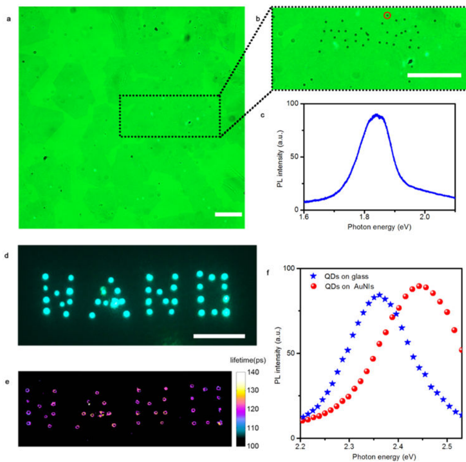
Figure 6. Versatility of BPL in patterning 2D materials and quantum dots. (a) Optical micrograph of the 2D MoS 2 monolayers on the AuNIs substrate. (b) Optical micrograph of the “MoS 2 ” patterns of individual 0.96 μm PS beads written on the 2D MoS 2 monolayer. (c) The PL spectrum of the MoS 2 recorded from the regime with a single PS bead, as indicated by the red circle in (b). (d) Fluorescence image of the “NANO” pattern of 6 nm CdSe/ZnS quantum dots on the AuNIs. (e) Fluorescence lifetime image of the patterned CdSe/ZnS quantum dots as shown in panel d. (f) PL spectra of the quantum dots patterned on the plasmonic substrate and of the quantum dots on the glass substrate. Scale bar: 50 μm.
