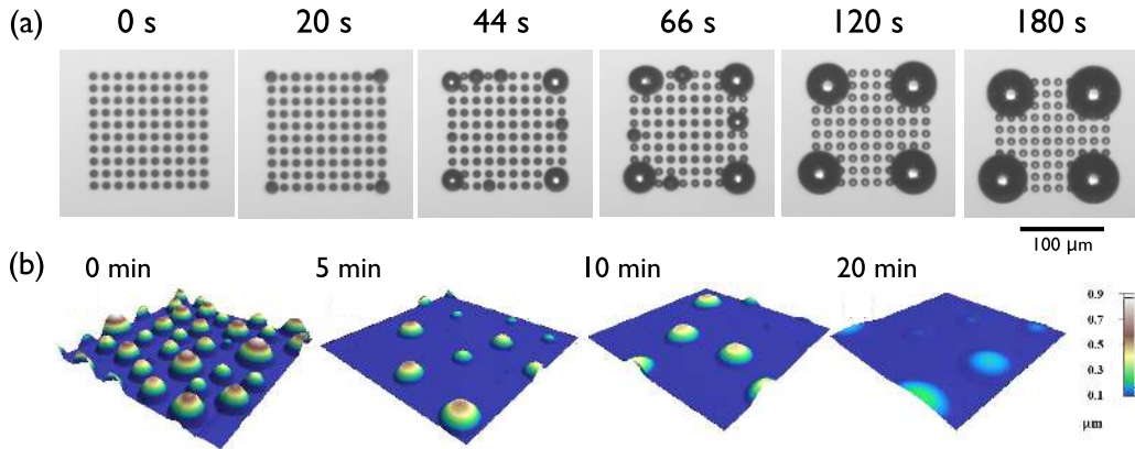
FIG. 21. (a) Controlled microbubble formation and growth on hydrophobic surfaces decorated with micromachined micropits (with a diameter of 10\ \mu\text{m} and edge-to-edge distance of 13\ \mu\text{m} ) by solvent exchange. The microchannel was first filled with air-saturated water, which was then replaced by ethanol solution under a flow rates of 100\ \mu\text{L}/\text{min} . The figure has been taken from Ref. [142]. (b) Dissolution process of an ensemble of HDODA nanodroplets with a typical contact diameter of L = 10\text{--}30\ \mu\text{m} . The color scale corresponds to a height of 0\ \mu\text{m} (blue) to 0.9\ \mu\text{m} (red) of the droplets. The dissolution process was stopped by polymerization of the HDODA by UV radiation, so a visualization of the droplets by AFM became possible, a trick introduced in Ref. [143]. The figure has been taken from Ref. [144].
