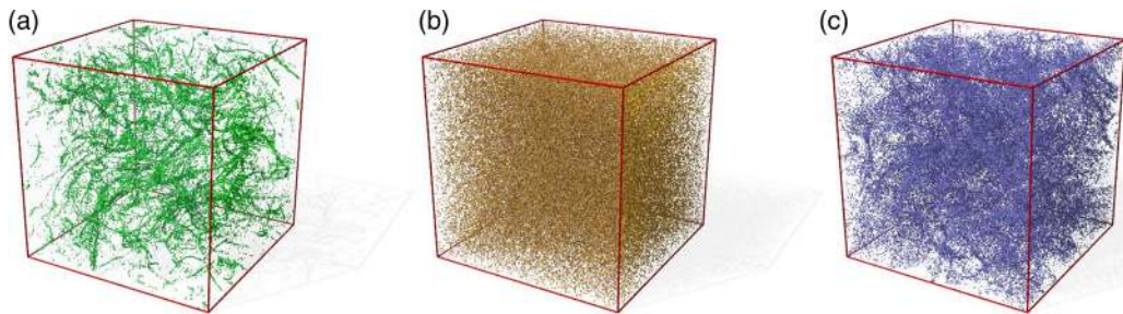
FIG. 25. Snapshots of the particle distribution in turbulent flow field for a Stokes number St = 0.6 for (a) bubbles, (b) tracers, and (c) heavy particles, all for a Taylor-Reynolds number Re_\lambda = 75 , obtained with the point-particle approach in the spirit of Maxey and Riley [175]. The figure has been taken from Ref. [192].
