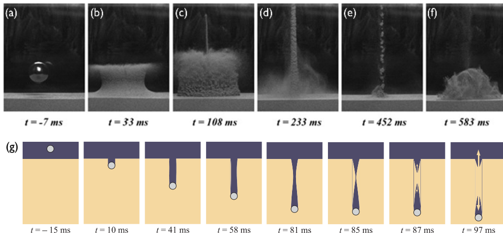
FIG. 12. (a)–(f) Impact (at t = 0 \text{ s} ) of a steel ball (diameter 2.5 \text{ cm} ) on soft decompactified sand (grain diameter typically 40 \mu\text{m} ). The splash and the jet emerge, just as in water. The grains in the jet cluster due to their inelastic collisions. The last frame shows a granular eruption caused by the rising air bubble. (g) Cross section of the void collapse following from the axially symmetric Rayleigh-type model of Ref. [76]. The void is pressed together by the hydrostatic pressure from the side, leading to a singularity and an upward and downward jet. Both series of images have been taken from Ref. [76].
