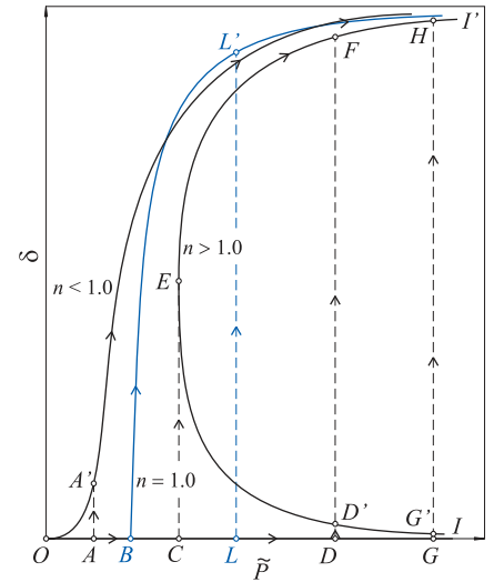
Fig. 6 (online colour at: www.zamm-journal.org ) Sketch of the \tilde{P} - \tilde{\delta} curve.
