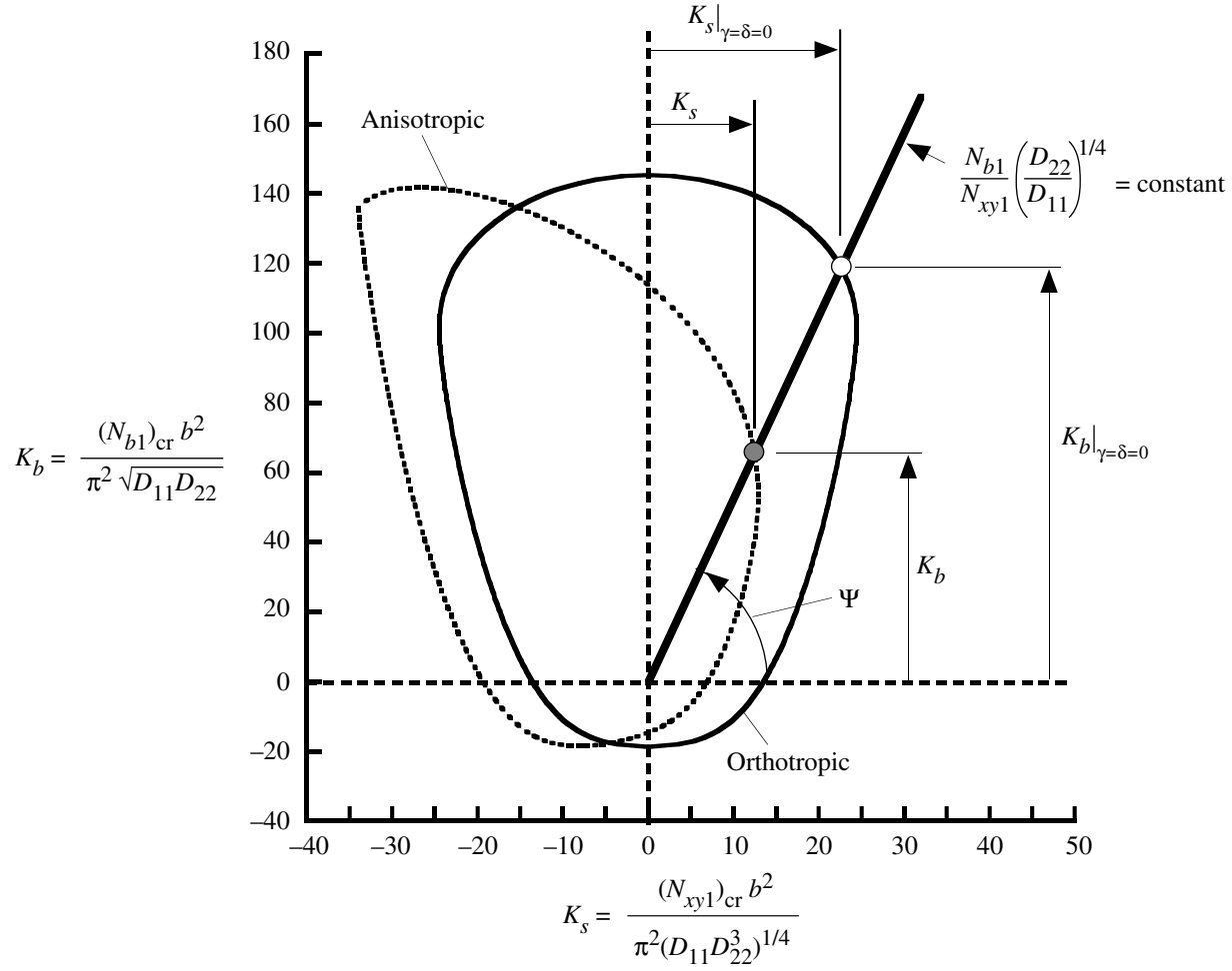
Figure 29. Illustration of stiffness-weighted load ratio angle \Psi for specially orthotropic and anisotropic plates subjected to shear and linearly varying edge loads.
