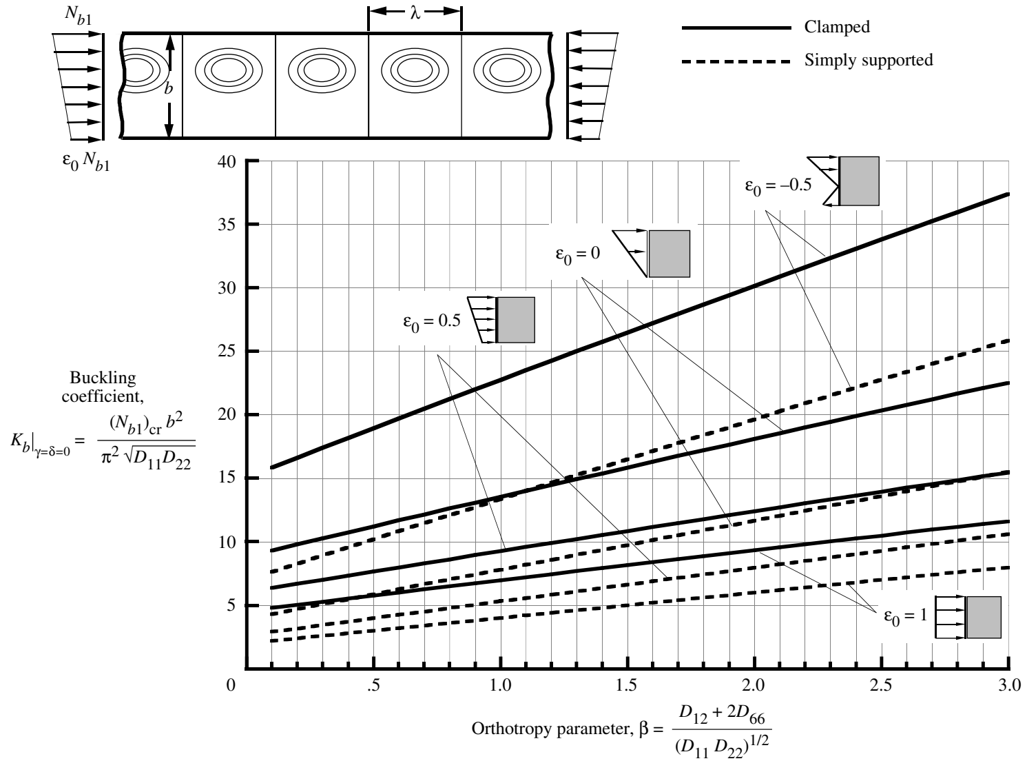
Figure 7. Effect of orthotropy parameter \beta on buckling coefficients for specially orthotropic plates ( \gamma = \delta = 0 ) subjected to linearly varying edge loads ( \epsilon_0 = -0.5, 0, 0.5, \text{ and } 1 ).
