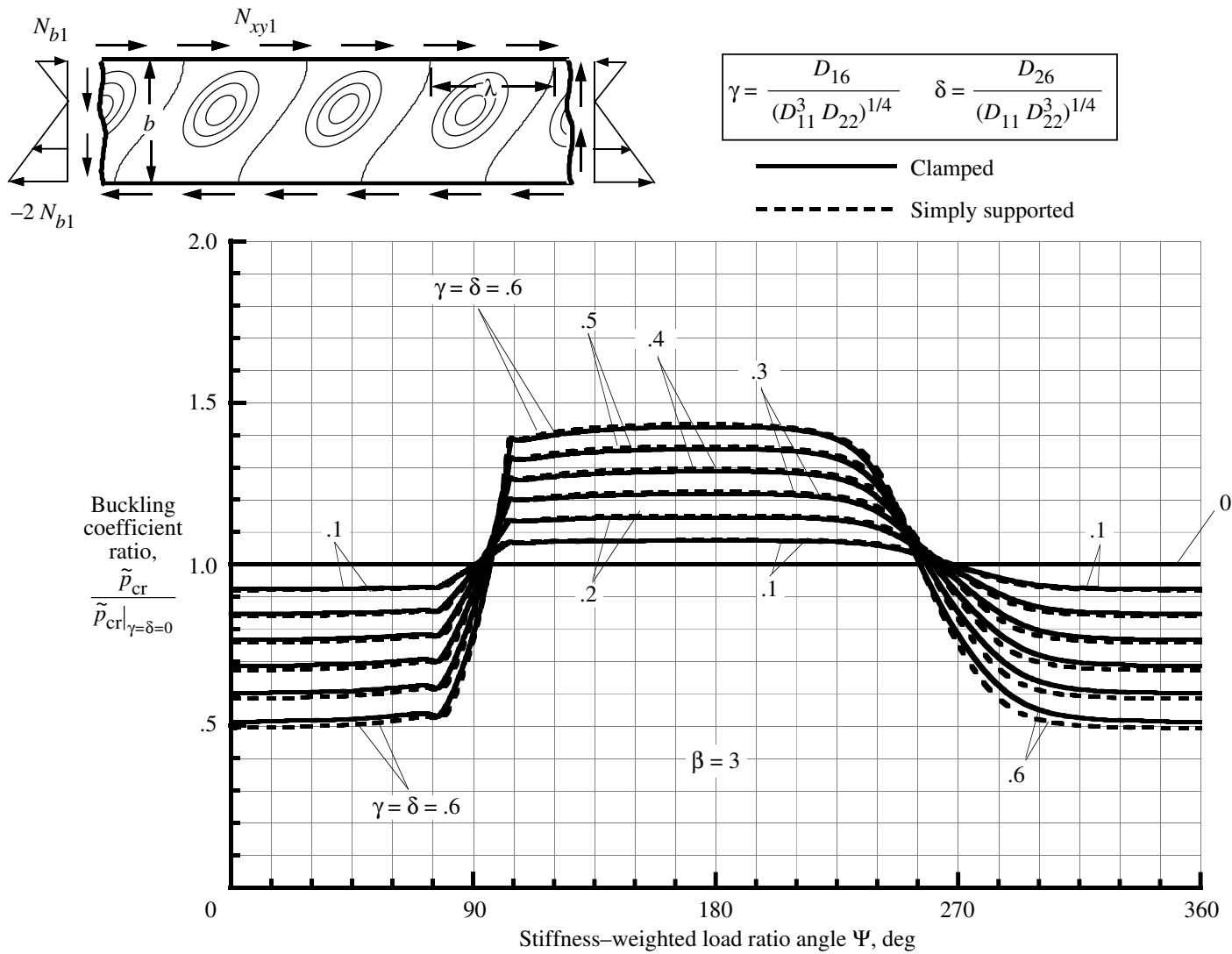
Figure 32. Effect of anisotropy parameters and stiffness-weighted load ratio angle \Psi on behavior of plates subjected to shear and linearly varying edge loads ( \beta = 3 ; \epsilon_0 = -2 ).
