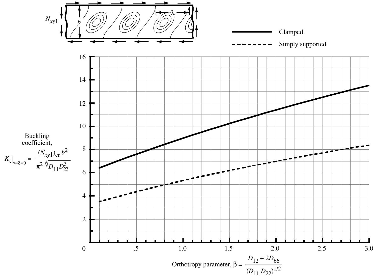
Figure 11. Effect of orthotropy parameter \beta on buckling coefficients for specially orthotropic plates ( \gamma = \delta = 0 ) subjected to shear loads.
