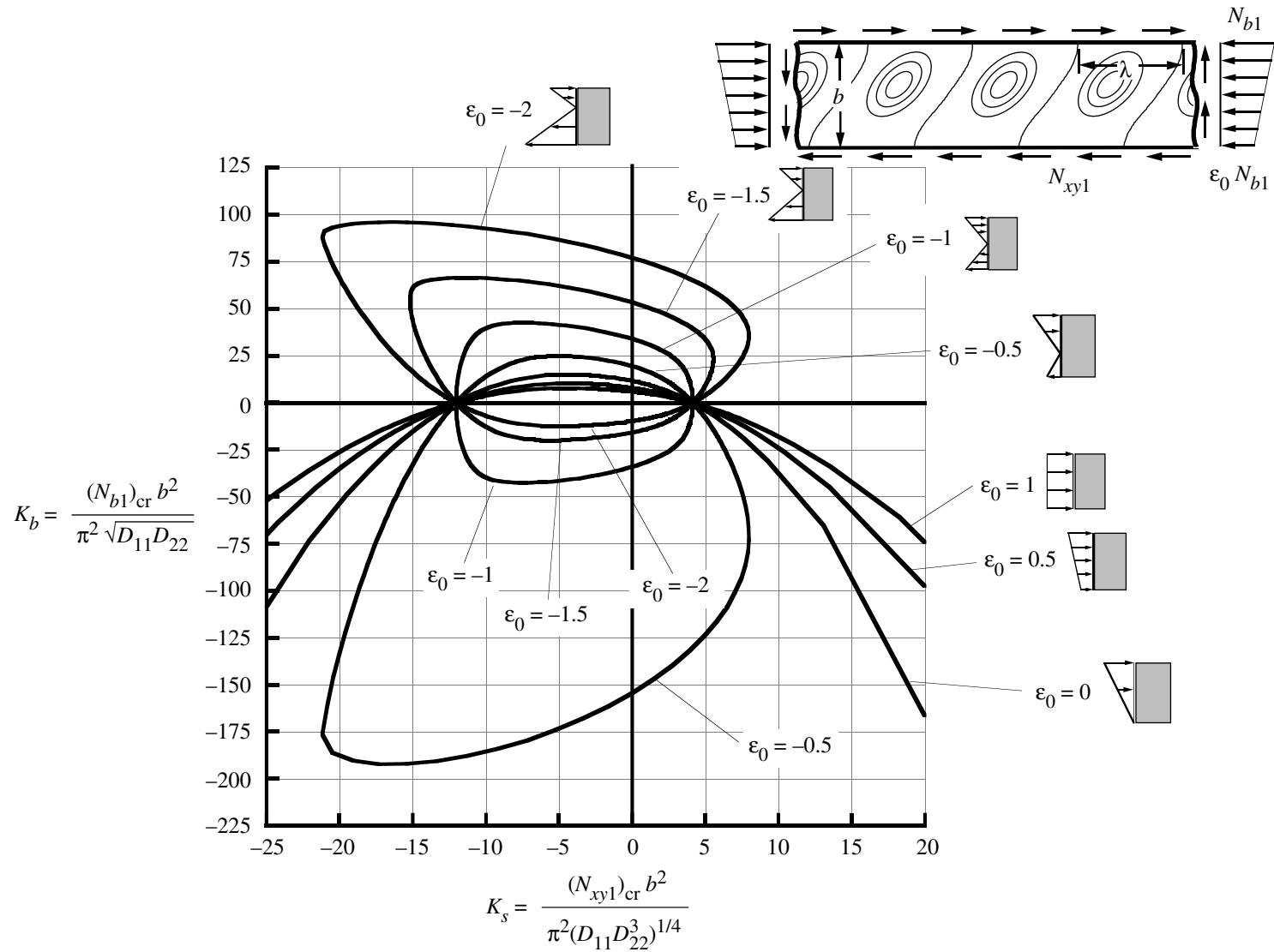
Figure 30. Effect of load distribution parameter \epsilon_0 on buckling interaction curves for simply supported anisotropic plates subjected to shear and linearly varying edge loads ( \beta = 3 ; \gamma = \delta = 0.6 ).
