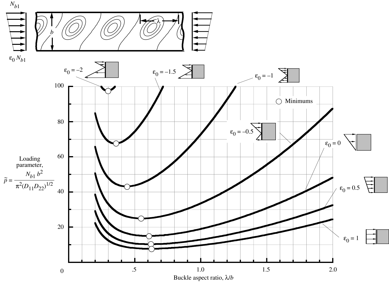
Figure 3. Buckling results for clamped [\pm 45]_s plates subjected to linearly varying edge loads.
