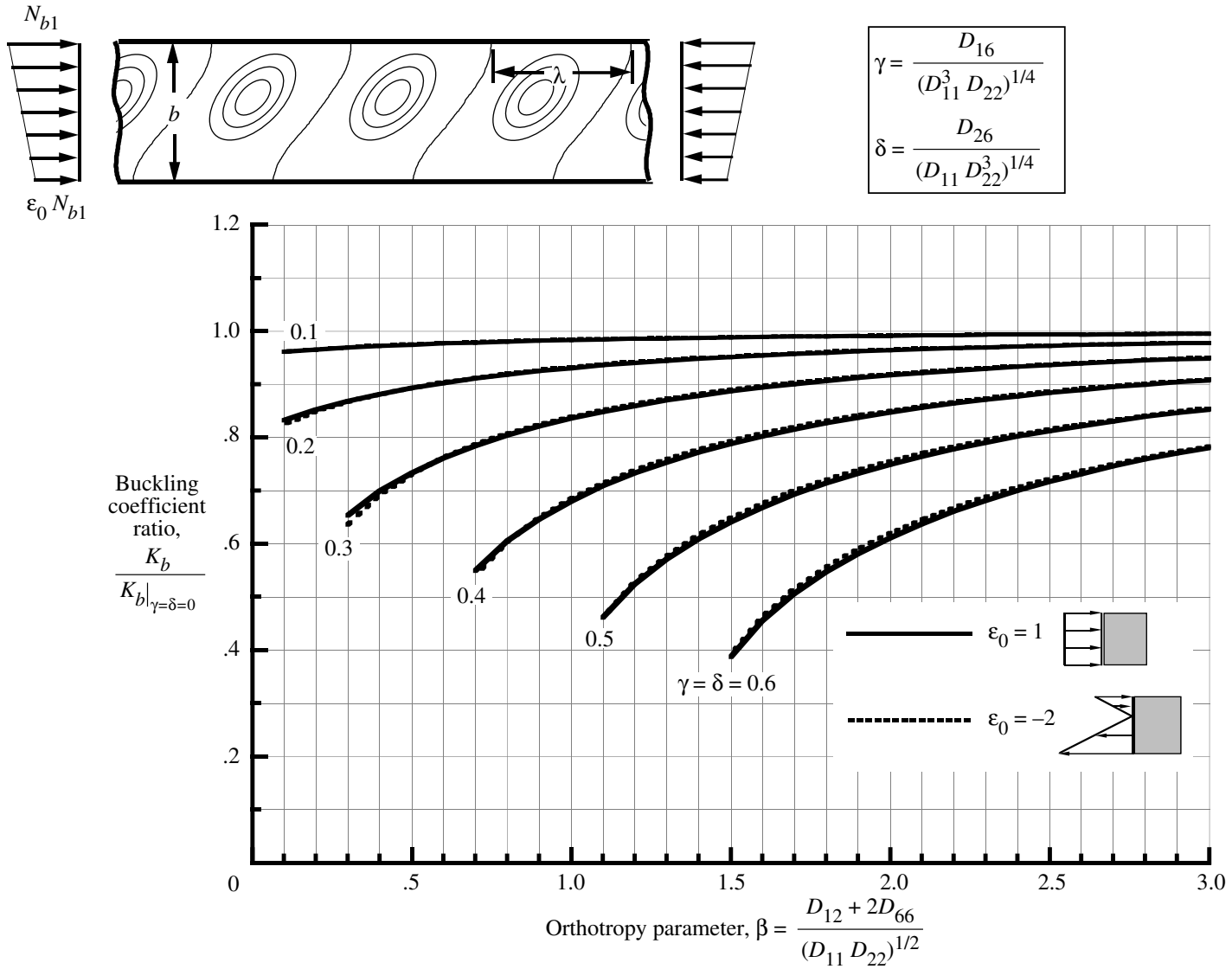
Figure 13. Effect of orthotropy parameter \beta and anisotropy parameters \gamma and \delta on buckling coefficients for clamped plates subjected to linearly varying edge loads.
