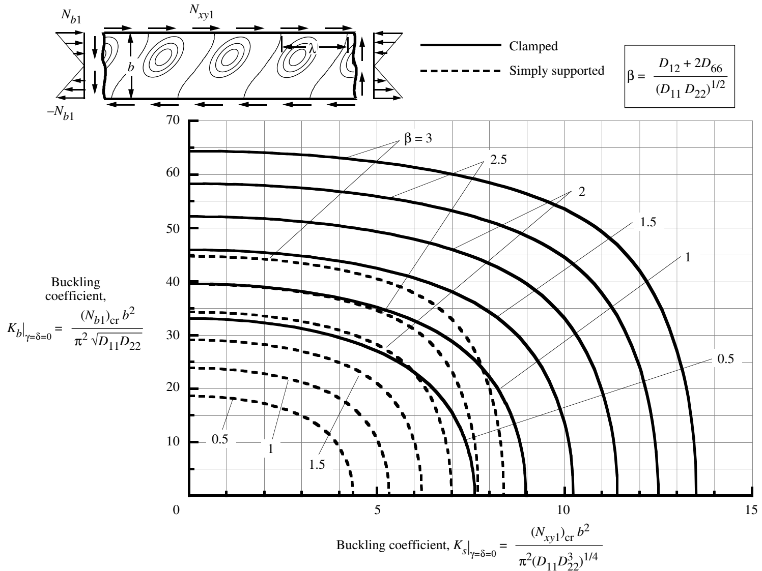
Figure 24. Effect of orthotropy parameter \beta on buckling interaction curves for specially orthotropic plates ( \gamma = \delta = 0 ) subjected to shear and linearly varying edge loads ( \epsilon_0 = -1 ).
