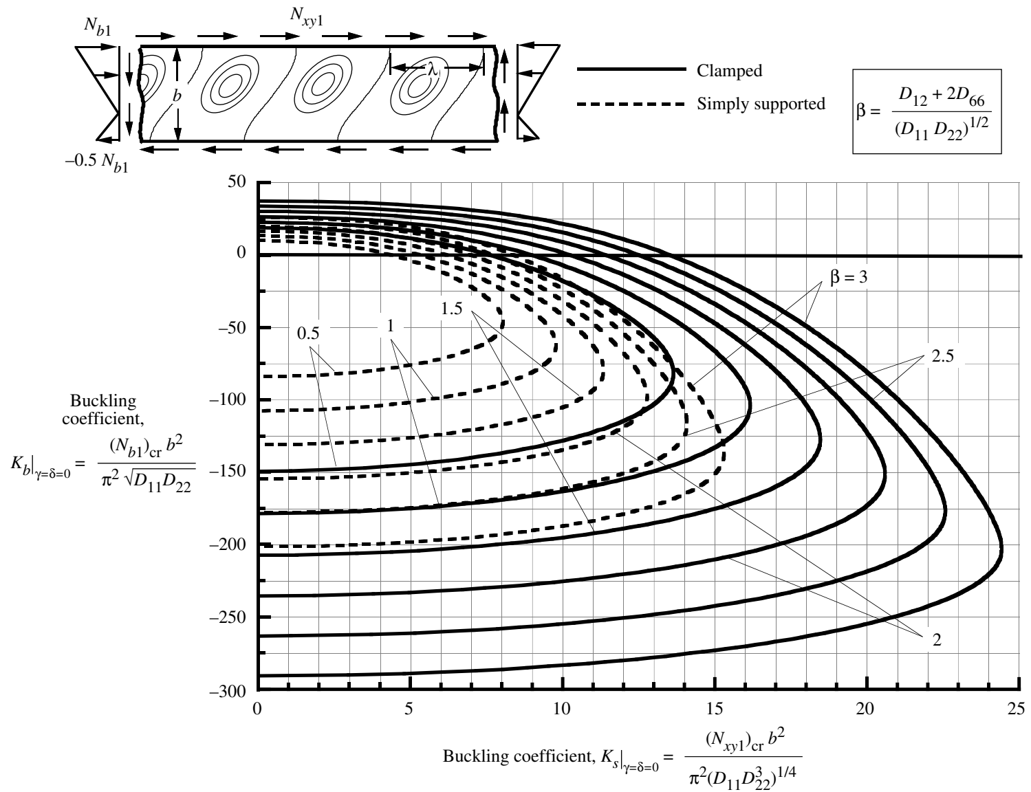
Figure 25. Effect of orthotropy parameter \beta on buckling interaction curves for specially orthotropic plates ( \gamma = \delta = 0 ) subjected to shear and linearly varying edge loads ( \epsilon_0 = -0.5 ).
