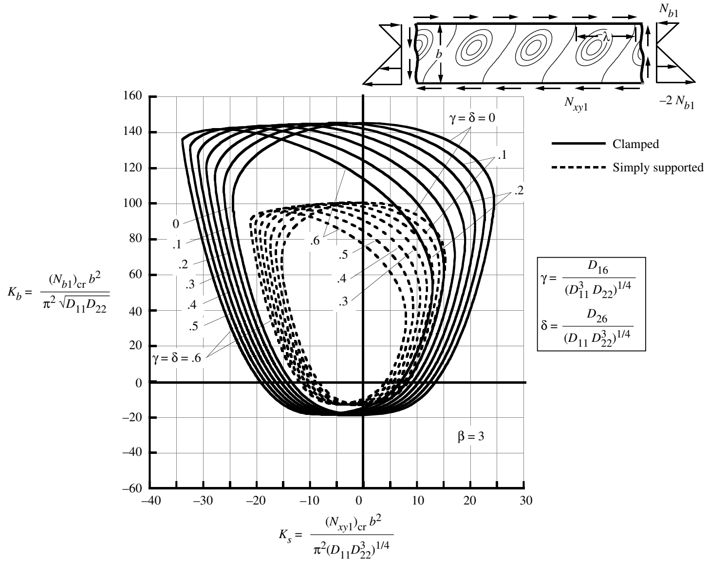
Figure 31. Effect of anisotropy parameters \gamma and \delta on buckling interaction curves for plates subjected to shear and linearly varying edge loads ( \beta = 3 ; \epsilon_0 = -2 ).
