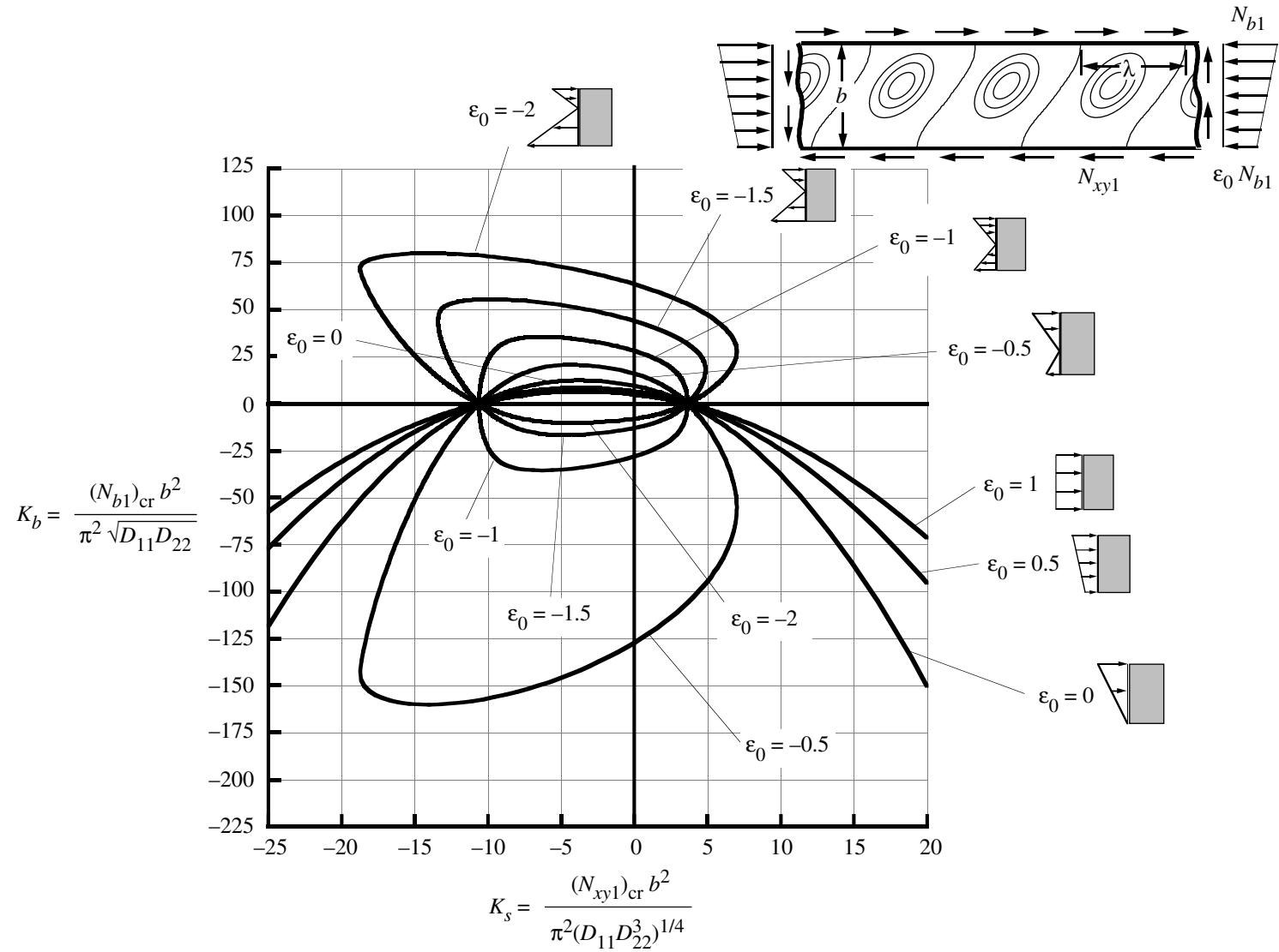
Figure 19. Effect of load distribution parameter \epsilon_0 on buckling interaction curves for [\pm 45]_s simply supported plates subjected to linearly varying edge loads and shear loads (anisotropy included).
