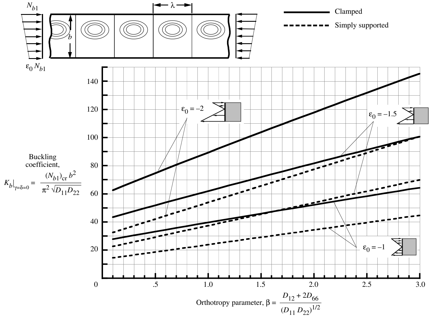
Figure 6. Effect of orthotropy parameter \beta on buckling coefficients for specially orthotropic plates ( \gamma = \delta = 0 ) subjected to linearly varying edge loads ( \epsilon_0 = -2, -1.5, \text{ and } -1 ).
