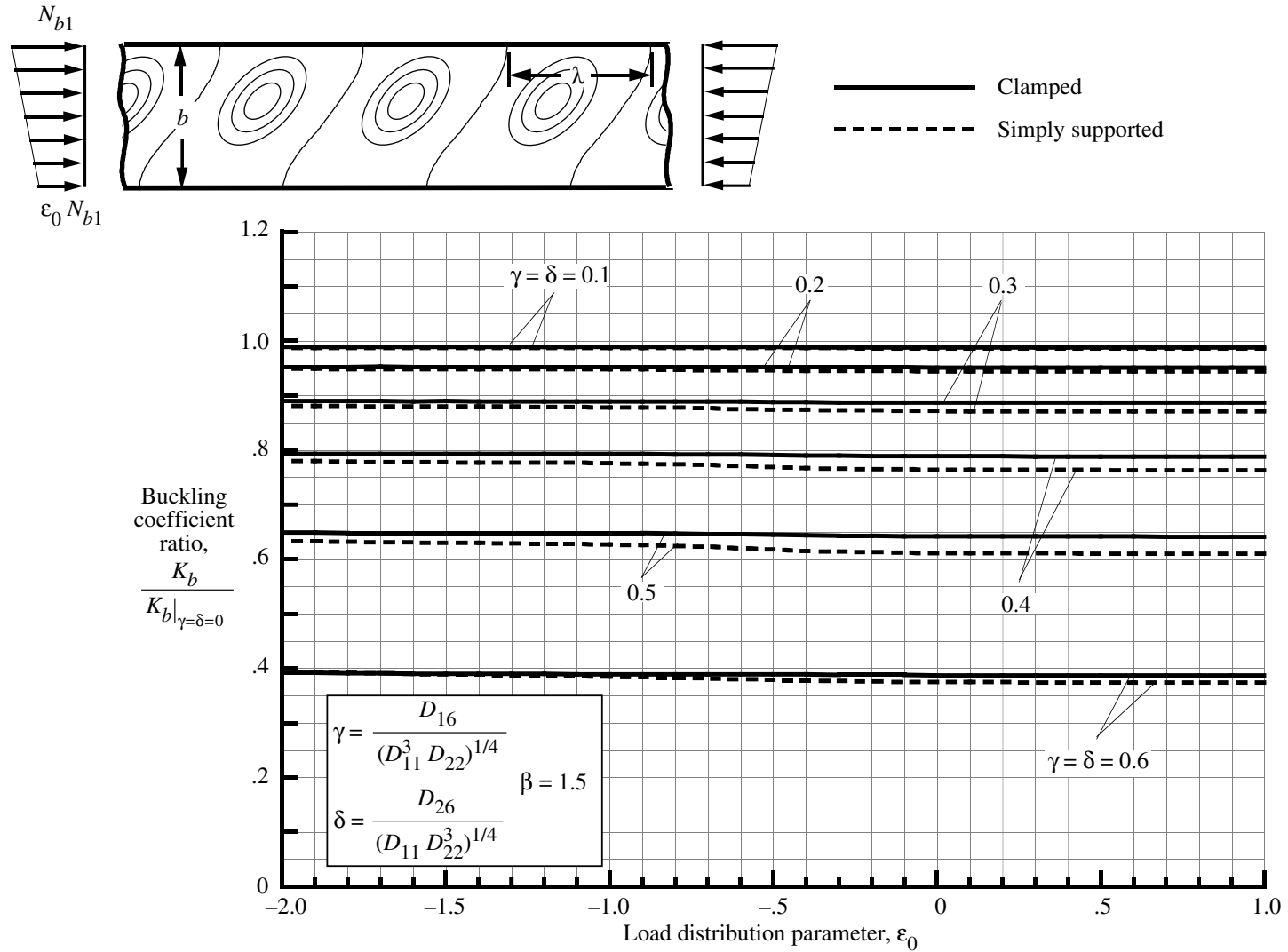
Figure 15. Effect of load distribution parameter \epsilon_0 and anisotropy parameters \gamma and \delta on buckling coefficients for plates subjected to linearly varying edge loads ( \beta = 1.5 ).
