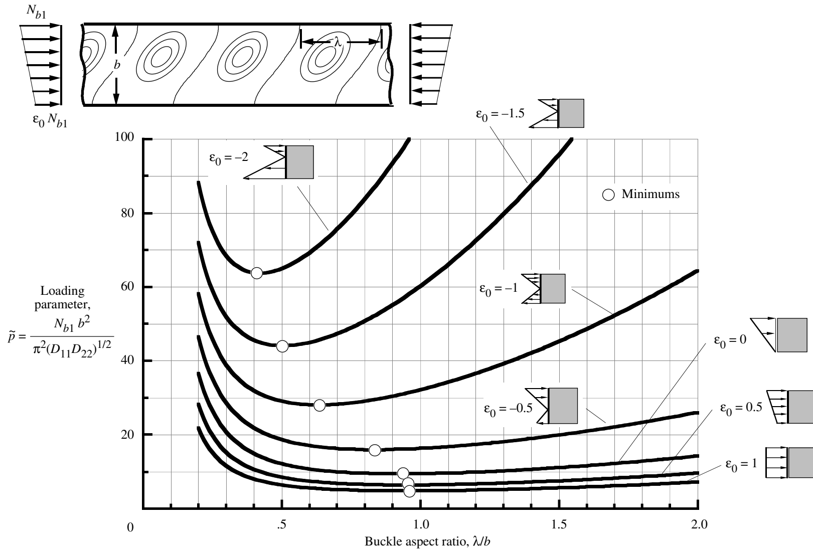
Figure 2. Buckling results for simply supported [\pm 45]_s plates subjected to linearly varying edge loads.
