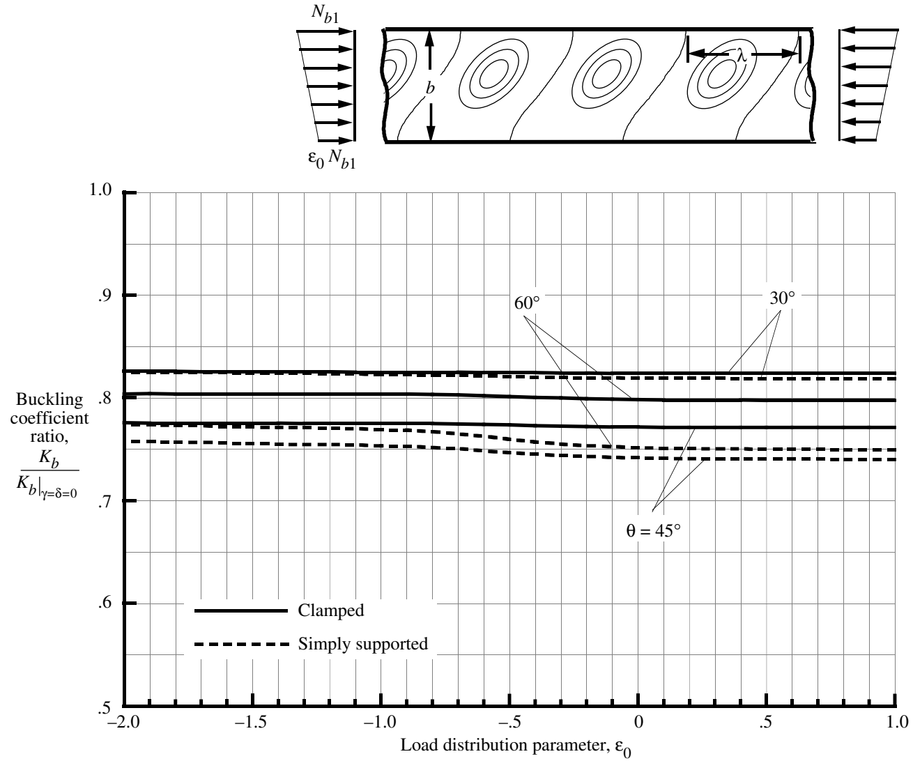
Figure 5. Ratio of anisotropic-to-orthotropic buckling coefficient for simply supported and clamped [\pm\theta]_s plates subjected to linearly varying edge loads.
