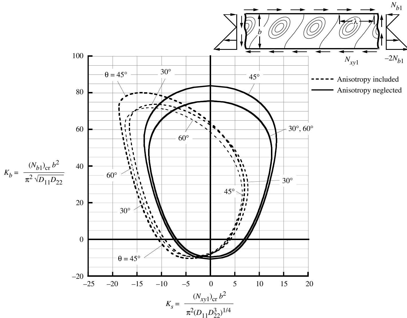
Figure 20. Importance of anisotropy on buckling interaction curves for [\pm\theta]_s simply supported plates subjected to linearly varying edge loads ( \epsilon_0 = -2 ) and shear loads.
