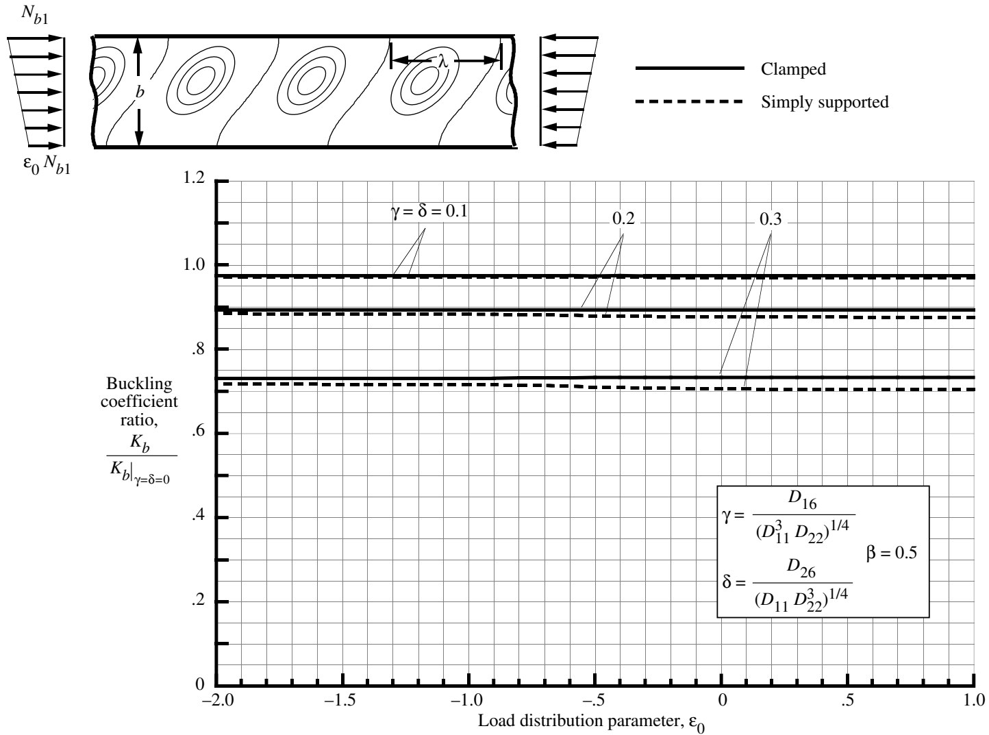
Figure 16. Effect of load distribution parameter \epsilon_0 and anisotropy parameters \gamma and \delta on buckling coefficients for plates subjected to linearly varying edge loads ( \beta = 0.5 ).
