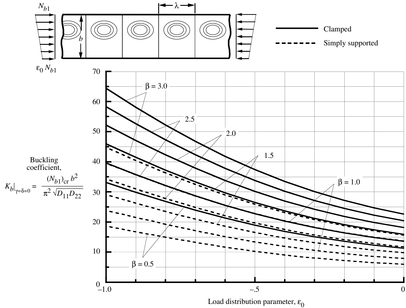
Figure 9. Effect of load distribution parameter \varepsilon_0 on buckling coefficients for specially orthotropic plates ( \gamma = \delta = 0 ) subjected to linearly varying edge loads.
