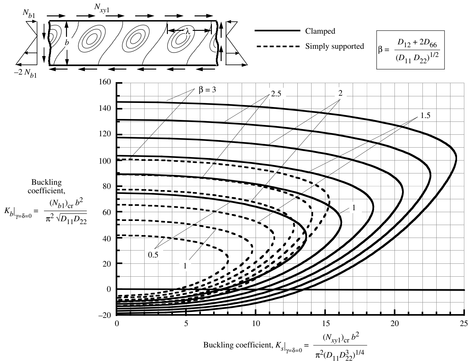
Figure 22. Effect of orthotropy parameter \beta on buckling interaction curves for specially orthotropic plates ( \gamma = \delta = 0 ) subjected to shear and linearly varying edge loads ( \epsilon_0 = -2 ).
