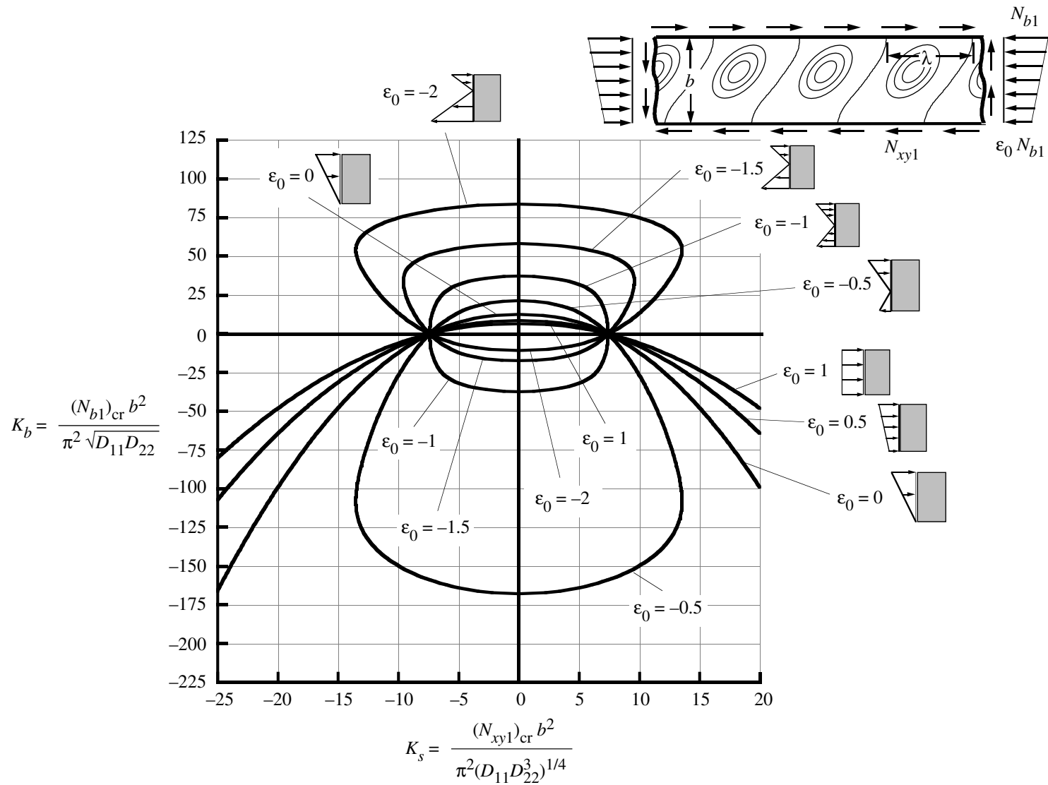
Figure 18. Effect of load distribution parameter \epsilon_0 on buckling interaction curves for [\pm 45]_s simply supported plates subjected to linearly varying edge loads and shear loads (anisotropy neglected).
