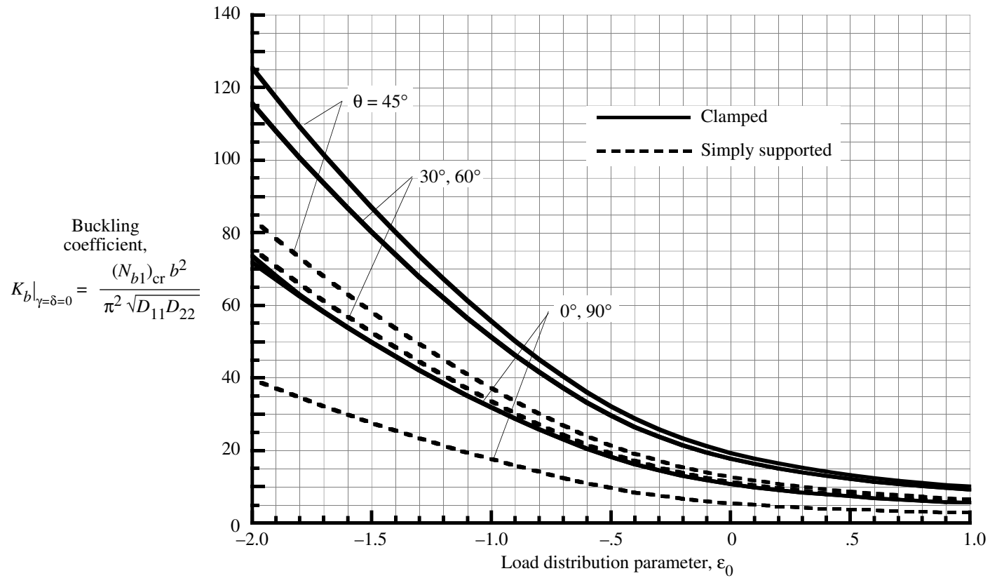
Figure 4. Buckling coefficients for simply supported and clamped [\pm\theta]_s plates subjected to linearly varying edge loads (anisotropy neglected in the analysis).
