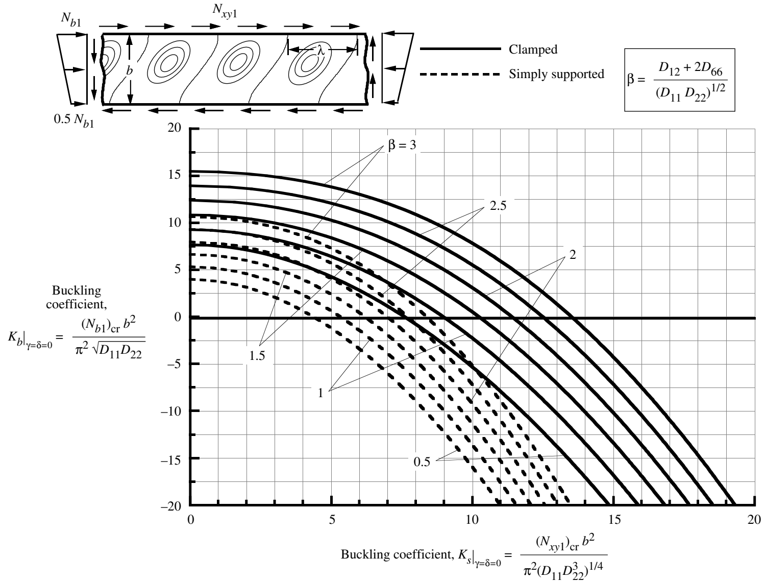
Figure 27. Effect of orthotropy parameter \beta on buckling interaction curves for specially orthotropic plates ( \gamma = \delta = 0 ) subjected to shear and linearly varying edge loads ( \epsilon_0 = 0.5 ).
