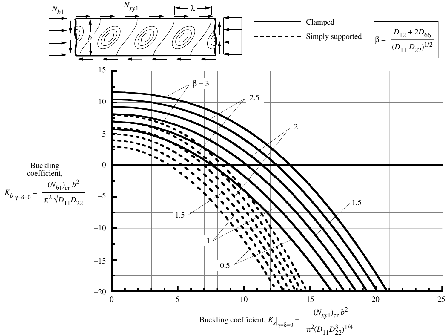
Figure 28. Effect of orthotropy parameter \beta on buckling interaction curves for specially orthotropic plates ( \gamma = \delta = 0 ) subjected to shear and linearly varying edge loads ( \epsilon_0 = 1 ).
