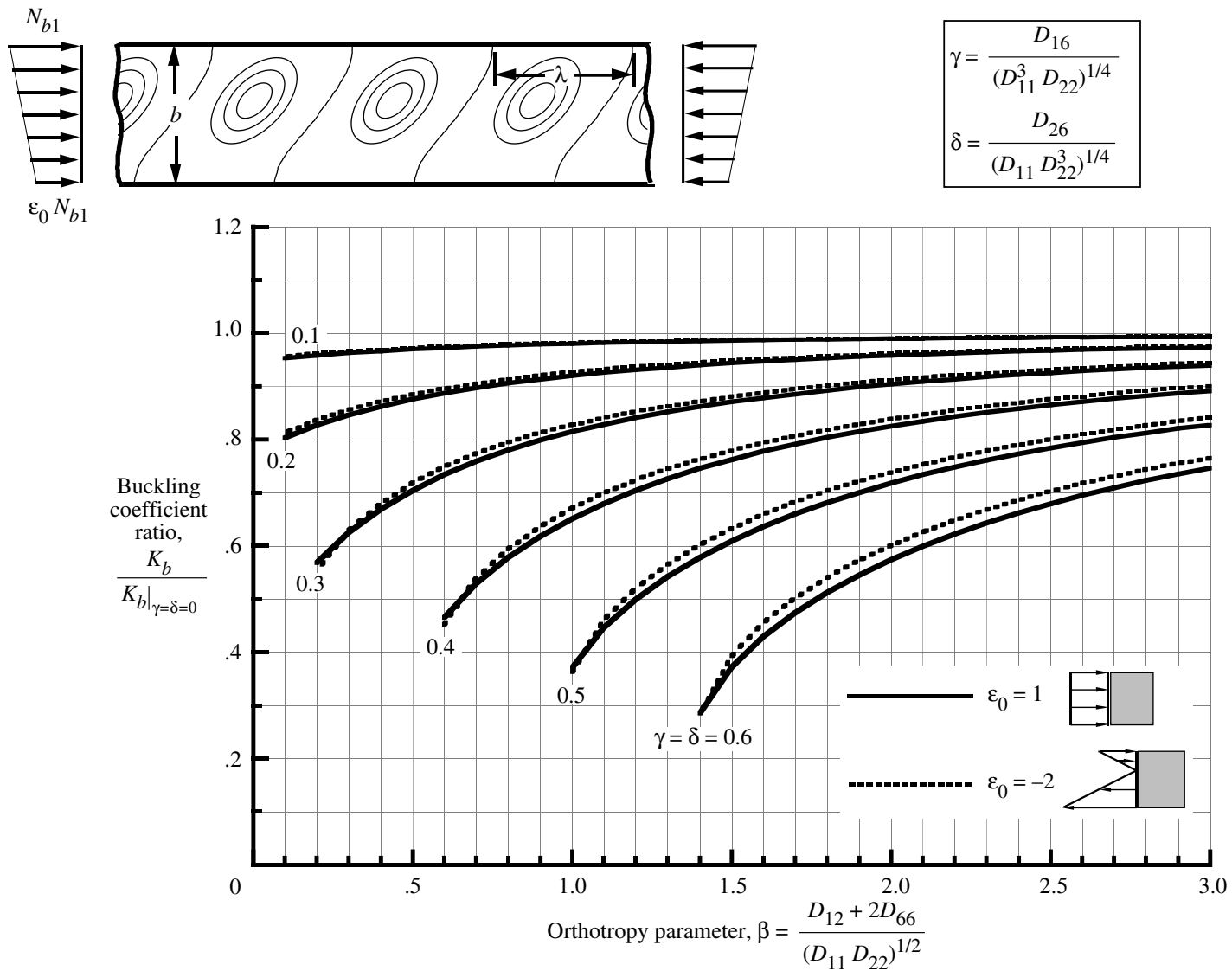
Figure 12. Effect of orthotropy parameter \beta and anisotropy parameters \gamma and \delta on buckling coefficients for simply supported plates subjected to linearly varying edge loads.
