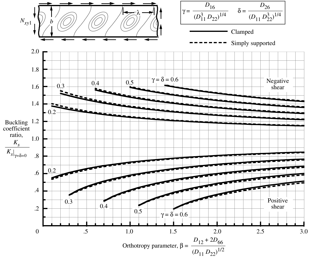
Figure 17. Effect of orthotropy parameter \beta and anisotropy parameters \gamma and \delta on buckling coefficients for plates subjected to shear loads.
