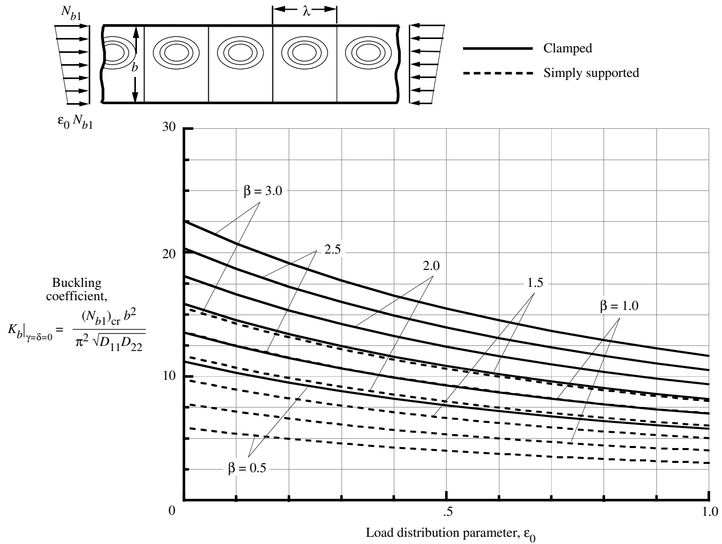
Figure 10. Effect of load distribution parameter \epsilon_0 on buckling coefficients for specially orthotropic plates ( \gamma = \delta = 0 ) subjected to linearly varying edge loads.
