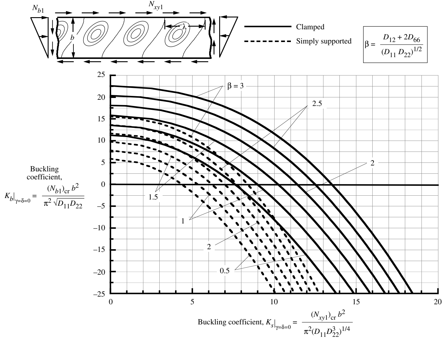
Figure 26. Effect of orthotropy parameter \beta on buckling interaction curves for specially orthotropic plates ( \gamma = \delta = 0 ) subjected to shear and linearly varying edge loads ( \epsilon_0 = 0 ).
