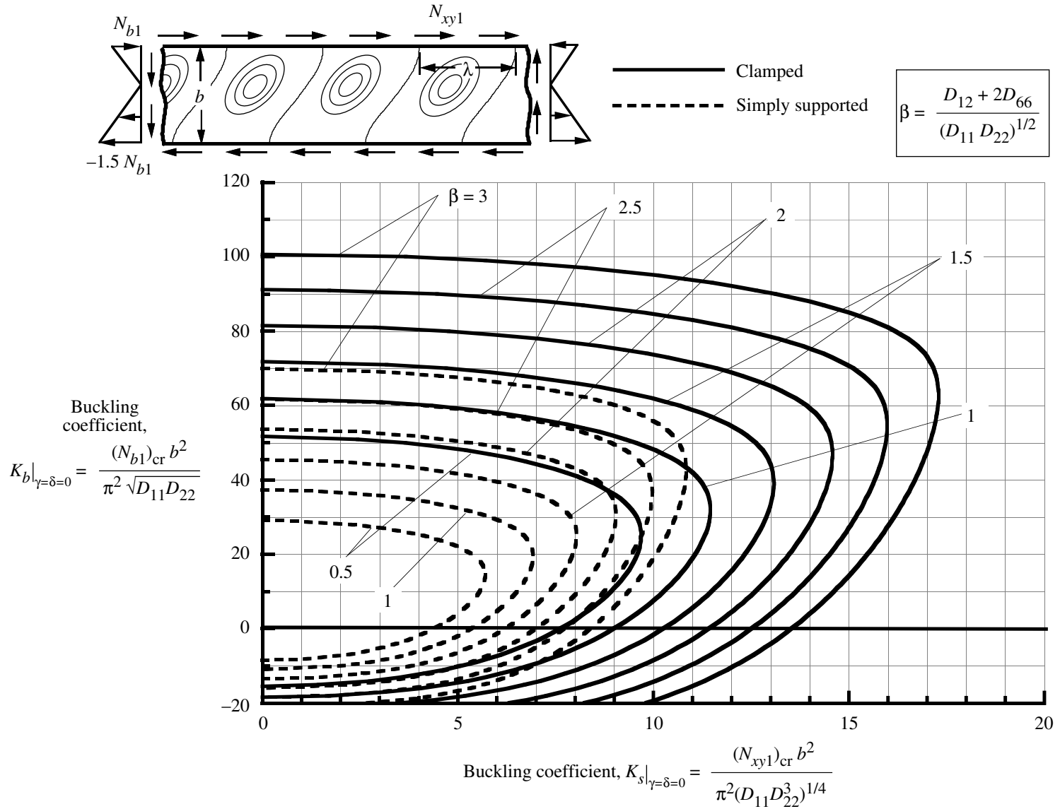
Figure 23. Effect of orthotropy parameter \beta on buckling interaction curves for specially orthotropic plates ( \gamma = \delta = 0 ) subjected to shear and linearly varying edge loads ( \epsilon_0 = -1.5 ).
