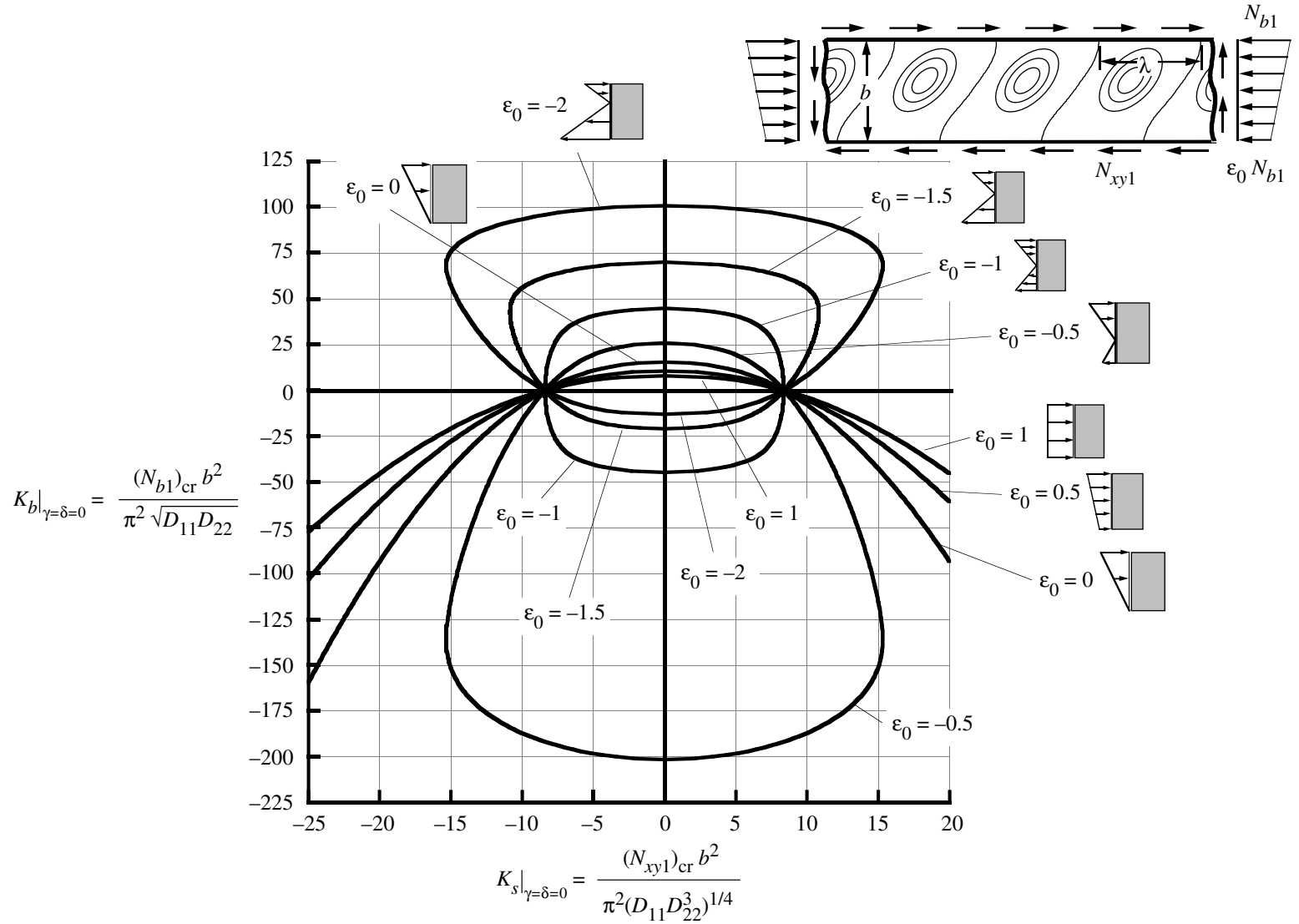
Figure 21. Effect of load distribution parameter \epsilon_0 on buckling interaction curves for simply supported specially orthotropic plates subjected to shear and linearly varying edge loads ( \beta = 3 ).
