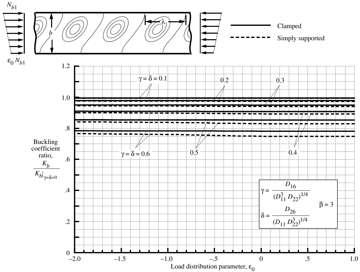
Figure 14. Effect of load distribution parameter \epsilon_0 and anisotropy parameters \gamma and \delta on buckling coefficients for plates subjected to linearly varying edge loads ( \beta = 3 ).
