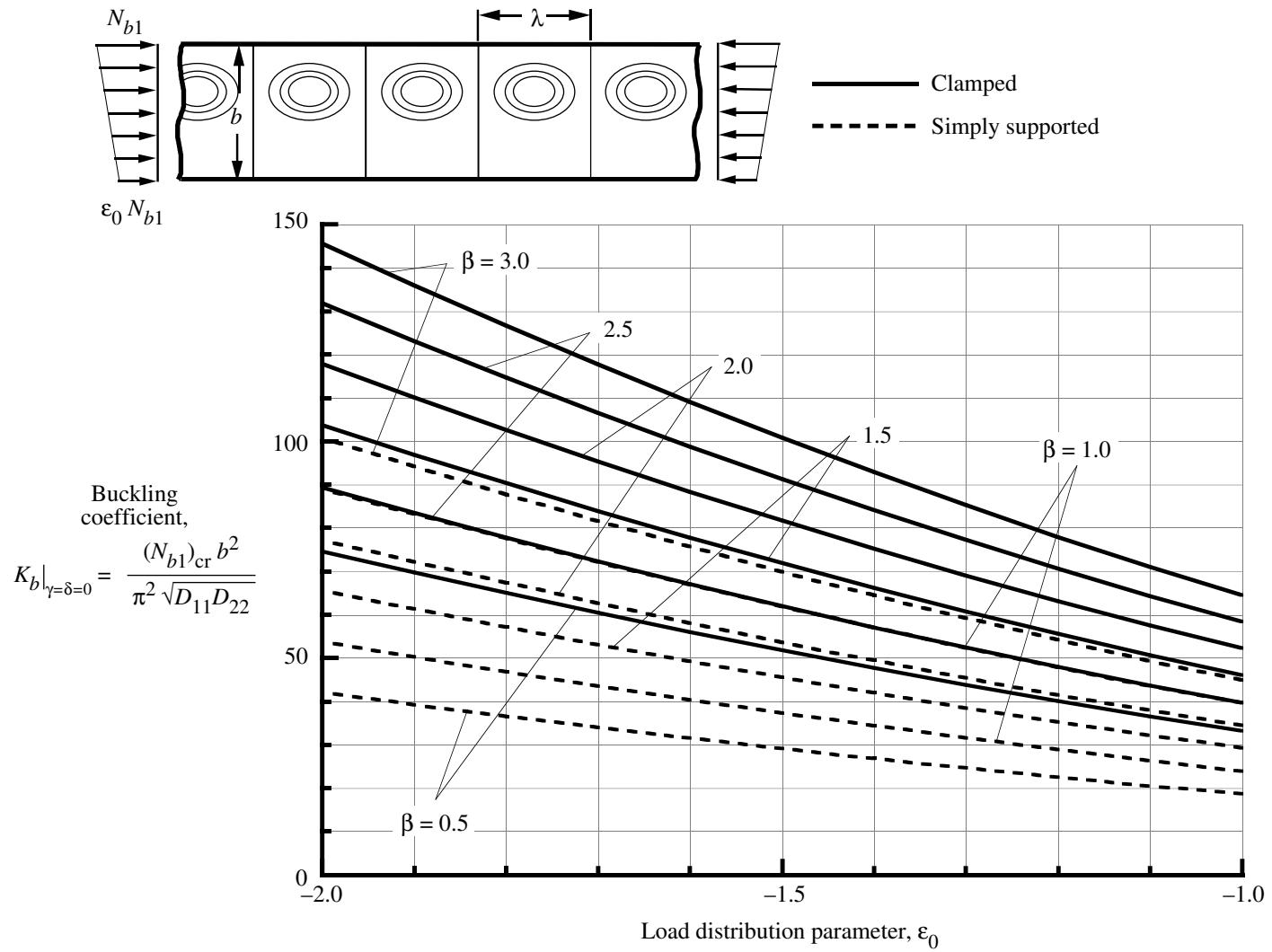
Figure 8. Effect of load distribution parameter \epsilon_0 on buckling coefficients for specially orthotropic plates ( \gamma = \delta = 0 ) subjected to linearly varying edge loads.
