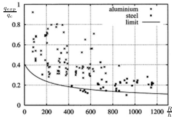
Figure 1: Experimental results for spherical shells under external pressure, published in [3].
