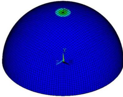
Figure 5: FE model and deformed shell under external pressure and concentrated load just before buckling.
