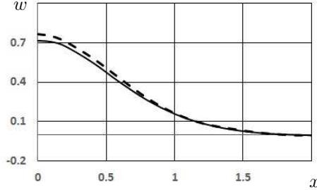
Figure 4: Deflection diagram at intermediate post-buckling shell stage.
