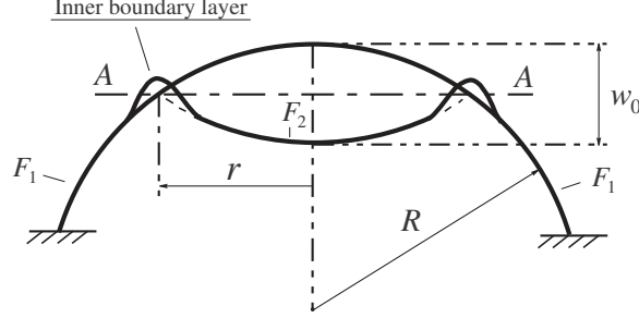
Figure 2: Spherical shells with large deflections.
