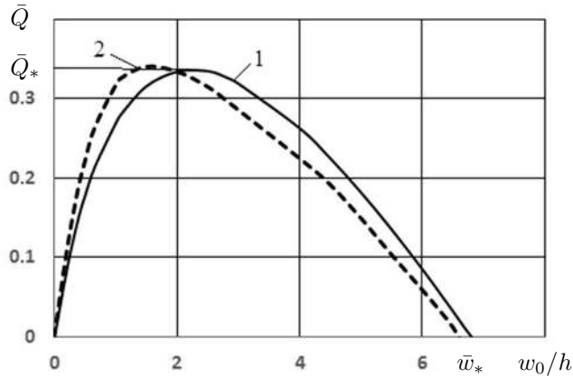
Figure 6: Load deflection diagram obtained for external pressure parameter \bar{q} = 0.2 .
