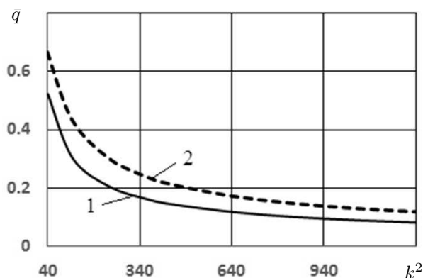
Figure 8: Buckling external pressure parameter versus shell slenderness.
