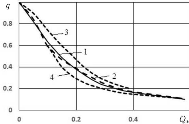
Figure 7: Buckling load combination diagram.
