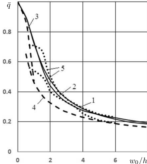
Figure 3: Post-buckling behavior of spherical shell (asymptotic, numerical and experimental results).
