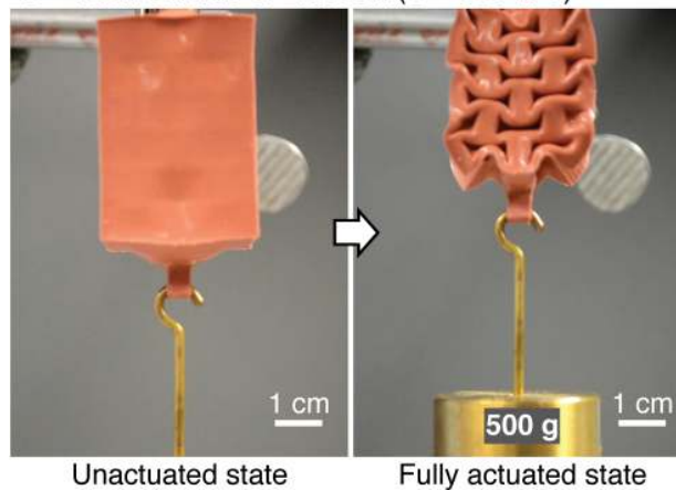
D VAMPs made of Elastosil ( E = 520 kPa)
