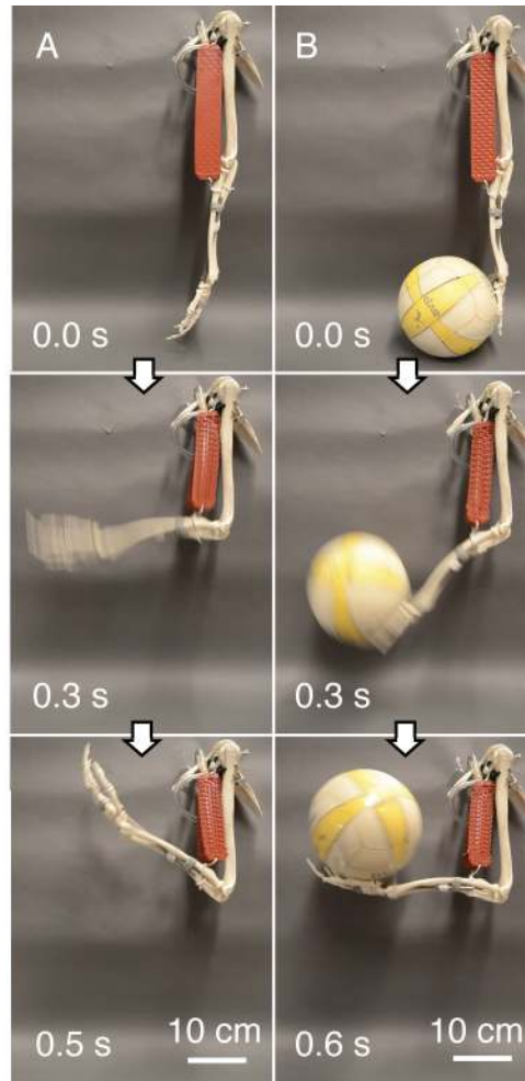
Figure 3. Demonstration of muscle-like actuation. (A) Use of a VAMP to actuate a polymer replica of the bones of a human arm, with mechanics similar to that employed by a human bicep muscle. Here metal wires serve as “tendons” to connect VAMP and replica bone, but high tensile strength polymer fibers could serve equally well. (B) The VAMP-actuated “arm” lifting a standard size and weight (274 g) volleyball. See Movies S4 and S5 for the videos. (See the SI, Figure S5, and Movies S6 and S7 for speed comparison with a fast-moving human arm.)
