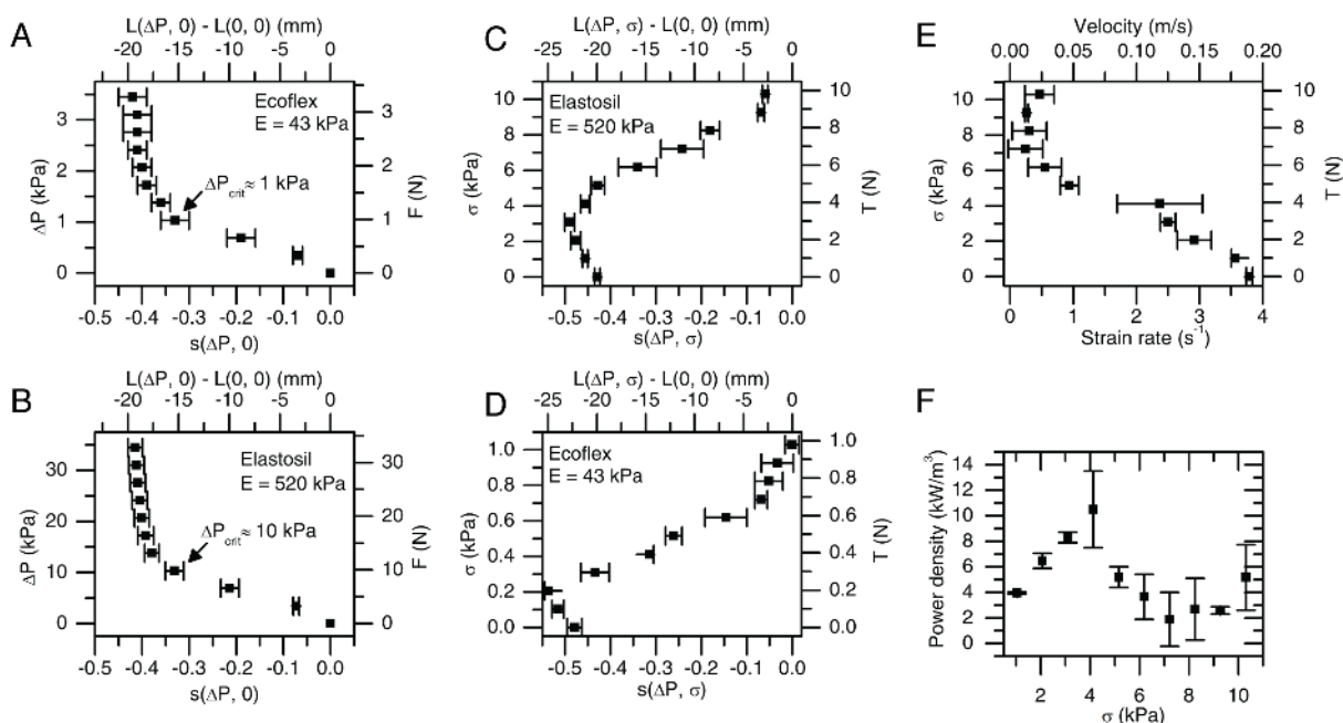
Figure 2. Static and dynamic characteristics of VAMPs. (A, B) Applied differential pressure \Delta P vs. actuation strain s(\Delta P, 0) curves of seven different VAMPs made of Ecoflex ( E = 43 kPa) and Elastosil ( E = 520 kPa) at no load. The critical differential pressure ( \Delta P_{crit} ) at which VAMPs compress almost completely is proportional to the Young's modulus of the material. (C, D) Loading stress \sigma vs. actuation strain s(\Delta P, \sigma) curves of seven different VAMPs made of Ecoflex ( E = 43 kPa) and Elastosil ( E = 520 kPa), when a differential pressure of \Delta P = 90 kPa is applied (i.e. force-length relationship under active loading). A VAMP exerts greater force when fabricated in a stiffer elastomer—an approximately ten-fold increase in the modulus of material results in an approximately ten-fold increase in loading stress. (See the SI for discussions on the shape of the curve.) Reported values for static characteristics are mean \pm S.D. ( n = 7 different samples). (In addition, L(\Delta P, \sigma) - L(0, \sigma) is the change in length of the VAMP, F is the force due to difference of pressure, and T is the total loading force.) (E) The relationship between force and
