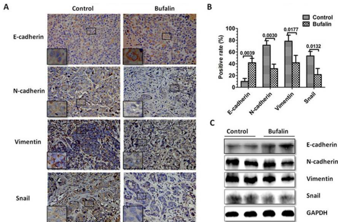
Figure 3: Bufalin inhibits the EMT in vivo . At the end of the experiment in an orthotopic xenograft model, the control and the bufalin-treated tumors were excised and analyzed using immunohistochemistry and western blot to measure the expression of EMT markers. (A) IHC staining with anti-E-cadherin, anti-N-cadherin, anti-vimentin, and anti-Snail antibodies were performed using sections of the orthotopic transplanted tumors. (B) The positive rate of the EMT-related markers E-cadherin, N-cadherin, vimentin and Snail are based on IHC. (C) Western blot analysis was used to measure the expression of the EMT-related markers E-cadherin, N-cadherin, vimentin and Snail in the cells derived from two representative xenograft samples from each group. GAPDH was used as a loading control in the western blot analysis.
