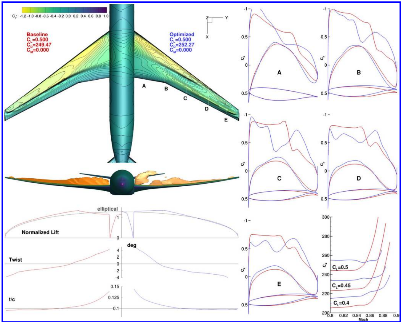
Fig. 14 Baseline analysis compared to the Case 5.2 result. To obtain a small improvement at the highest Mach numbers, performance is sacrificed across a large range of Mach numbers.
