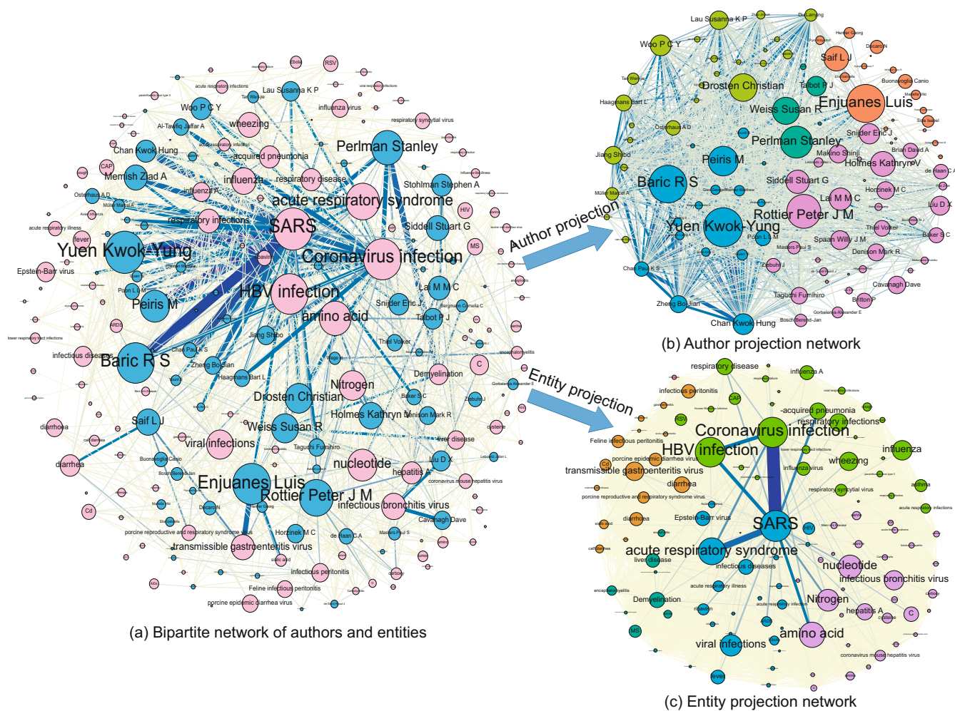
Fig. 5 Bipartite network analysis of coronavirus.
