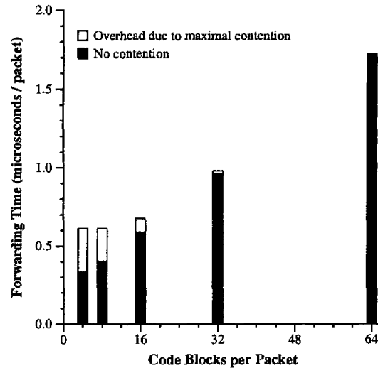
Figure 10: Forwarding time breakdown under maximal output port contention for the case of 10 register instructions and a 4-byte SRAM read per code block. (The “no contention” portion corresponds to the circle points of Figure 9.)
