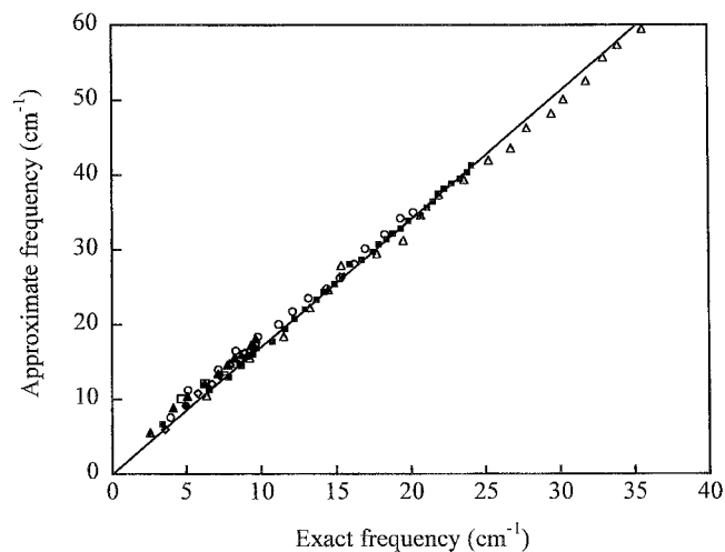
Fig. 1. Approximate frequencies calculated with the RTB approach, each block containing a single amino acid, as a function of the frequencies calculated with standard approaches. Proteins of various sizes were considered (see Table I): crambin (filled triangles), HIV-1 protease (open circles), adenylate kinase (open triangles), triglyceride lipase (open squares), alcohol dehydrogenase (crosses) and enolase (filled diamonds). For the sake of clarity, only some of the approximate values corresponding to exact frequencies calculated in the 10\text{--}20 \text{ cm}^{-1} range are shown.
