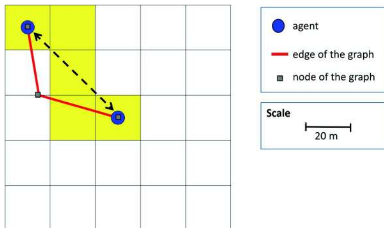
Fig. 4 Computation of distances between two agents (blue circle) according to different GAMA topologies : distance with the continuous topology (Euclidean): 56.6 m; distance with the grid topology (yellow cells): 4 cells, distance with the graph topology (red lines representing roads): 66.8 m
