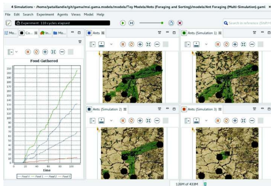
Fig. 5 Example of use of multi-simulation: 4 simulations concerning ant foraging are run in parallel with 4 different sets. The left chart shows in real time the results of the 4 simulations in terms of food gathered
