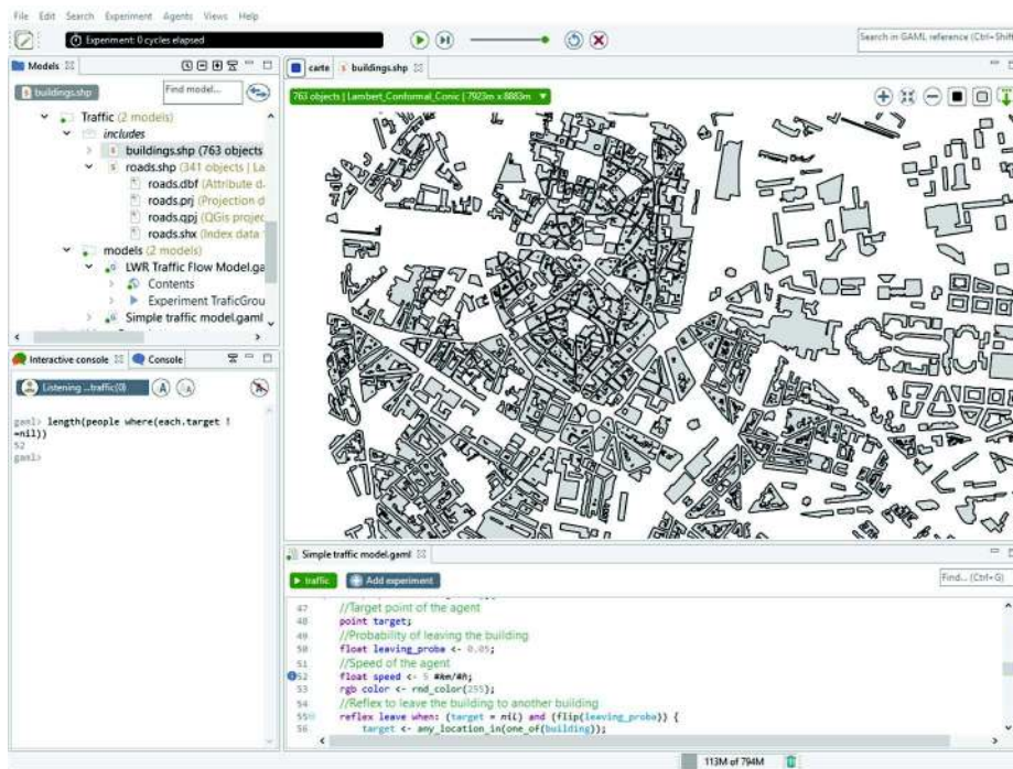
Fig. 1 Modeling interface of GAMA
