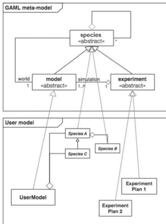
Fig. 2 Main concepts behind GAML
