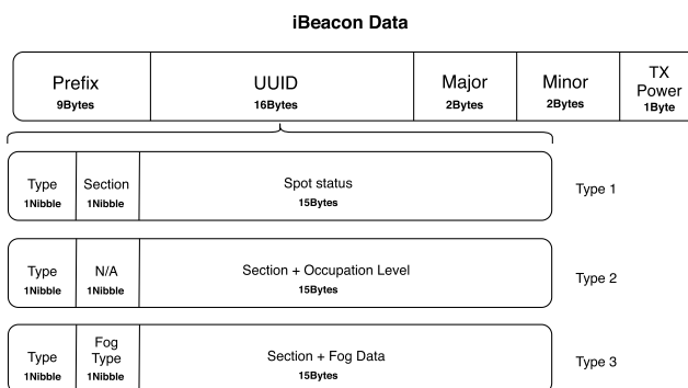
FIGURE 17. Internal structure of the three types of BLE beacons.
