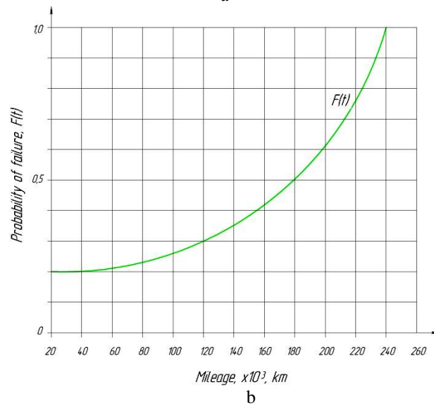
Fig. 1. Dependence of the probability of failure of freight cars from the path: a – the mechanical wear; b – fatigue wear
