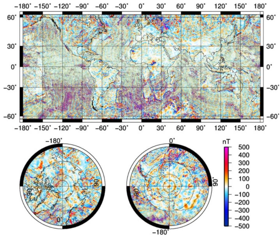
Fig. 7 Global map of the Earth's magnetic anomalies relative to the CM4 main field model for year 1990, divided by the \mathcal{J}_D factor
