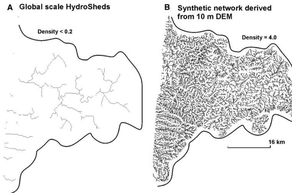
Fig. 6 a The global scale HydroSheds has a very low drainage density in the Oregon Coast Range, U.S.A. b The same river network showing the synthetic hydrography built using 10-m DEMs in a virtual watershed
