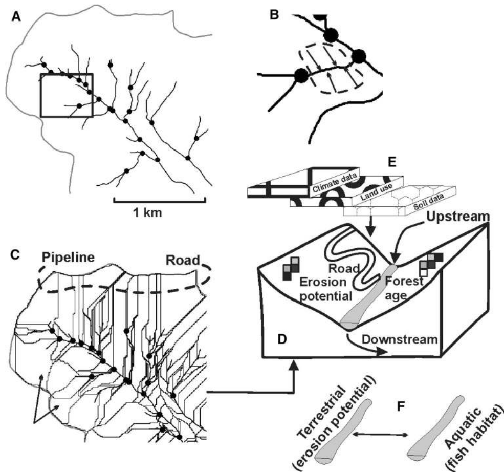
Fig. 8 a A virtual watershed contains a synthetic, attributed and routed river network with individual river segments delineated ( black dots denote tributary confluences). b Each river segment delineates a local contributing area (LCA) on both sides of the channel. c The virtual watershed is discretized into LCAs of appropriate scale; river segments of 100–200 m create LCAs of approximately 0.1 km 2 . Linear features such as roads and pipelines are discretized at pixel scales and associated with similarly scaled indices of other attributes such as erosion. d Each LCA creates similarly scaled terrestrial information including roads, erosion potential, wildfire risk, and
