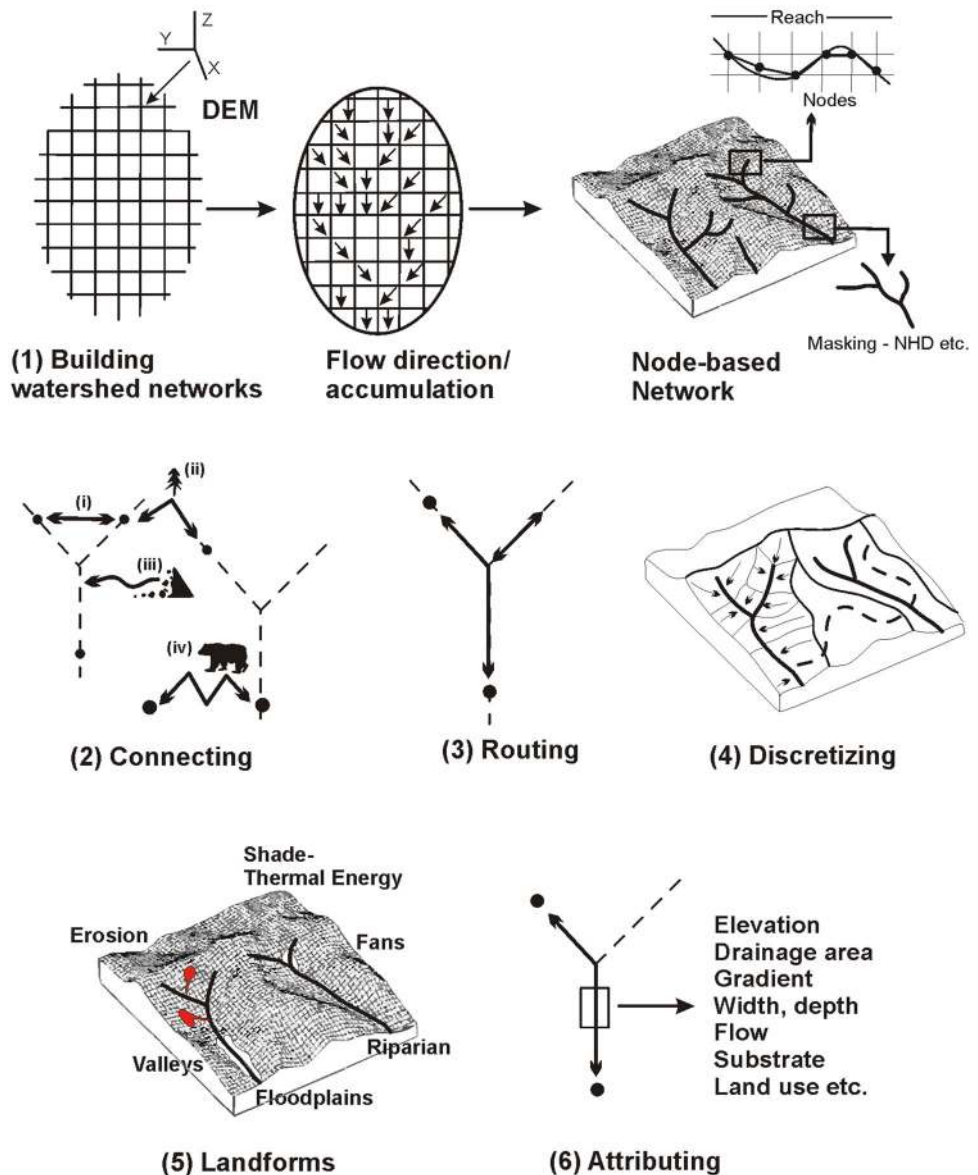
Fig. 7 The coupling of the DEM with synthetic hydrography contains a numerical data structure that support five types of analytical capabilities within a virtual watershed. Multiple connectivity pathways include (i) river connected, (ii) Euclidean distance, (iii) slope distance, (iv) gravity driven flow paths, and (v) modified slope distance
