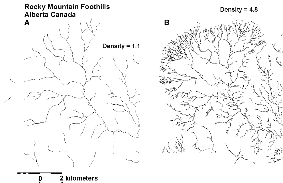
Fig. 1 a A cartographic Provincial stream layer in Alberta, Canada with a low stream density (most headwaters omitted). b A synthetic stream network built using 1 m LiDAR is shown for comparison
