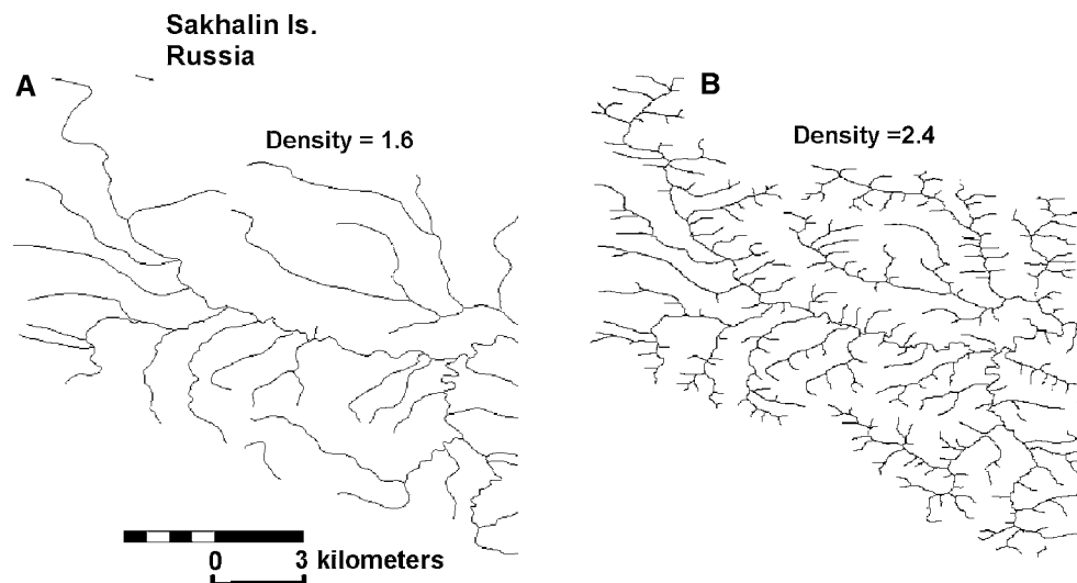
Fig. 3 a The Russian cartographic stream layer for Sakhalin Island has a low stream density (Table 2). b A synthetic stream layer built using 30-m DEMs has a higher channel density but still comparatively low because of the low-resolution DEMs (Table 2)
