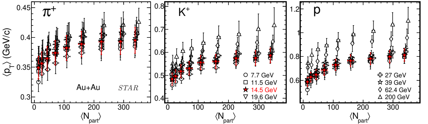
FIG. 8. \langle p_T \rangle of \pi^+ , K^+ and p as a function of \langle N_{\text{part}} \rangle for Au+Au collisions at \sqrt{s_{NN}} = 14.5 GeV. These averages are compared with the corresponding results from Au+Au collisions at \sqrt{s_{NN}} = 7.7, 11.5, 19.6, 27, 39, 62.4, and 200 GeV measured by STAR in earlier runs [32, 60, 65]. Statistical and systematic uncertainties have been added in quadrature.
