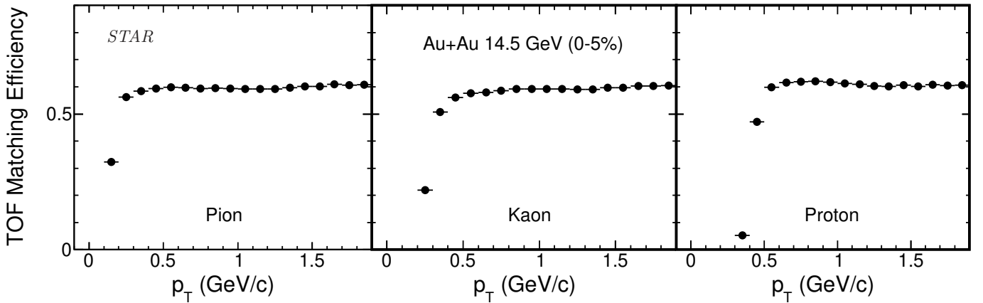
FIG. 6. TOF matching efficiency as a function of p_T for pions (left), kaons (middle) and protons (right) at midrapidity ( |y| < 0.1 ) in 0-5% Au+Au collisions at \sqrt{s_{\text{NN}}} = 14.5 GeV.
