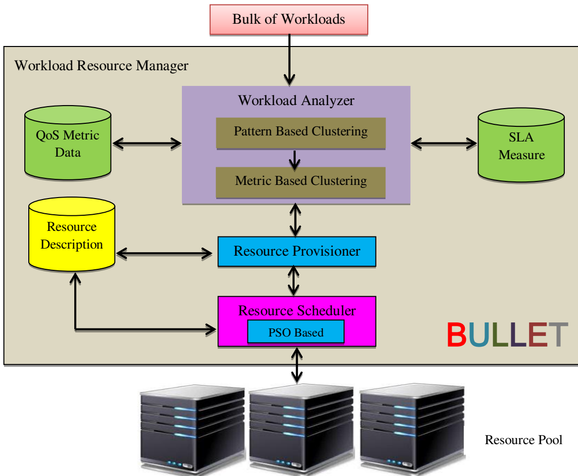
Figure 1: Architecture of BULLET
