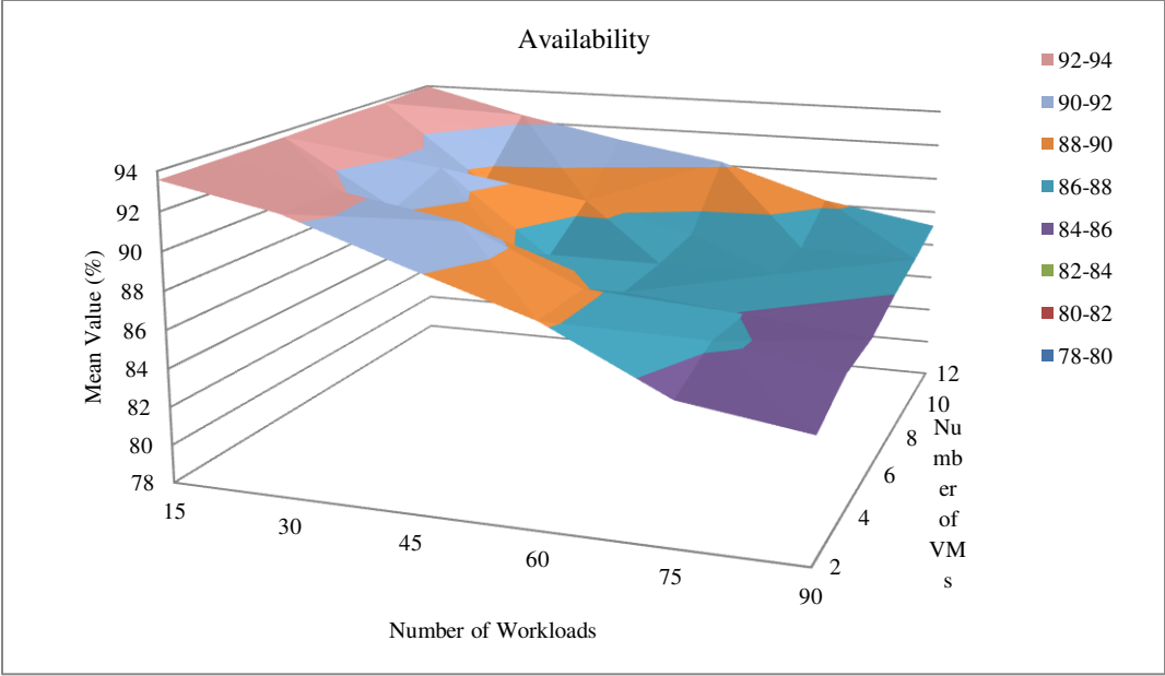
Figure 30: Statistical Analysis of Availability
