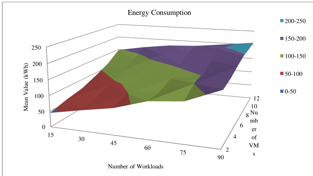
Figure 33: Statistical Analysis of Energy Consumption
