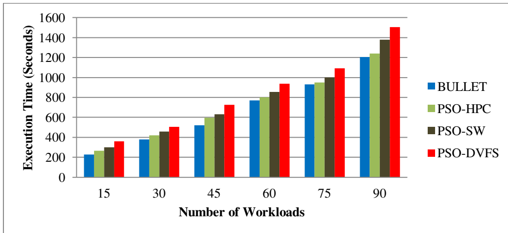
Figure 9: Effect of Execution Time with Change in Number of Workloads
