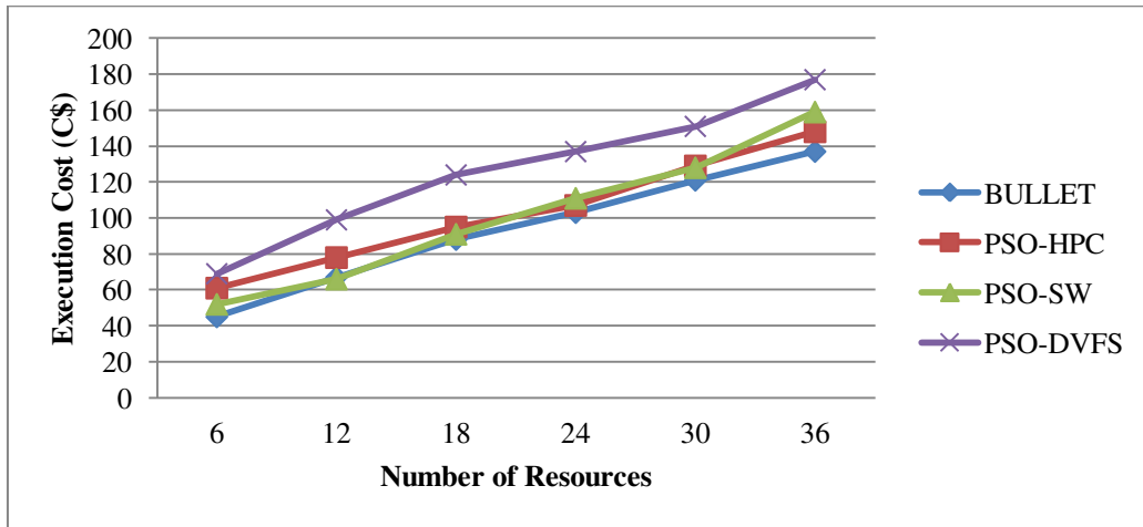
Figure 11: Effect of Execution Cost with Change in Number of Resources
