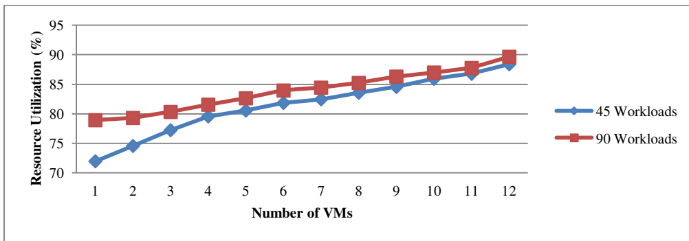
Figure 20: Effect of Change in Number of VMs on Resource Utilization
