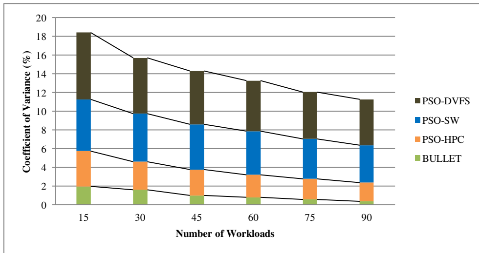
Figure 26: c_v for Execution Cost with Each Scheduling Algorithm
