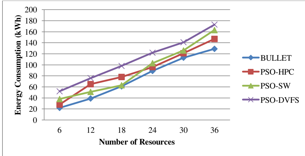
Figure 10: Effect of Change in Number of Resources Submitted on Energy Consumption
