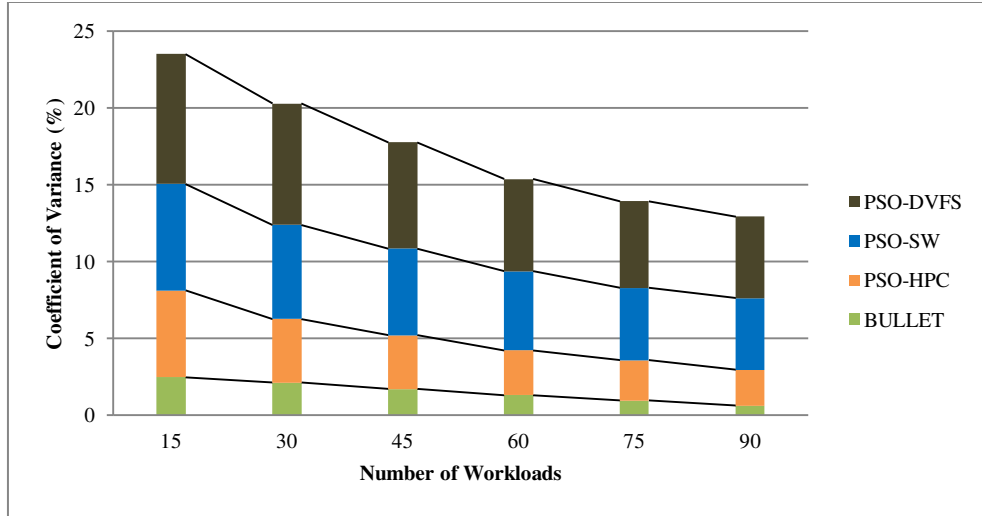
Figure 27: c_v for Energy Consumption with Each Scheduling Algorithm
