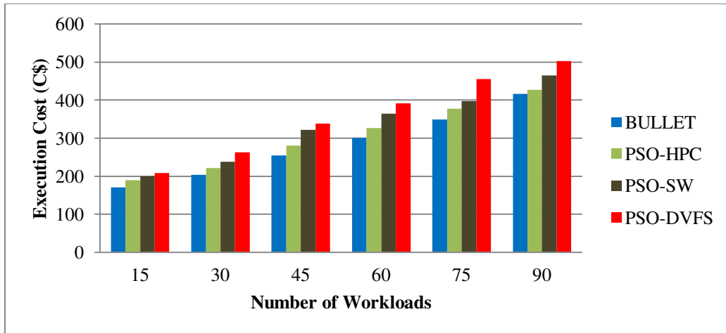
Figure 8: Effect of Execution Cost with Change in Number of Workloads
