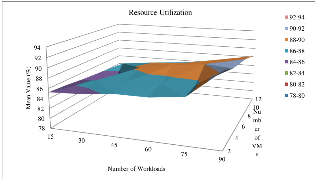
Figure 32: Statistical Analysis of Resource Utilization
