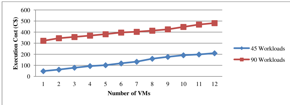
Figure 22: Effect of Change in Number of VMs on Execution Cost
