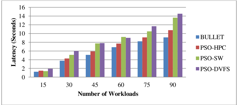
Figure 16: Effect of Change in Number of Workloads Submitted on Latency
