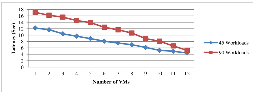
Figure 23: Effect of Change in Number of VMs on Latency
