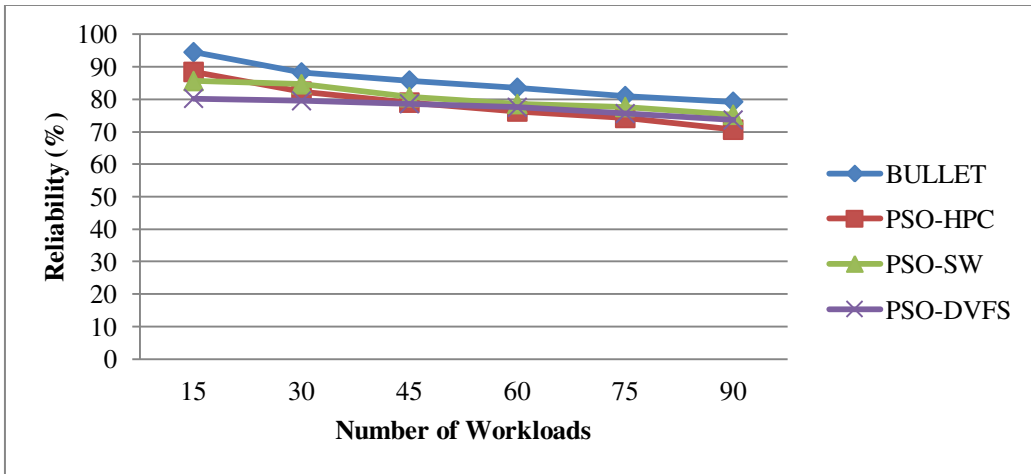
Figure 14: Effect of Change in Number of Workloads Submitted on Reliability
