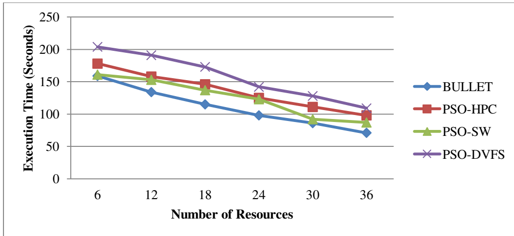
Figure 12: Effect of Execution Time with Change in Number of Resources
