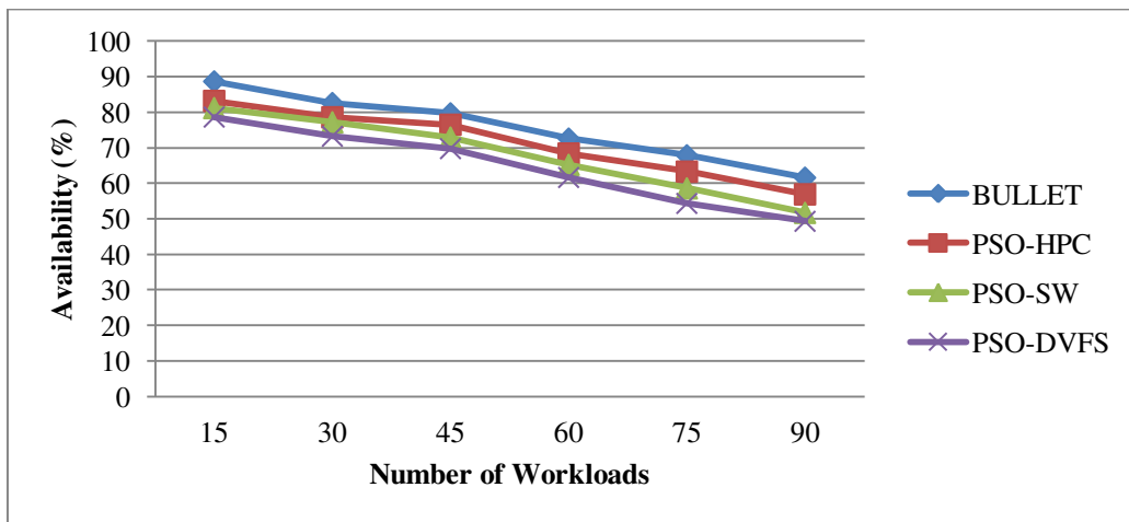
Figure 13: Effect of Change in Number of Workloads Submitted on Availability
