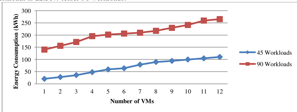
Figure 24: Effect of Change in Number of VMs on Energy Consumption
