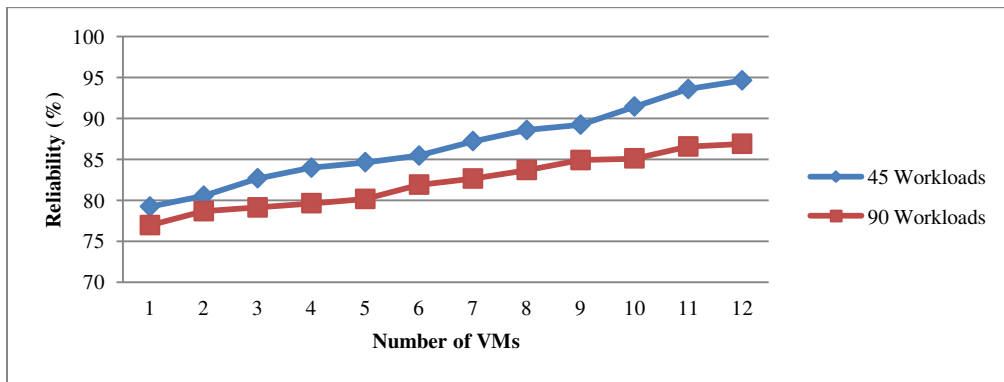
Figure 18: Effect of Change in Number of VMs on Reliability
