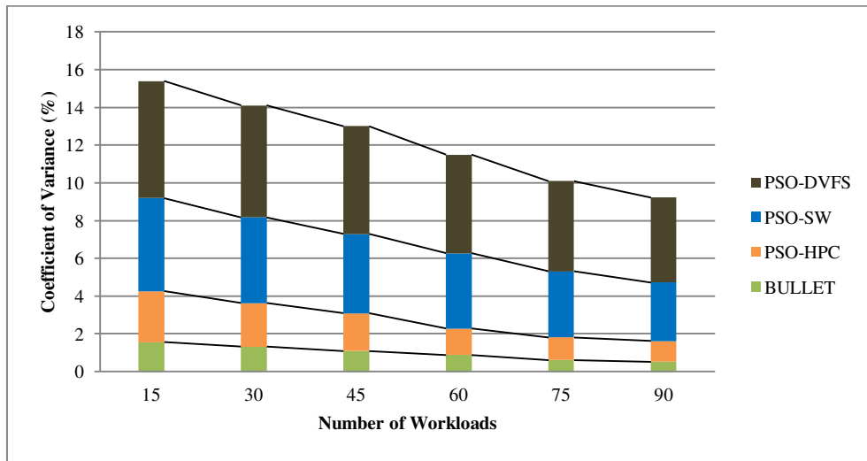
Figure 25: c_v for Execution Time with each scheduling Algorithm
