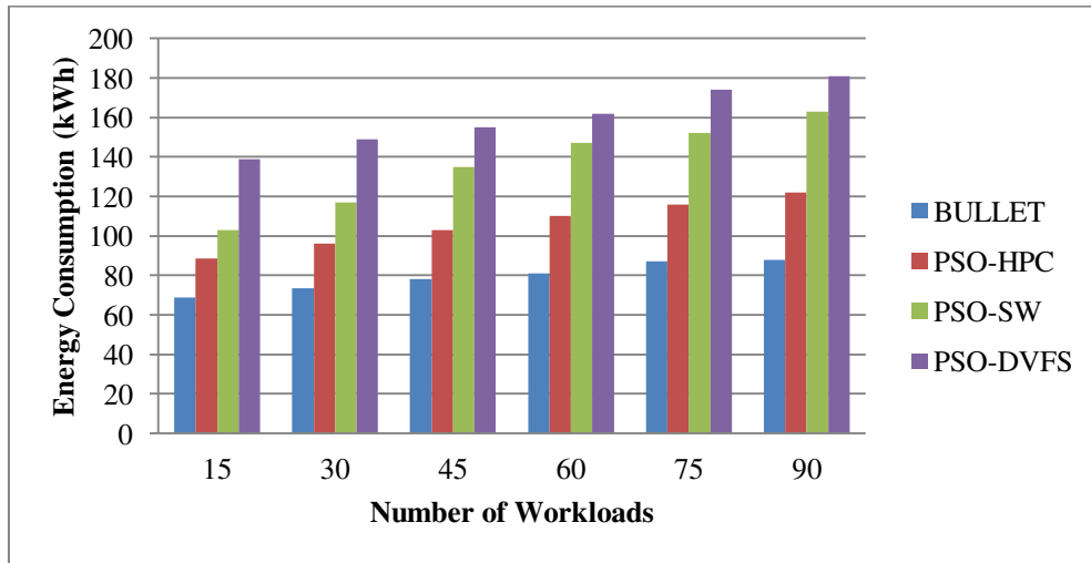
Figure 7: Effect of Change in Number of Workloads Submitted on Energy Consumption
