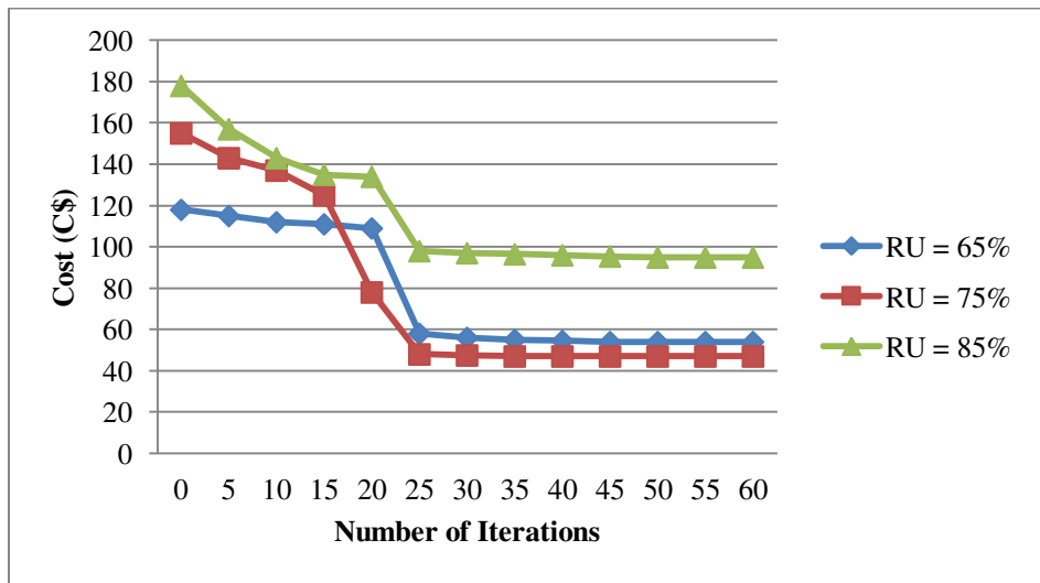
Figure 17: Convergence Curve of Total Cost
