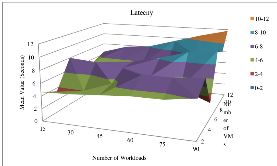
Figure 29: Statistical Analysis of Latency
