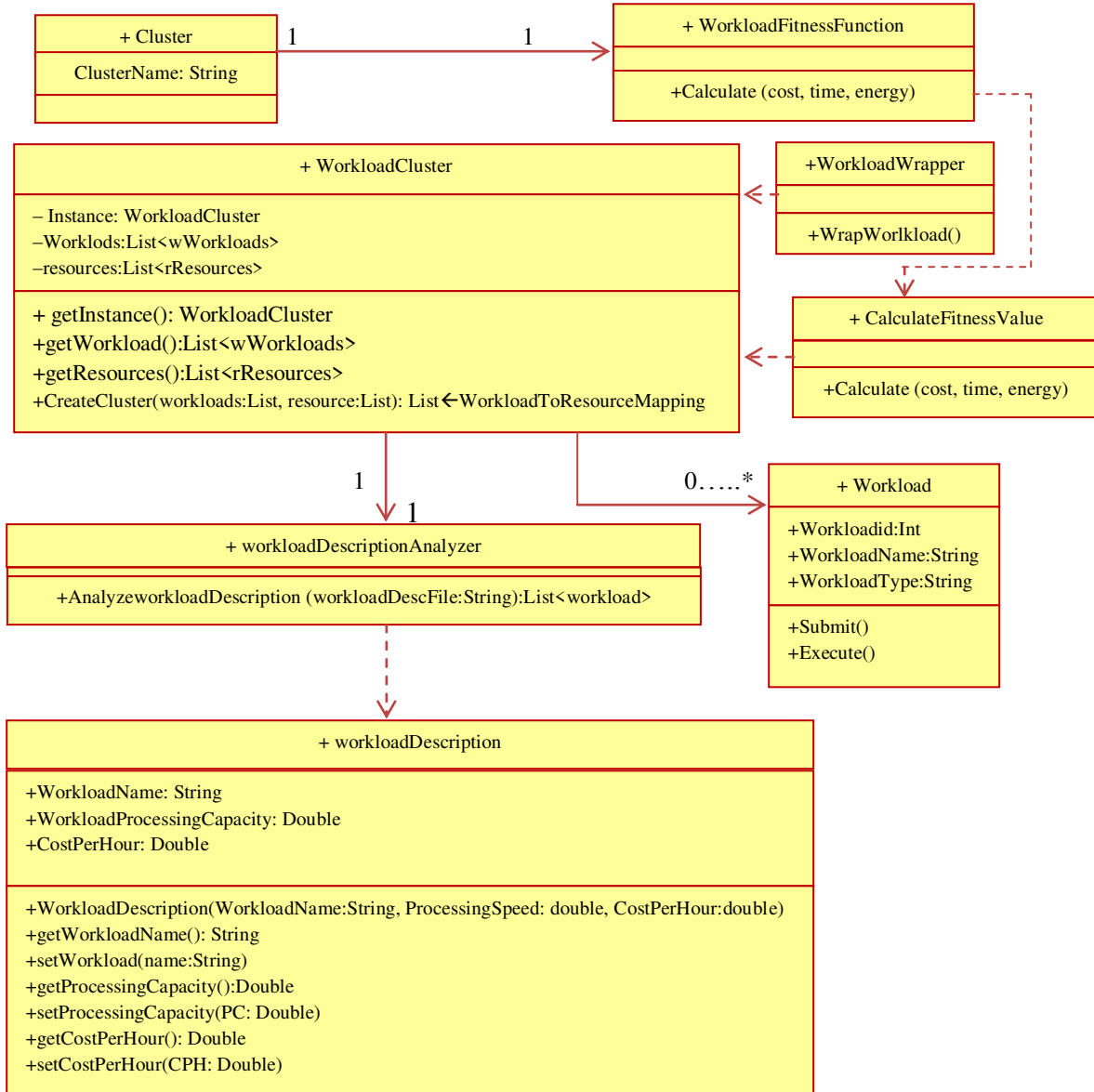
Figure 3: Interaction Among Different Classes For Workload Execution
