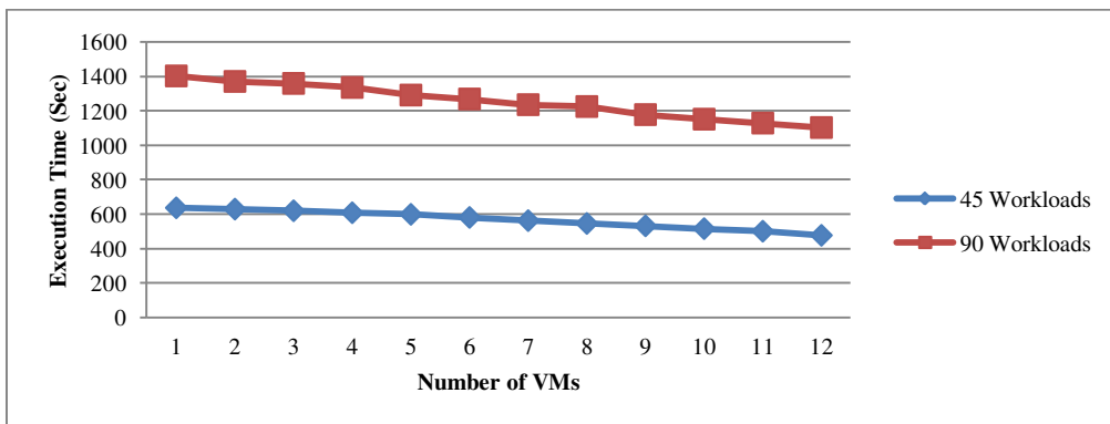
Figure 21: Effect of Change in Number of VMs on Execution Time
