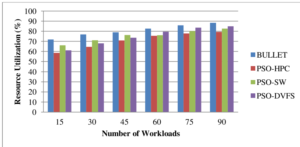
Figure 15: Effect of Change in Number of Workloads Submitted on Resource Utilization
