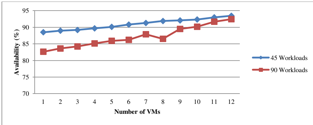
Figure 19: Effect of Change in Number of VMs on Availability
