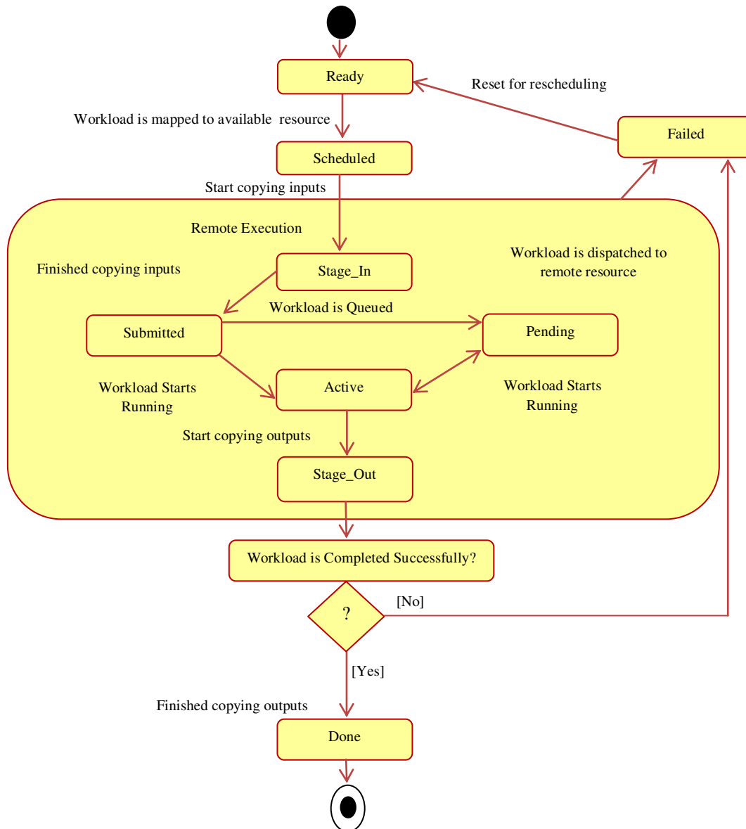
Figure 4: Different Stages For Cloud Workload
