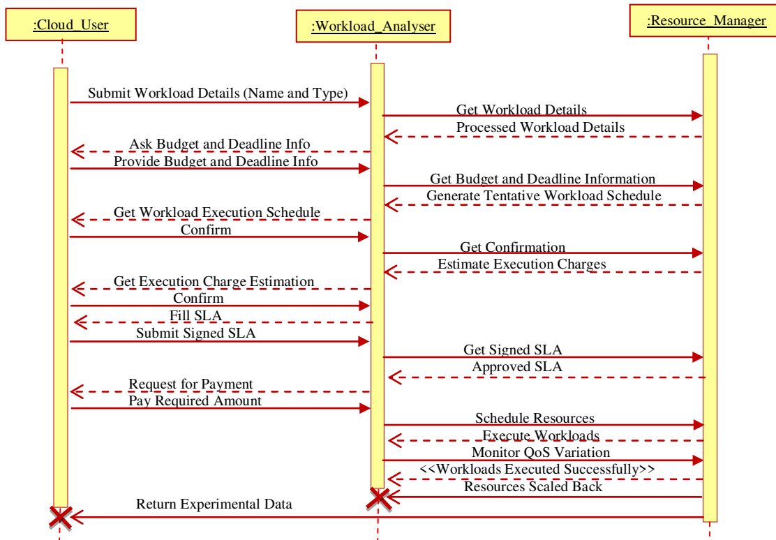
Figure 6: Workload Execution
