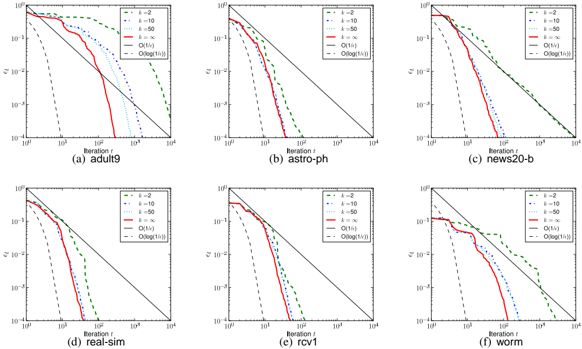
Figure 5: Approximation gap \epsilon_t as a function of number of iterations t ; for different bundle sizes k (and fixed regularization constant \lambda = 10^{-4} ).
