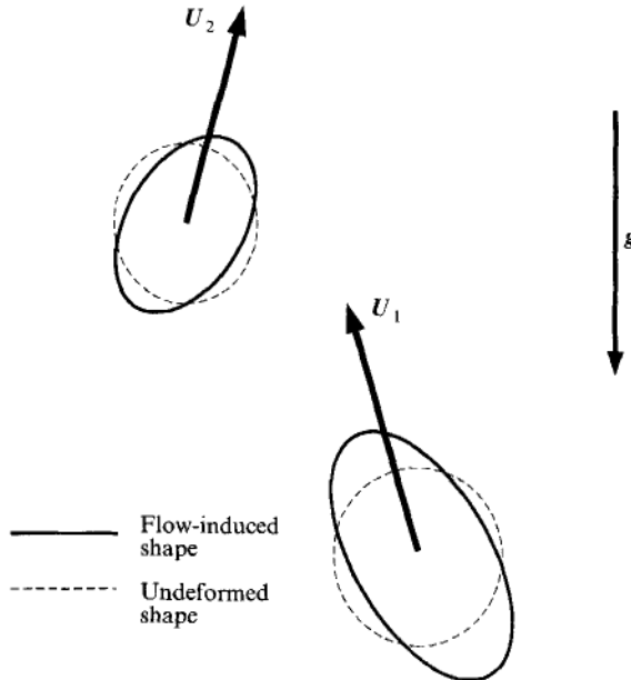
FIGURE 14. Illustration of the mechanism for the alignment of two rising deformable drops. The deformation of each drop by the flow produced by the other drop, as shown in figure 4, allows the drops to translate with velocities U_1 and U_2 which have horizontal components that favour alignment.
