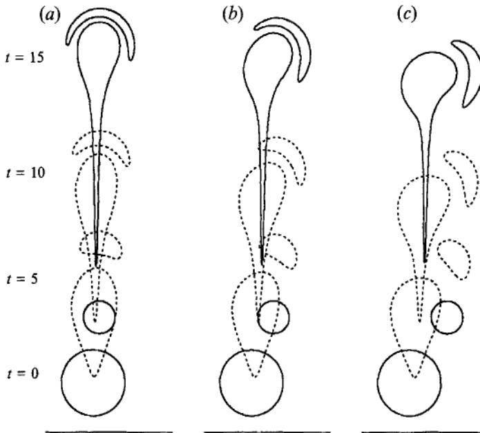
FIGURE 16. The effect of initial configuration. Results are shown for three different offsets; \lambda = 1 ; \mathcal{R} = \infty ; a_1/a_2 = 2 . The horizontal line represents a free-slip lower planar surface.
