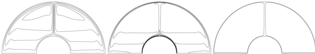
Figure 3. Streamline, isotherm and isoconcentration contours for \text{Al}_2\text{O}_3 + \text{H}_2\text{O} , \phi_{av} = 0.02 , D_i = 0.05 m, \delta = 3 , d_p = 25 nm, T_{av} = 315 K, and \Delta T = 10 K
