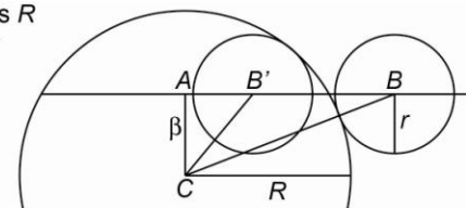
Figure 1: Eclipse geometry.
