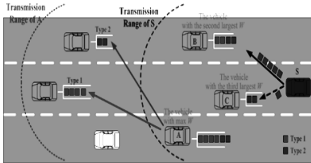
Fig. 3. DiffServ scenario in the FAB scheme.
