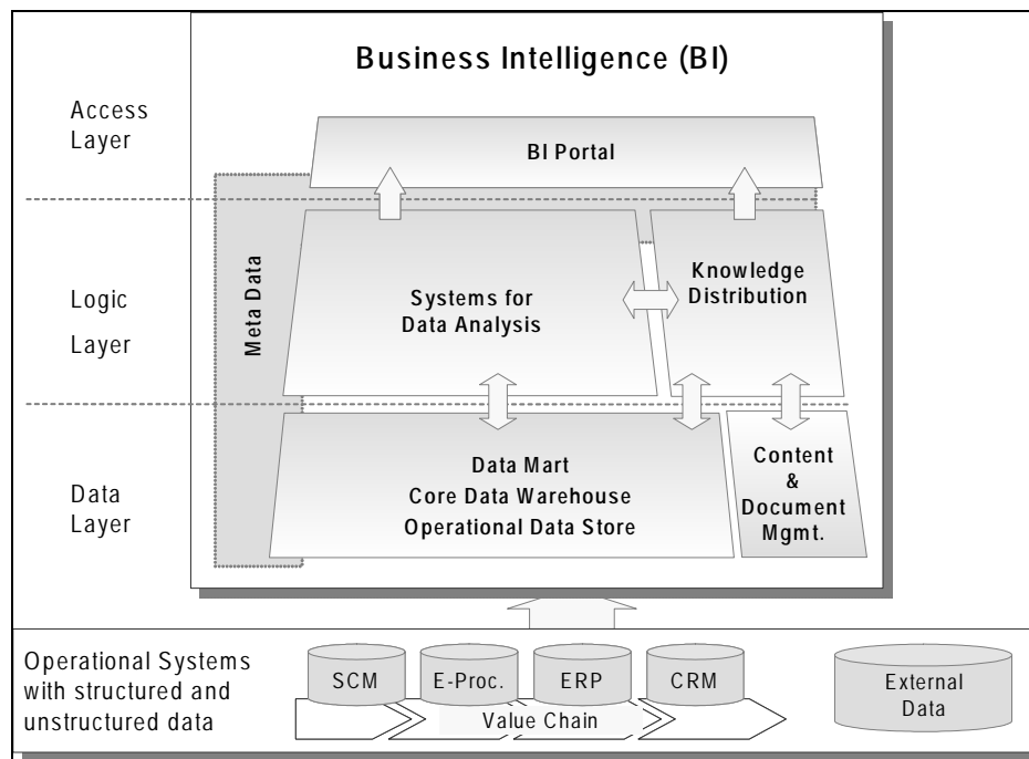
Figure 1 Conceptual three-layer BI architecture (Kemper and Baars 2006)
