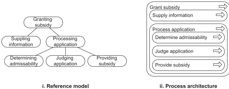
Figure 6. Example of function-based design of process architecture.
