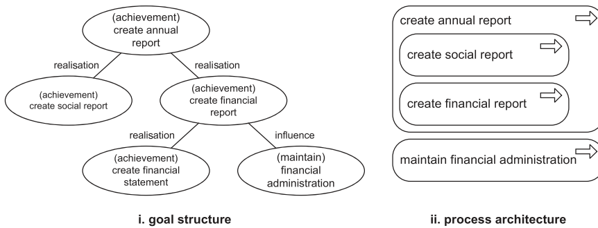
Figure 2. Example of goal-based design of process architecture.
