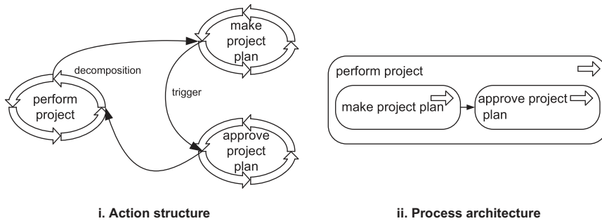
Figure 3. Example of action-based design of process architecture.
