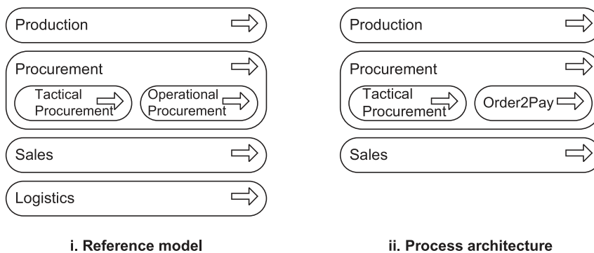
Figure 5. Example of reference model-based design of process architecture.
