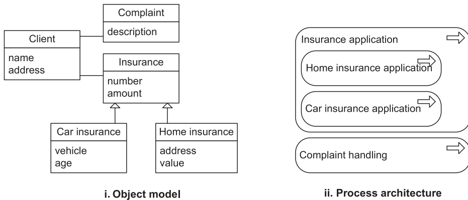
Figure 4. Example of object-based design of process architecture.
