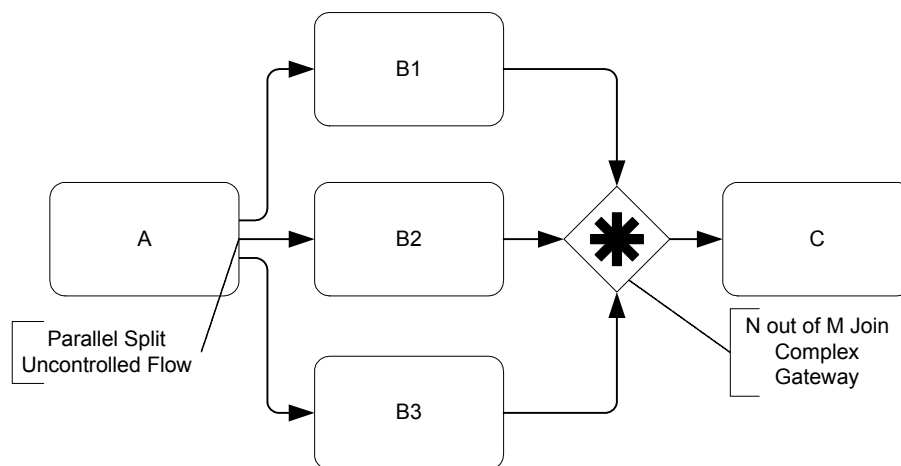
Figure 78 Workflow Pattern #8 -- N out of M Join
