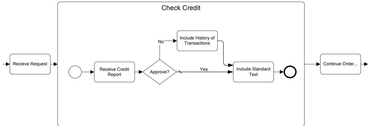
Figure 90 Example of Sub-Process with Start and End Events Inside
