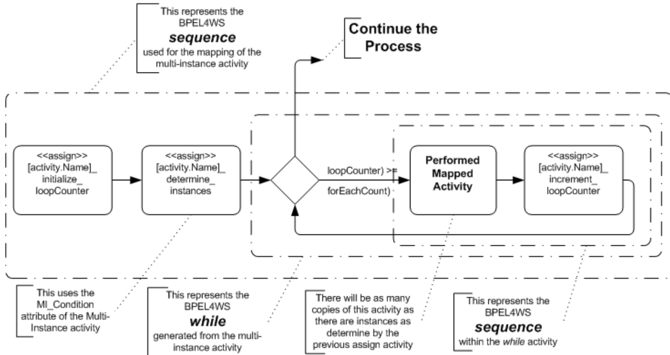
Figure 104 BPMN Depiction of BPEL4WS Pattern for a Sequential Multi-Instance loop
