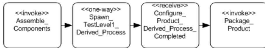
Figure 127 Example of the BPEL4WS Pattern for Substituting for the Derived Process
