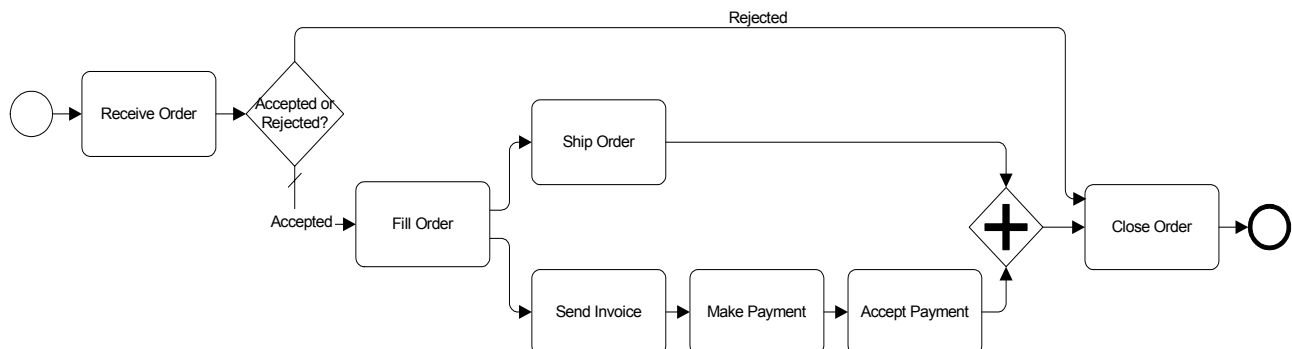
Figure 56 A Process with Normal Flow
