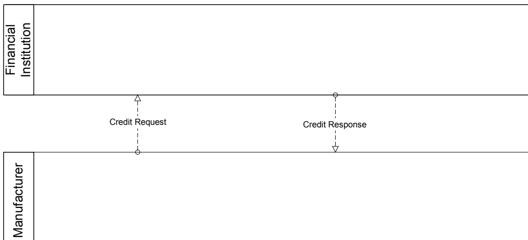
Figure 34 Message Flow connecting to the boundaries of two Pools
