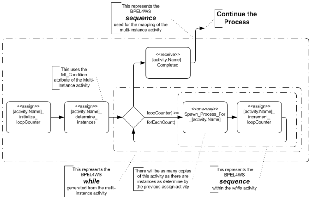
Figure 107 BPEL4WS Pattern of Parallel Multi-instance, MI_FlowCondition = One
