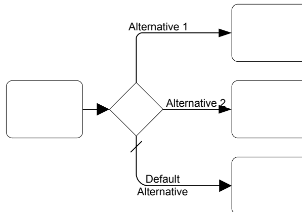
Figure 19 An Exclusive Data-Based Decision (Gateway) Example without the Internal Indicator
