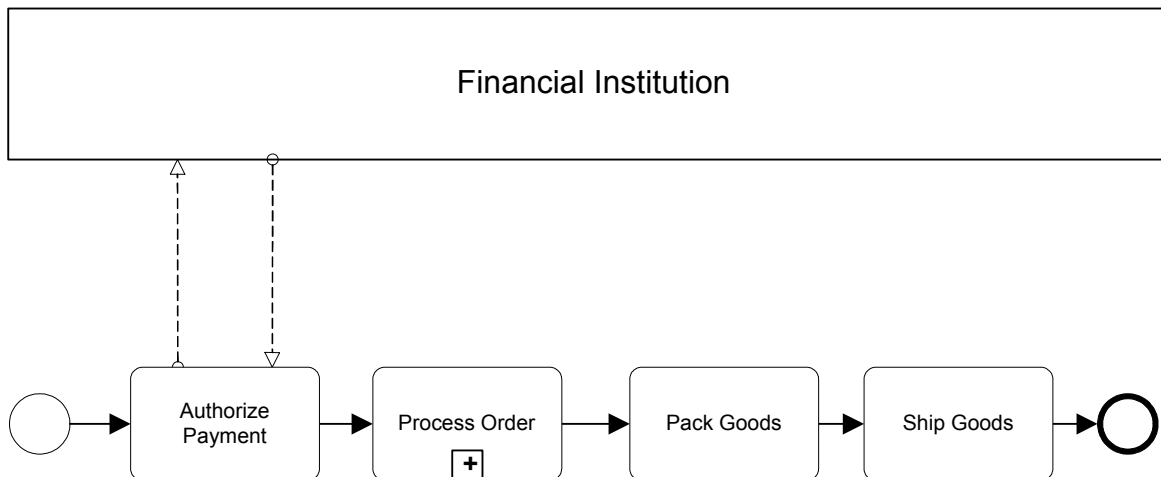
Figure 36 Main (Internal) Pool without boundaries
