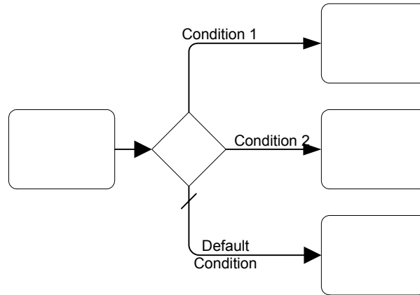
Figure 68 A Data-Based Decision Example -- Workflow Pattern #4 -- Exclusive Choice
