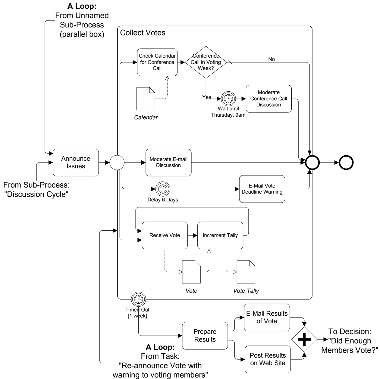
Figure 136 “Collect Votes” Sub-Process Details
