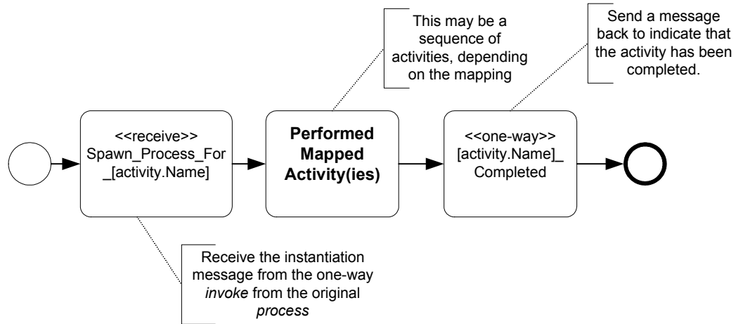
Figure 105 Structure of Process to be Spawned for Parallel Multi-instance
