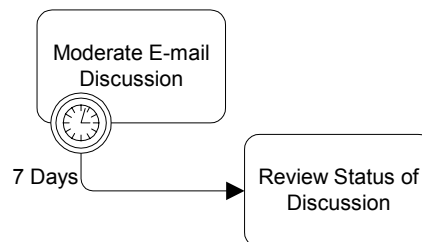
Figure 96 A Task with Exception Flow (Interrupts Event Context)
