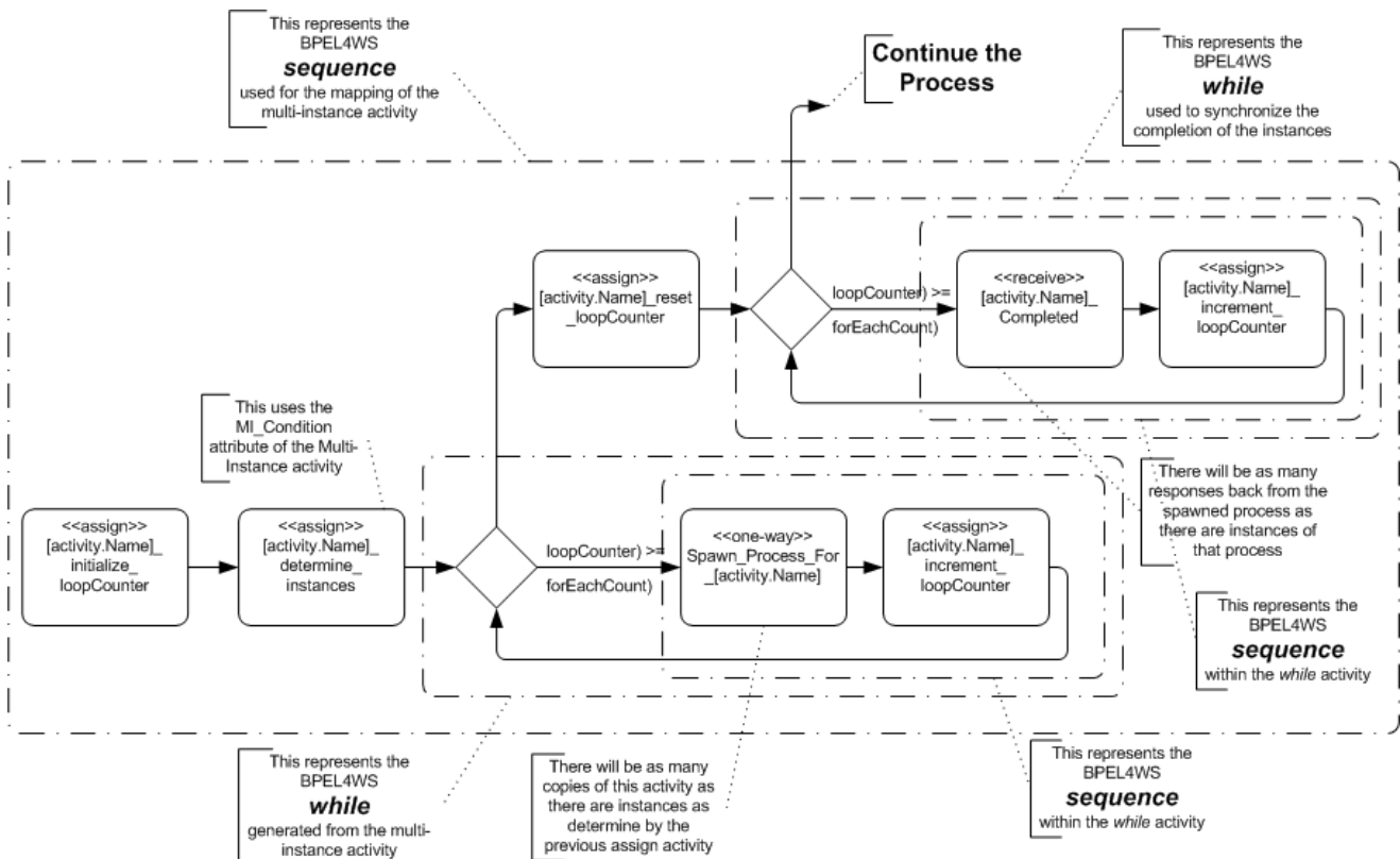
Figure 106 BPEL4WS Pattern of Parallel Multi-instance, MI_FlowCondition = All
