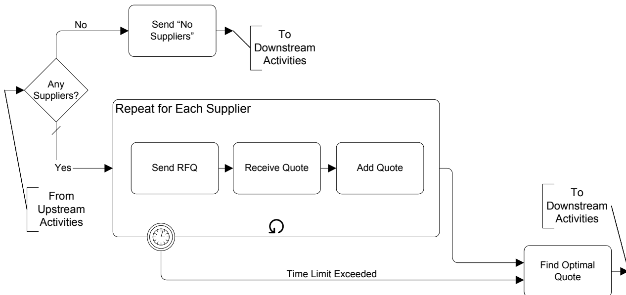
Figure 57 An Expanded Sub-Process without a Start Event and End Event
