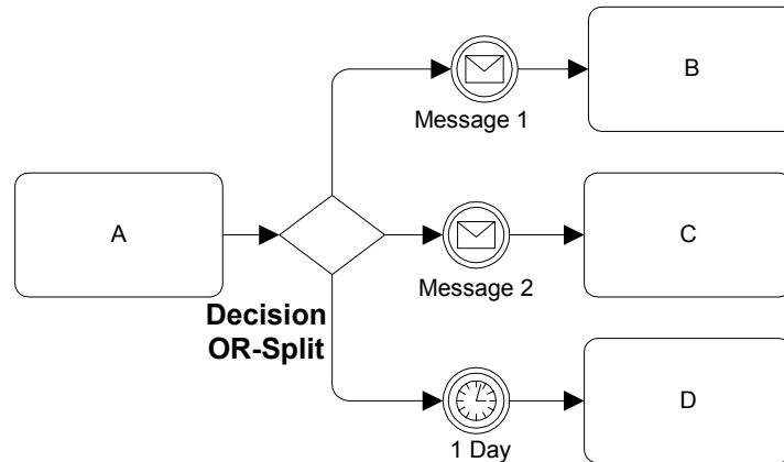
Figure 72 An Event-Based Decision Example
