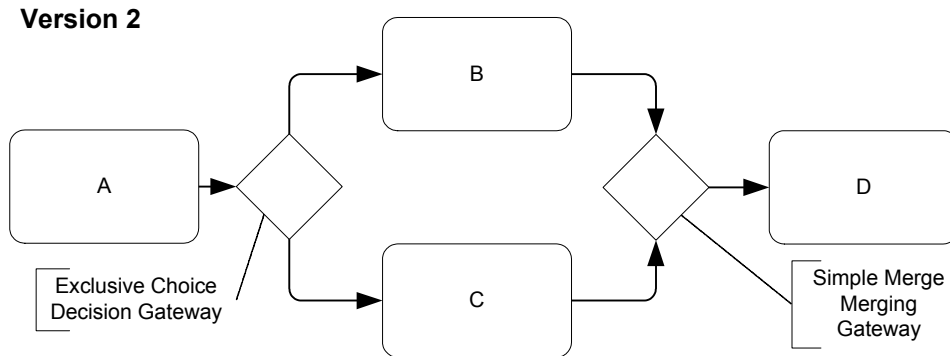
Figure 75 Workflow Pattern #5 -- Simple Merge – Version 2
