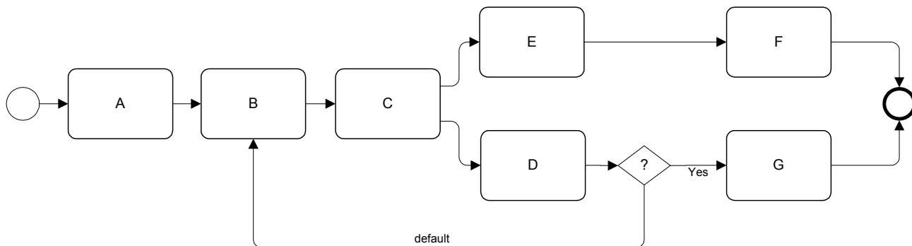
Figure 94 Improper Looping
