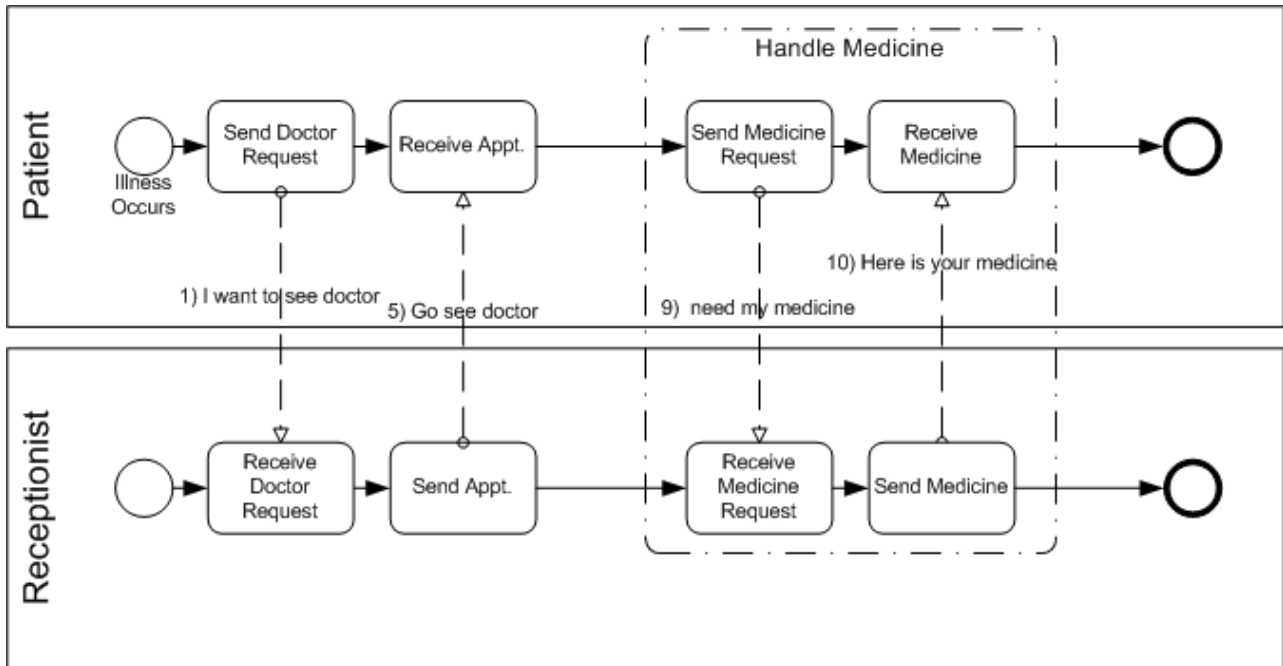
Figure 43 A Group around activities in different Pools
