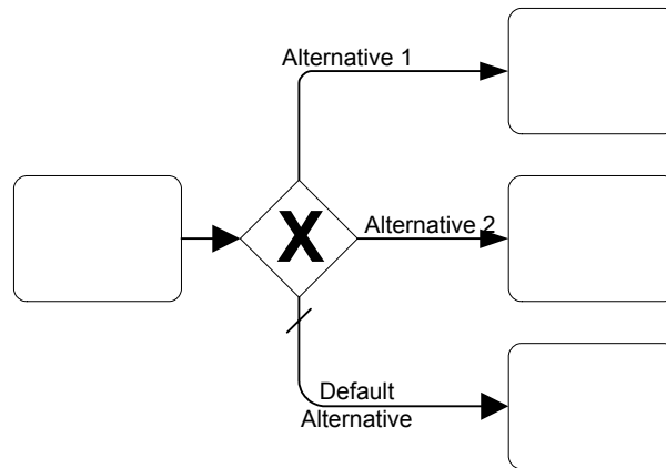
Figure 20 A Data-Based Exclusive Decision (Gateway) Example with the Internal Indicator
