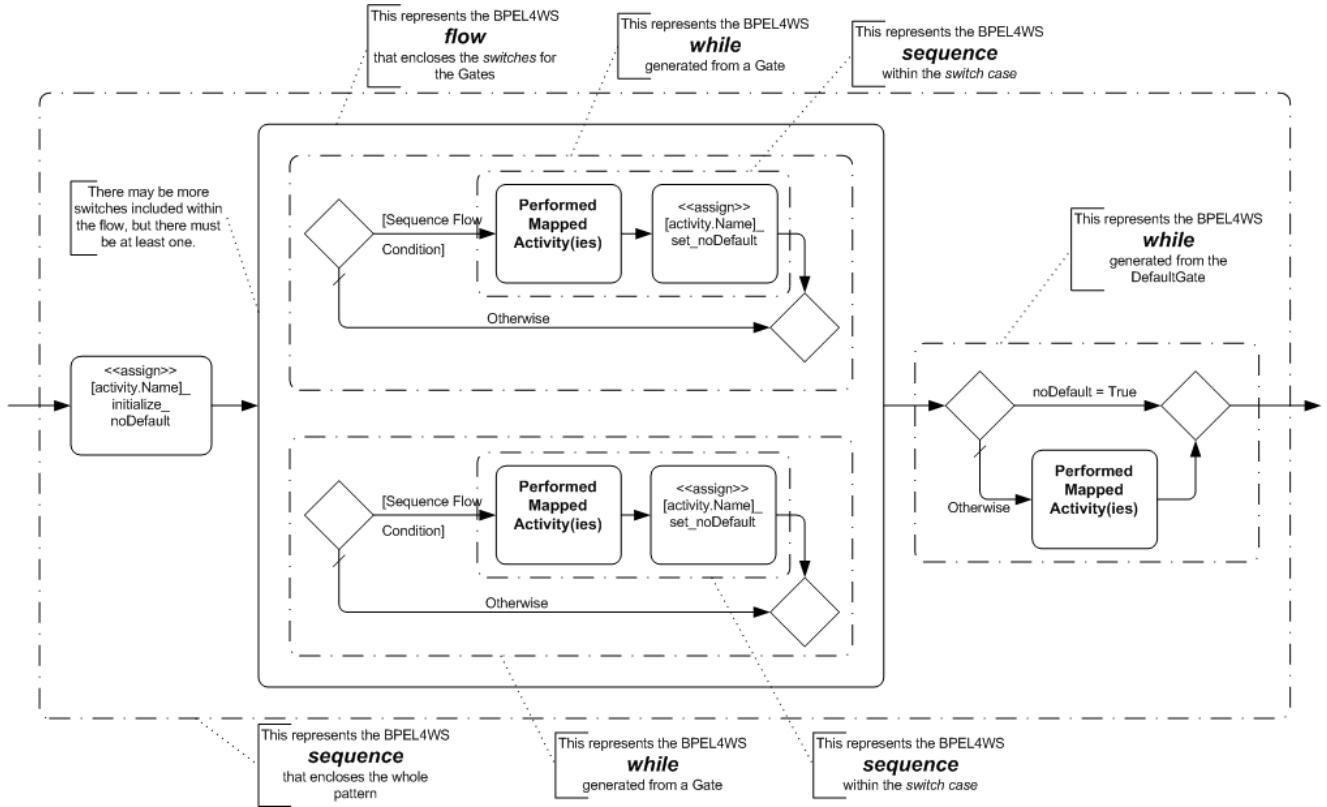
Figure 109 BPEL4WS Pattern of Inclusive Decision with two (2) Gates and a DefaultGate
