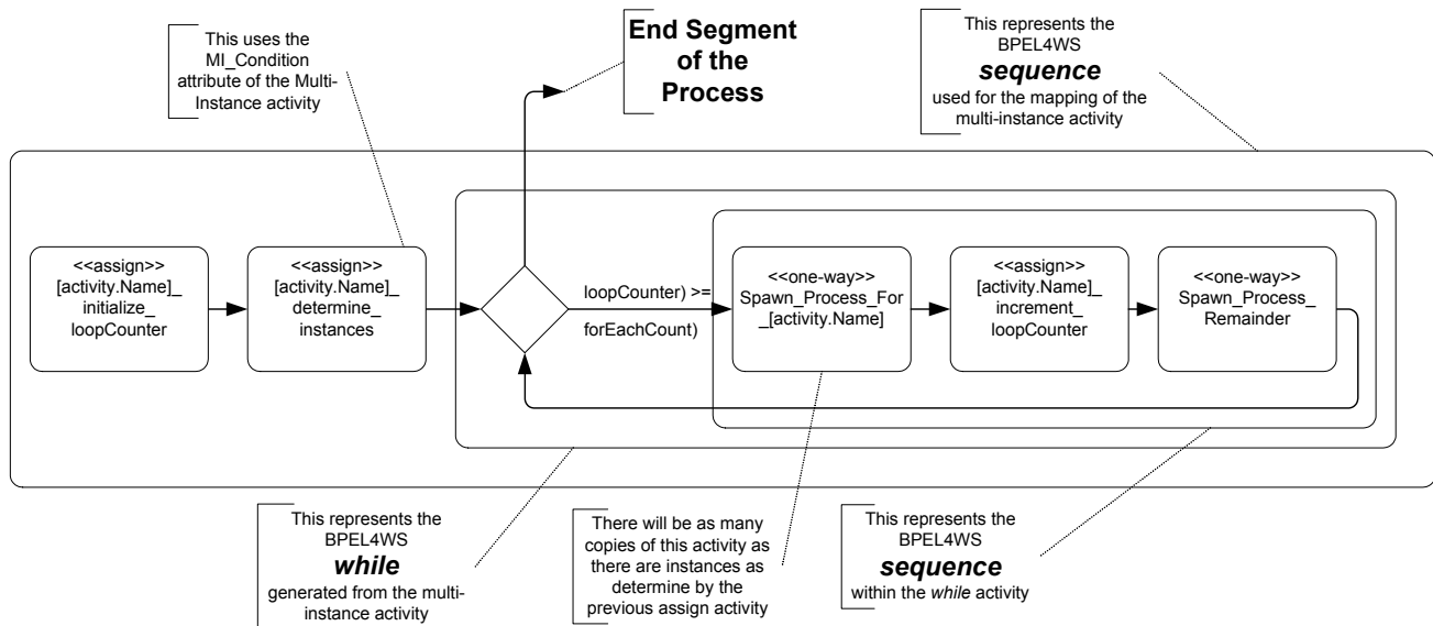
Figure 108 BPEL4WS Pattern of Parallel Multi-instance, MI_FlowCondition = None
