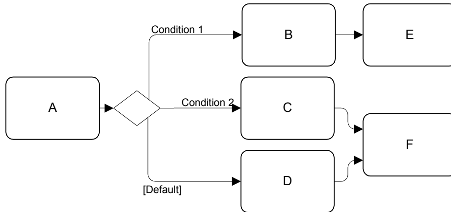
Figure 79 The Split-Merge Relationship is not Fixed
