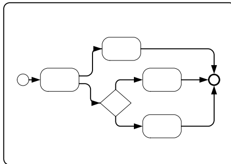
Figure 9 Expanded Sub-Process
