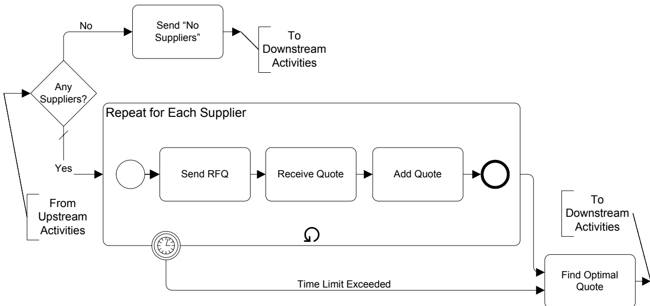
Figure 58 An Expanded Sub-Process with a Start Event and End Event Internal
