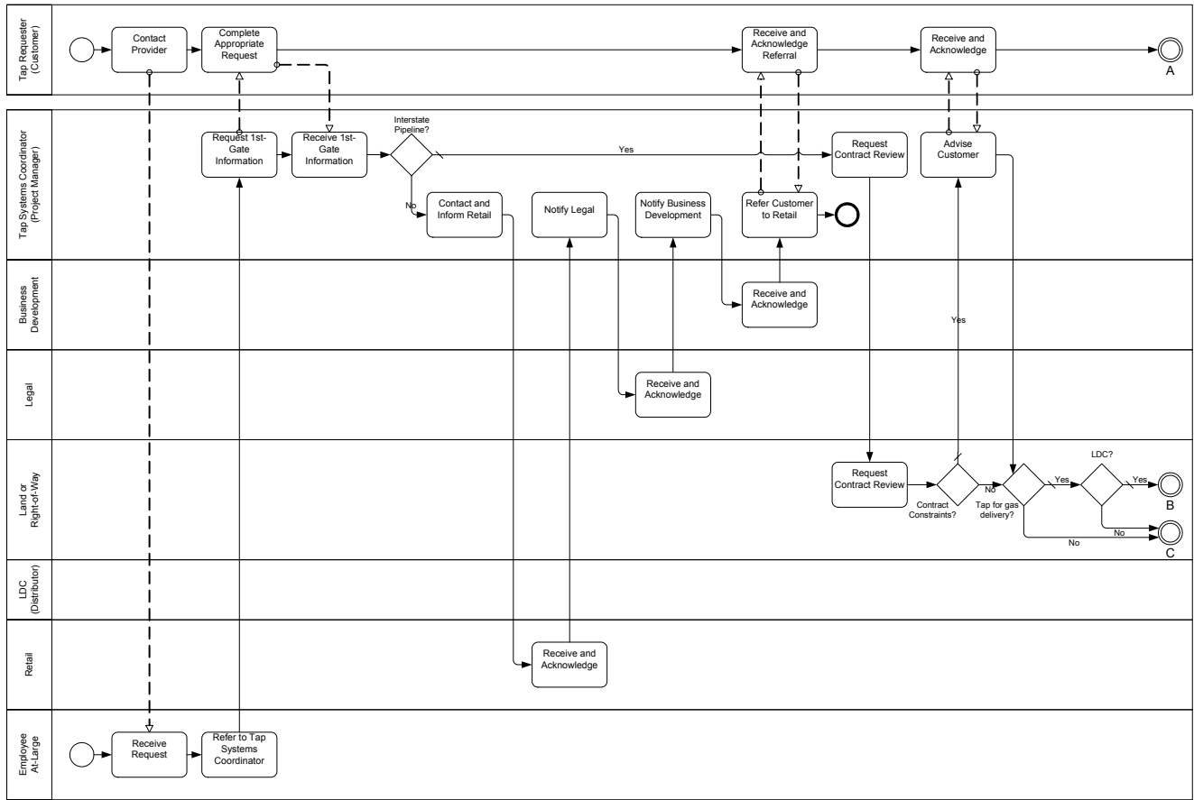
Figure 13 A Process and Diagram Details of the Sub-Process Object in the Previous Figure
