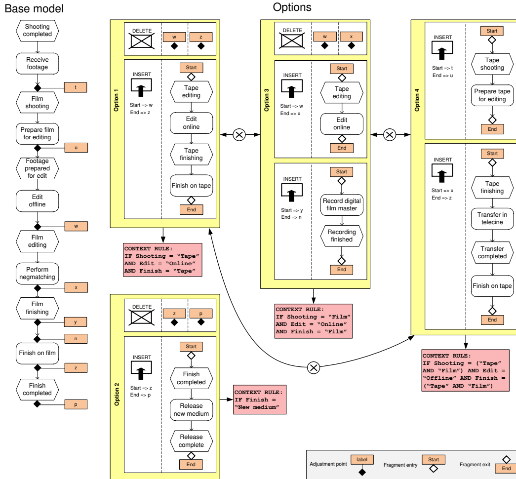
Fig. 13: The application of Provop to the process family of Figure 4.
