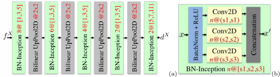
Fig. 3. Inception-based mask Deconvolution module. (a) Mask deconvolution network and (b) parametric BN-inception module, where s1 , s2 and s3 indicates the kernel sizes used in three Conv2D layers, respectively, and n stands for the number of filters.
