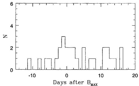
FIG. 4. Histogram showing the time with respect to B_{MAX} of the first photometric observation in B , V , or I . Note that for nearly one third of the SNe the photometric monitoring started before or at maximum light.
