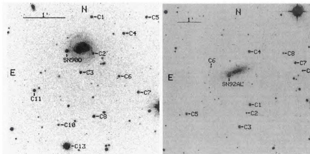
FIG. 2. V band CCD images of the two SNe Ia, 19900 and 1992al, discovered at other observatories and included in the Calán/Tololo follow-up photometric program. The photometric sequence stars are labeled along with the SNe.
