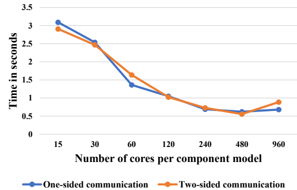
Figure 9. Comparison of data transfer times (for 100 ping-pong couplings) between a one-sided and a two-sided implementation, with the same configuration as Fig. 8.
