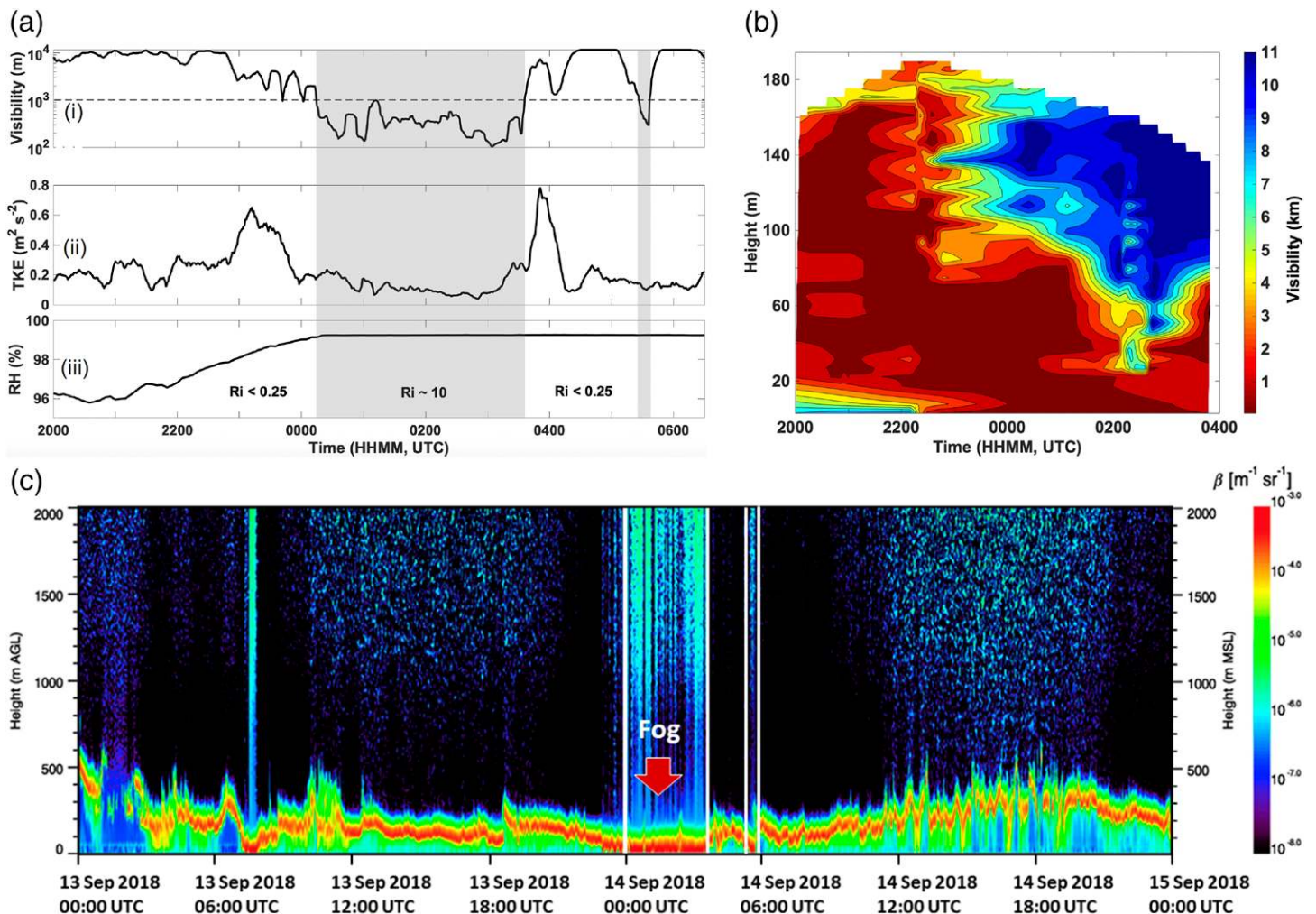
Fig. 10. (a) Time series of near-surface (i) 5-min-averaged visibility by PWD, (ii) TKE, and (iii) RH at the Blackhead site from 2000 UTC 13 Sep to ~0630 UTC 14 Sep. (b) Contour plot of visibility with time (2000 UTC 13 Sep to 0400 UTC 14 Sep) from the surface to 200 m AGL, showing stratus lowering, development of fog near the surface, and penetration of clear air from above down near the surface. Visibility here was derived using the correlations between an optical particle counter suspended on the tethered balloon and a PWD. (c) Ceilometer backscatter for Blackhead.
