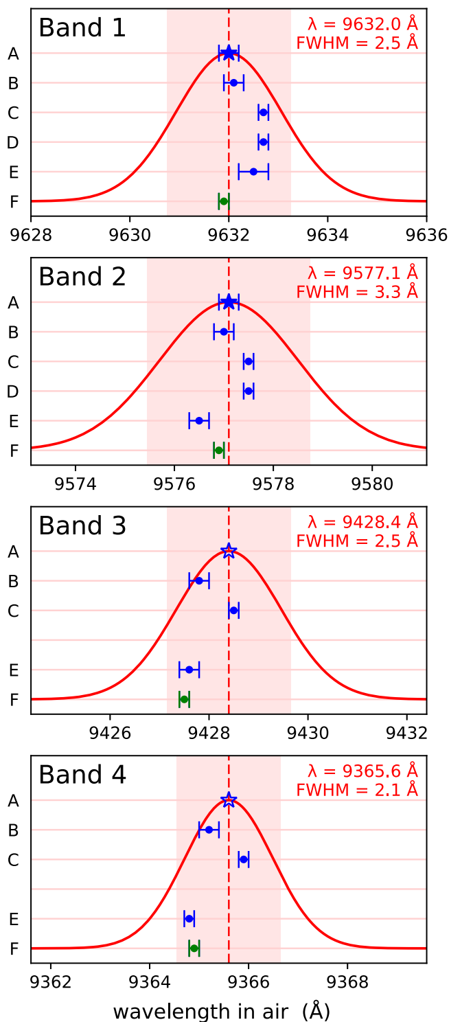
Figure 3. A comparison of the astronomical DIB data (A) with all reported laboratory data, obtained in the He-tagged ion trap experiments by Campbell et al. (2016a, 2016b, 2015; B, C, D), in the He droplet experiment by Kuhn et al. (2016b; E), and in the present work (F). The red curves are the (normalized) astronomical profiles and the red shaded zone shows the astronomical FWHM as reported in Cox et al. (2014) or Walker et al. (2016). All wavelengths are in air.
