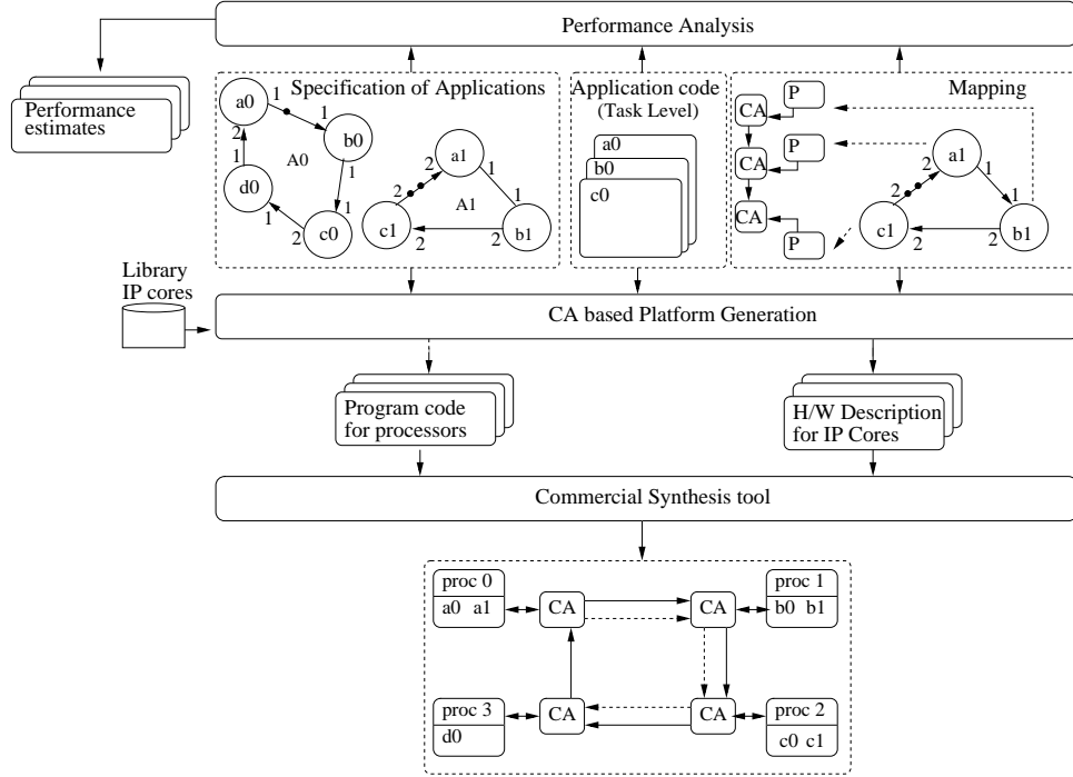
Figure 7: Design flow.
