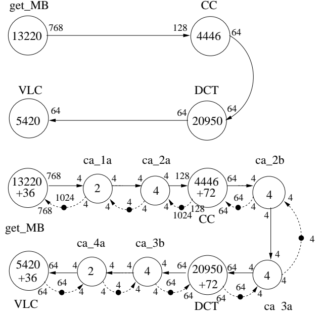
Figure 5: SDF graph of JPEG encoder and its transformation into CA-based platform.
