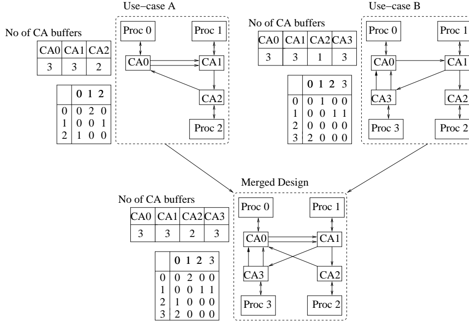
Figure 9: An example of showing how the combined hardware for different use-cases is generated. The corresponding communication matrix and no. of buffers are also shown for each hardware design.
