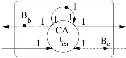
Figure 4: SDF model of CA.
