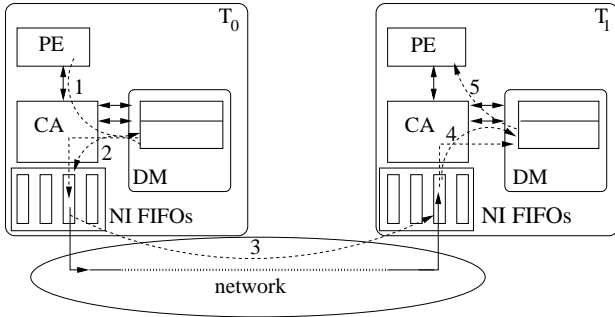
Figure 1: Proposed CA-based platform.
