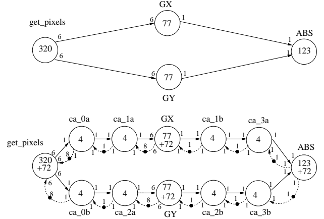
Figure 13: SDFG of Sobel and its transformation into CA-based platform.
