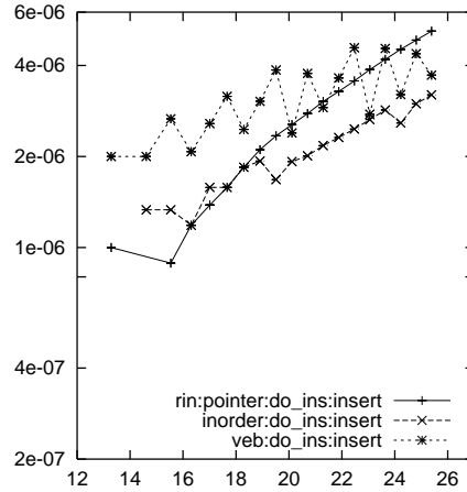
Figure 7: Insert time per element
