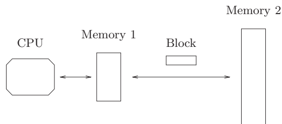
Figure 1: The I/O model
