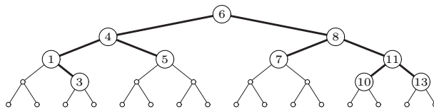
Figure 2: The embedding of a search tree with height 4 and size 10 in a complete tree with height 5
