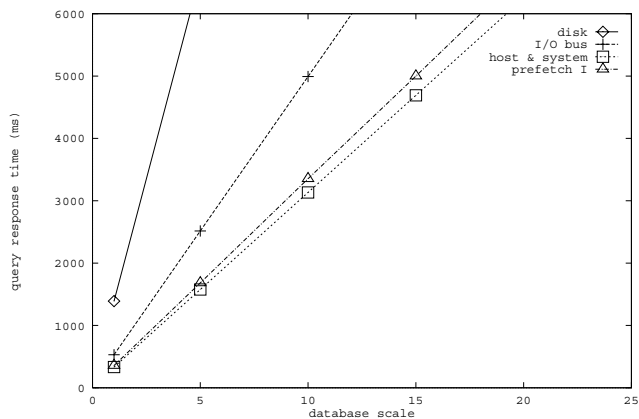
Figure 7: Scaling the database up to a 4 second response time for the best index organization.
