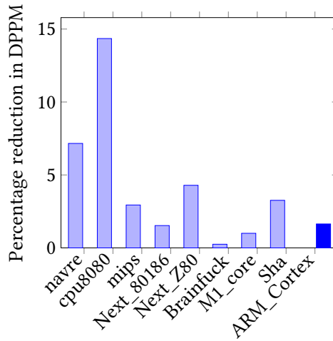
Fig. 14. Change in test escape rates expressed as DPPM when the original library is used instead of the fake one.
