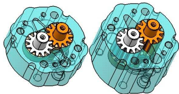
Fig. 5. The pump assembly for min/max flow values.
