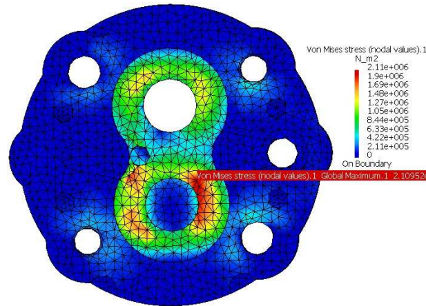
Fig. 10. Stresses distribution on the gearing teeth and on the pump body.
