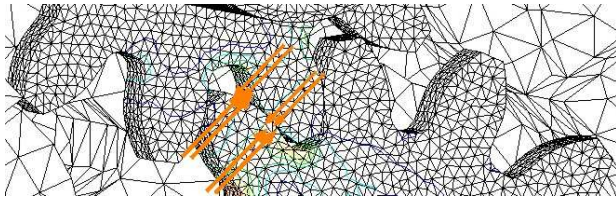
Fig. 9. Applying the tangential forces on the teeth in contact.
