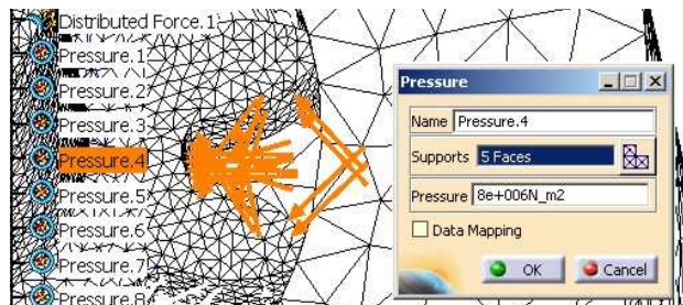
Fig. 8. Pressure distributed on teeth.
