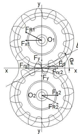
Fig. 7. Tangential and radial forces loaded on gearing and shafts.
