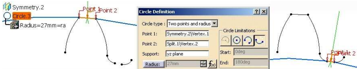
Fig. 1. Parametric coordinates of points and formulas to define the tooth profile.
