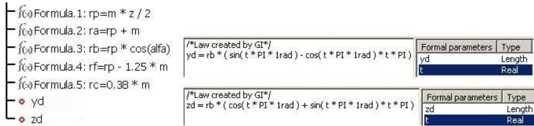
Fig. 1. Parametric coordinates of points and formulas to define the tooth profile.
