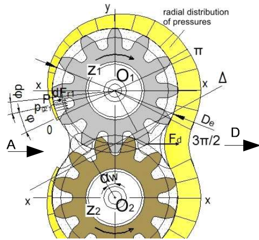
Fig. 6. Radial distribution of fluid pressures loaded on gearing.
