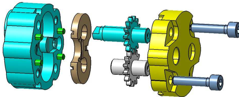
Fig. 3. The gear pump assembly in a 3D exploded view.
