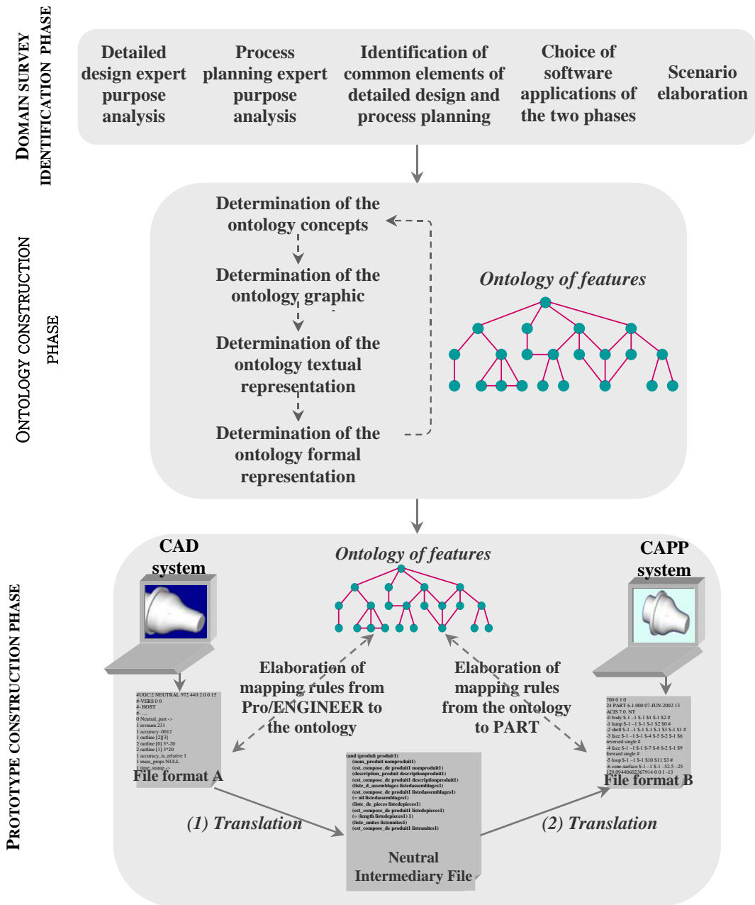
Figure 1: Global process for data exchange using ontologies
