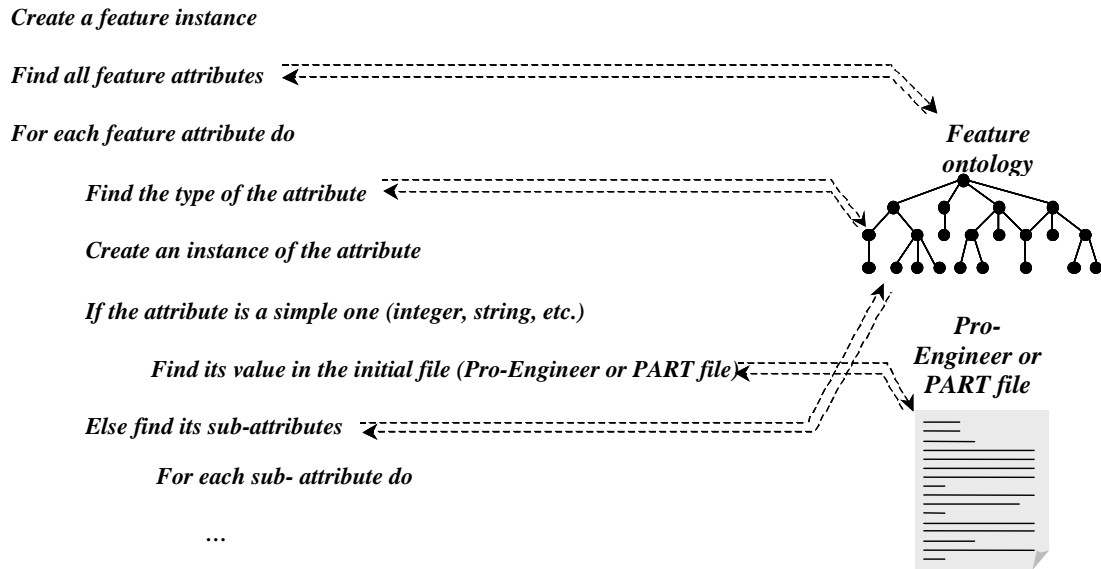
Figure 16: General algorithm for data exchange
