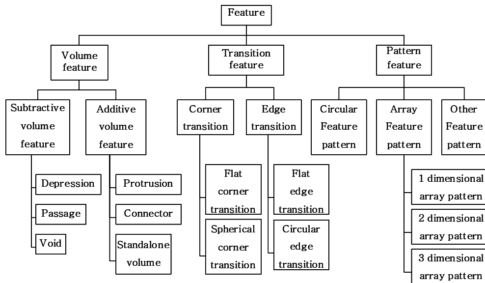
Figure 11: Feature decomposition
