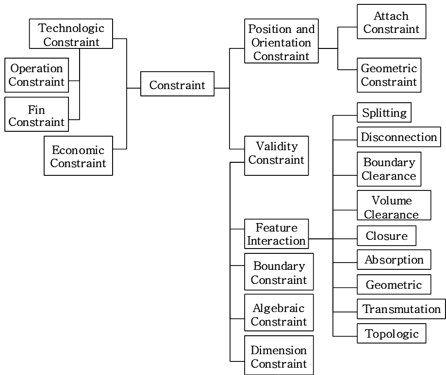
Figure 6: Constraint classification
