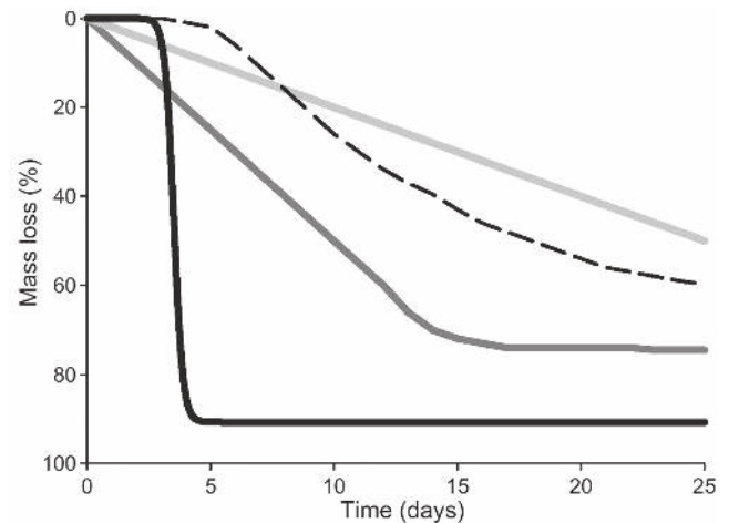
Figure 1. Mass loss curves typically associated with the decomposition of a cadaver on the soil surface (—), buried cadaver (- - -), plant material (—) or fecal (dung) material (—). Cadaver mass loss data was compiled from previous publications: cadaver on soil surface (Payne 1965); buried cadaver (Carter 2005); plant material (Wardle et al. 1994; Coleman et al. 2004); fecal matter (Putman 1983; Esse et al. 2001).
