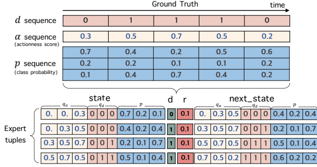
Figure 5. Expert database construction. Here, we assume that the number of classes is 3, as can be seen by a p sequence having 3 rows. From the given ground truth d , \alpha , and p sequences, we can extract four expert transitions, consisting of state, decision ( d ), reward ( r ), and next_state. Aggregating these tuples, we can construct an expert database.
