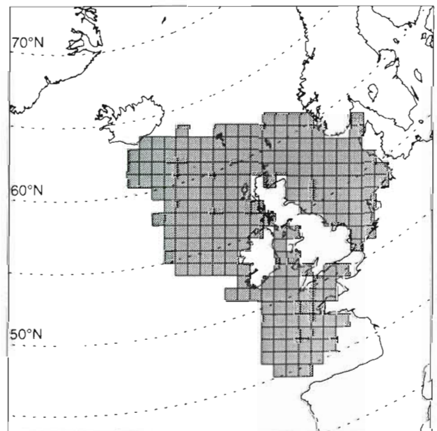
Fig. 1. Study area. Selection of this area was based on the regularity of the Continuous Plankton Recorder (CPR) sampling from 1962 to 1992
