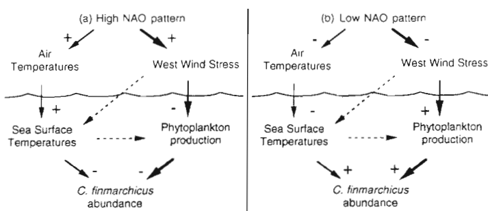
Fig. 7. General scheme of the connections between NAO and Calanus finmarchicus during (a) high and (b) low NAO patterns
