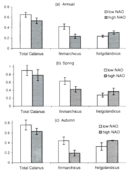
Fig. 6. (a) Mean annual log abundance of total Calanus species, C. finmarchicus and C. helgolandicus , during low (1963, 1964, 1966, 1969, 1977, 1979) and high (1983, 1989, 1990, 1991, 1992) NAO years, with confidence intervals at the 5% level. (b) Mean spring log abundance with confidence intervals. (c) Mean autumn log abundance with confidence intervals.
