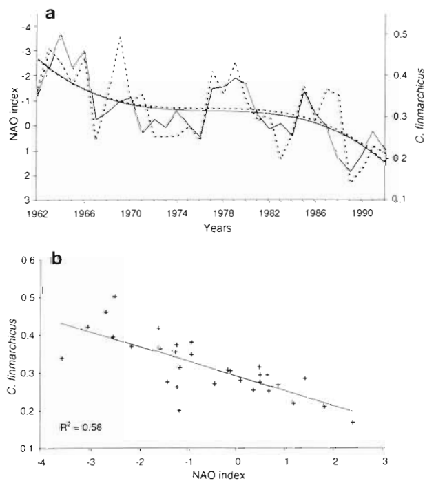
Fig. 4. (a) Average log abundance [ \log(x+1) ] of Calanus finmarchicus over the study area (solid line) and NAO index on a reverse scale (dashed line) from 1962 to 1992. Third-order polynomial fits are superimposed. (b) Linear regression plot between the NAO index and C. finmarchicus log abundance. Each annual value is based on ~2300 samples
