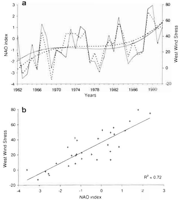
Fig. 3. (a) Average west wind stress (WWS) in m^2 s^{-2} over the study area (solid line) and NAO index (dashed line) from 1962 to 1992. Third-order polynomial fits are superimposed. (b) Linear regression plot between the NAO index and the WWS
