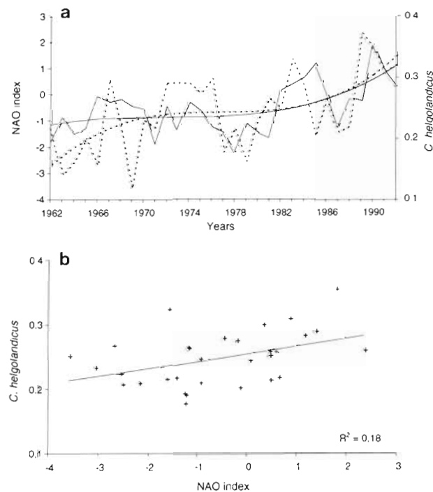
Fig. 5. (a) Average log abundance [ \log(x+1) ] of Calanus helgolandicus over the study area (solid line) and NAO index (dashed line) from 1962 to 1992. Third-order polynomial fits are superimposed. (b) Linear regression plot between the NAO index and C. helgolandicus log abundance. Each annual value is based on ~2300 samples
