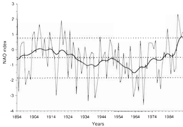
Fig. 2. North Atlantic Oscillation (NAO) December–April index based on the average pressure difference between the Azores and Iceland from 1895 to 1992. Dashed lines indicate the mean of the series (middle line) plus and minus standard deviation (upper and lower lines)
